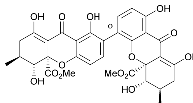
102 Penicillixanthone A (absolute stereochemistry)
