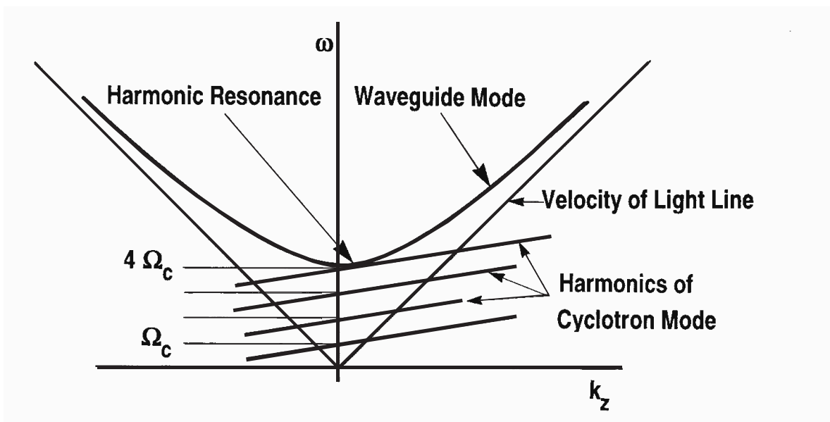
Fig. 4: Dispersion diagram of harmonic frequency gyrotron oscillator.
