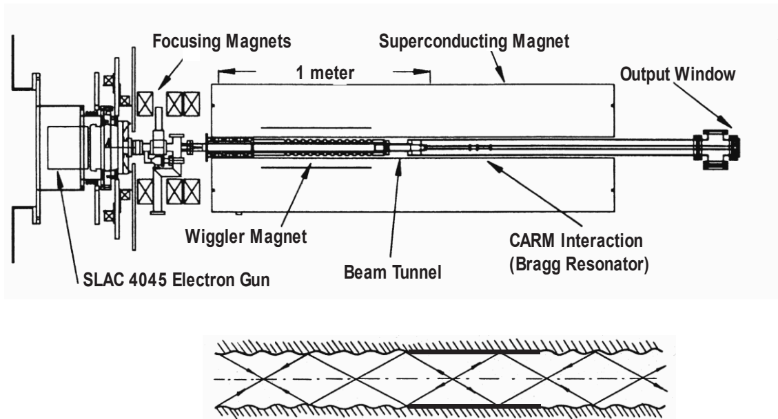
Fig. 7: Schematic of the long-pulse MIT CARM oscillator experiment [318] and scheme of a Bragg resonator [285].
