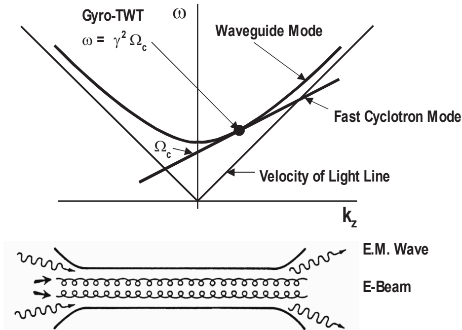
Fig. 8: Dispersion diagram and scheme of interaction circuit of Gyro-TWT amplifier.
