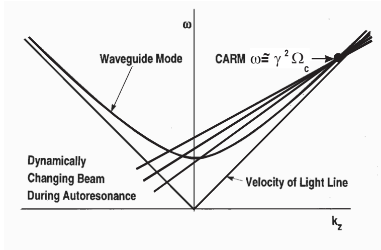
Fig. 6: Dispersion diagram of the cyclotron autoresonance maser (CARM).
