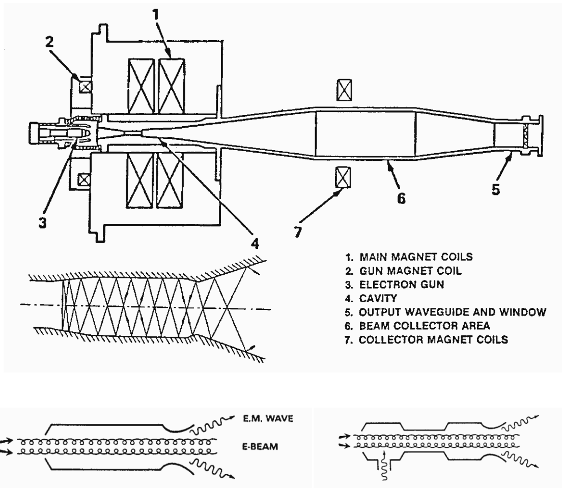
Fig. 1: Schematic of VARIAN CW gyrotron oscillator [14,19] and scheme of irregular waveguide cavities of gyromonotron oscillator (left) and two-cavity gyrokystron amplifier [302,303].
