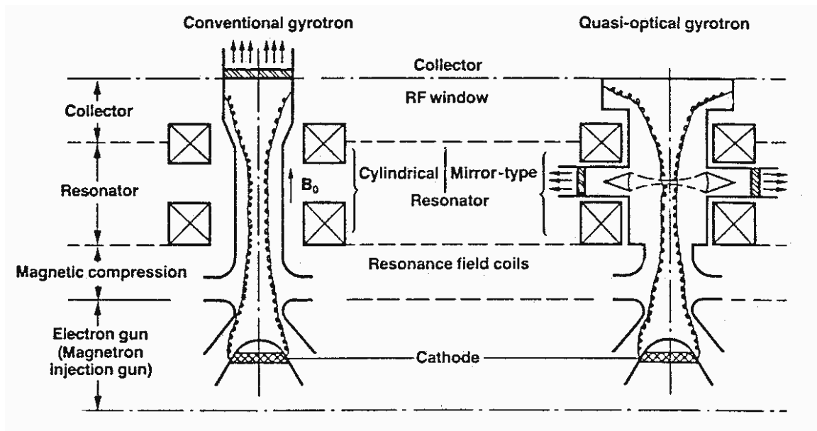
Fig. 2: Principle of a conventional gyrotron with cylindrical resonator and of a quasi-optical gyrotron with mirror resonator [84,85].
