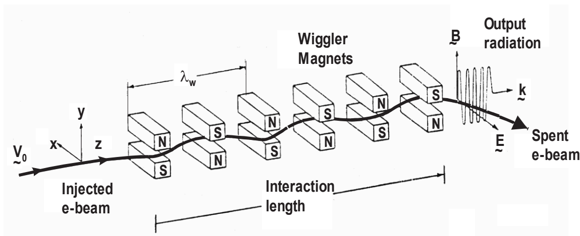
Fig. 11: The basic FEM configuration. Electrons in an injected electron beam undulate in the periodic magnetic field of the wiggler.
