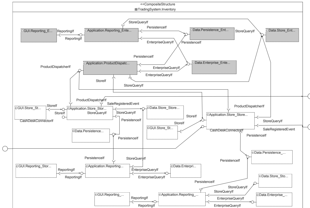
Figure 2.16.: Component Model of the CoCoME Architecture in PCM System View [158]
