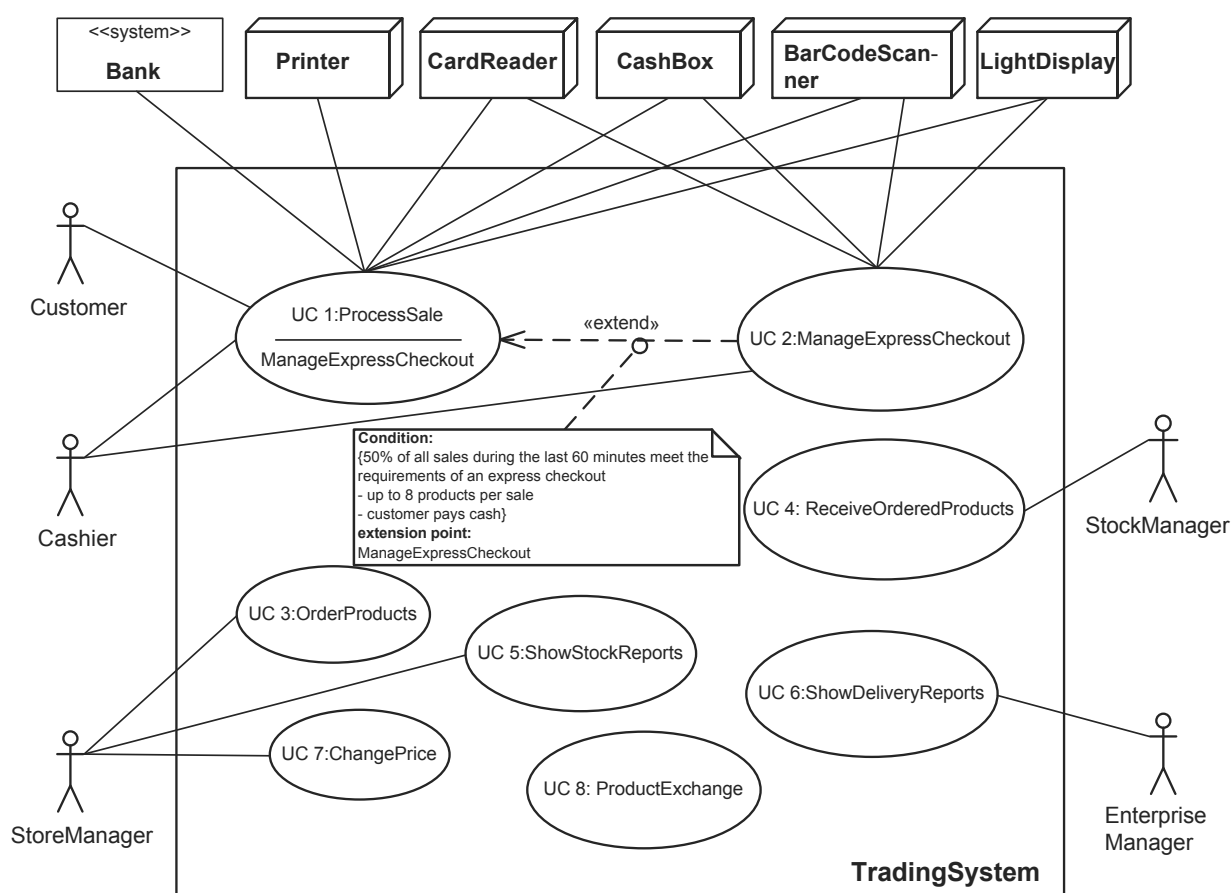
Figure 2.15.: An Overview of All Considered Use Cases of the CoCoME Trading System [155]
