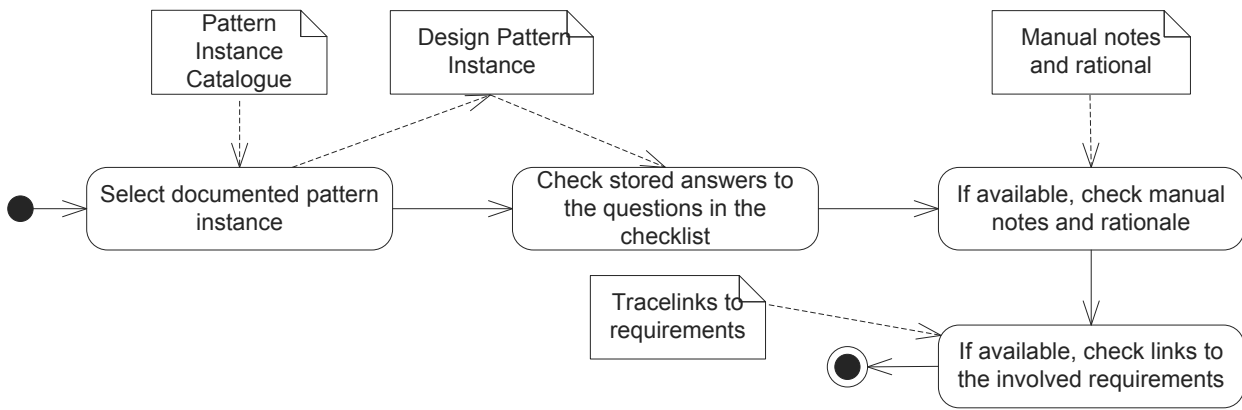
Figure 3.10.: Activity Diagram of Understanding Pattern Design Decision Use Case
