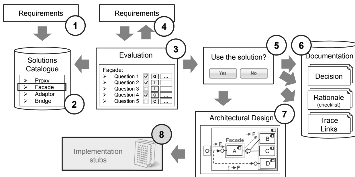
Figure 3.2.: Overview of the AM3D Approach (Adopted from [1])
