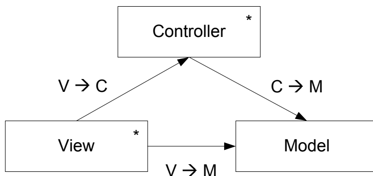
Figure 4.12.: An Example of Roles and Connectors Representation for the Model View Controller pattern
