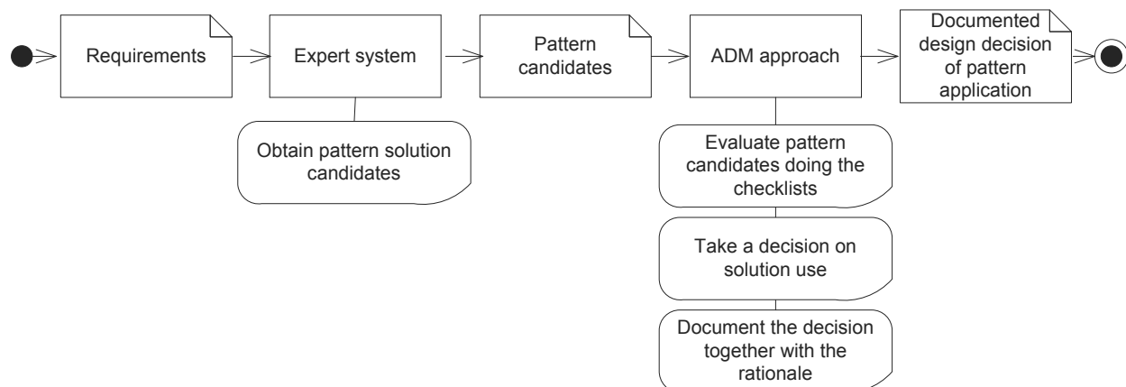
Figure 3.18.: Relation of an Expert System and the AM3D Approach in a Design Process
