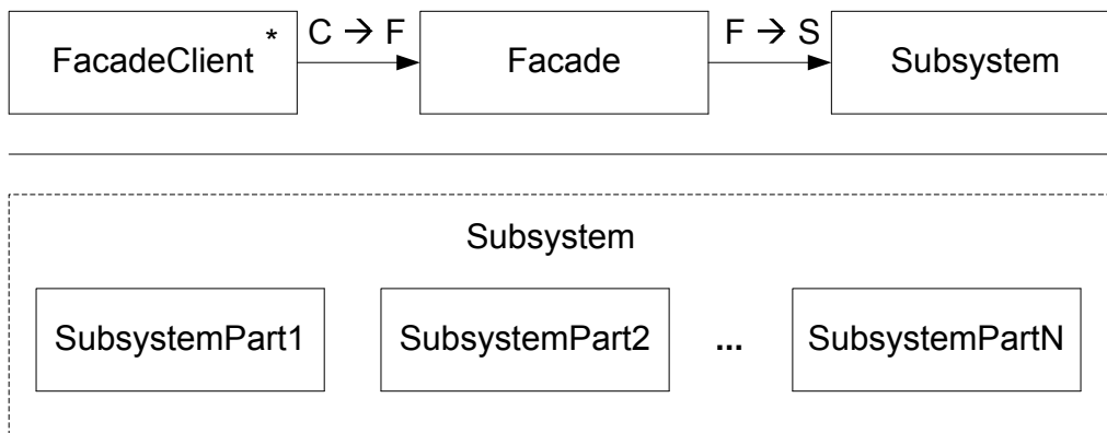
Figure 4.13.: An Example of Roles and Connectors Representation for the Façade Pattern
