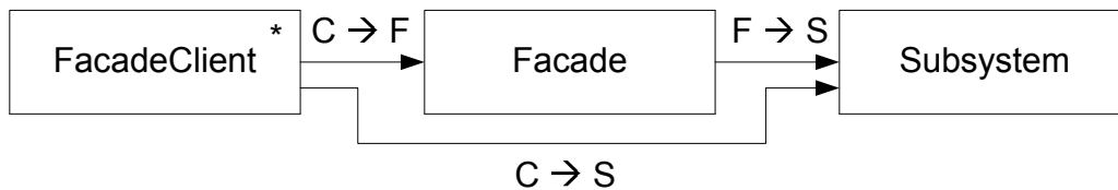
Figure 4.15.: An Example of Roles and Connectors Representation for the Variant of Façade Pattern
