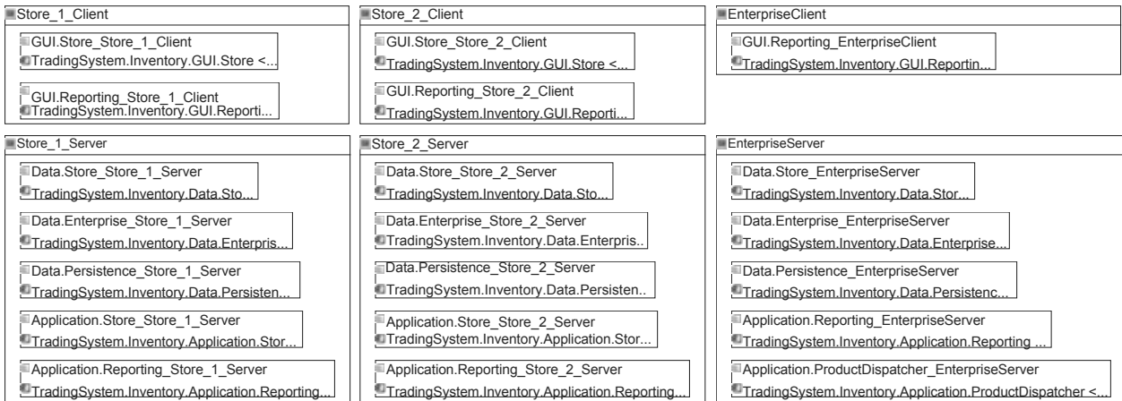
Figure 3.20.: Deployment Model of the CoCoME Architecture in PCM System View [158] (Repetition from Section 2.5.2)
