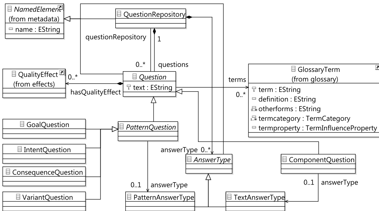
Figure 4.34.: Questions Meta-Model Package
