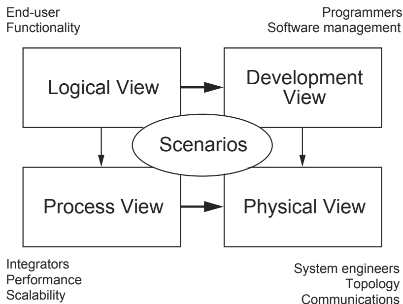
Figure 2.7.: 4 + 1 View Model [123]
