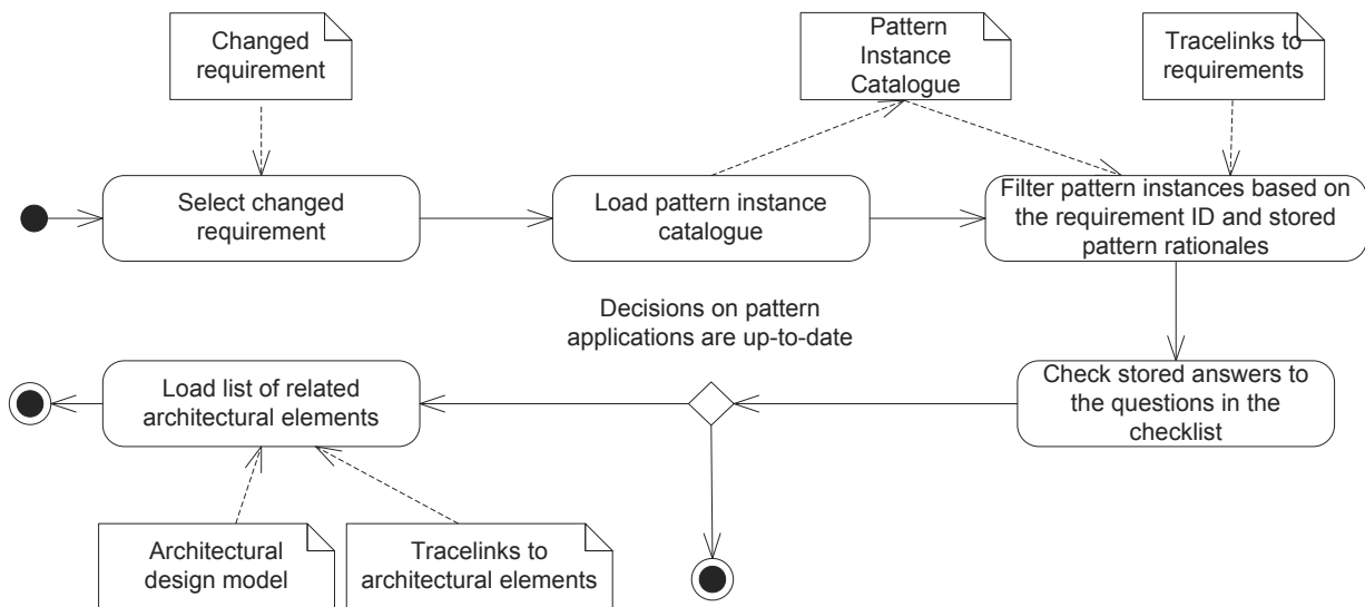
Figure 3.11.: Activity Diagram of Tracing Impact Caused by Changed Requirements Use Case
