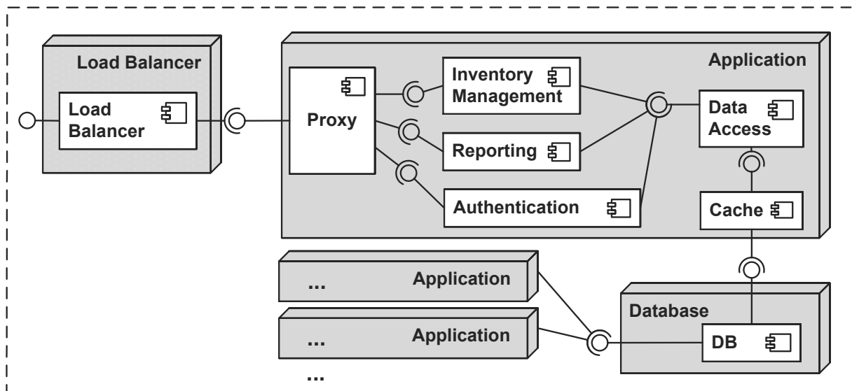
Figure 3.24.: Modified Hexxon CoCoMe Architecture of the Enterprise Server (Adopted from [2])
