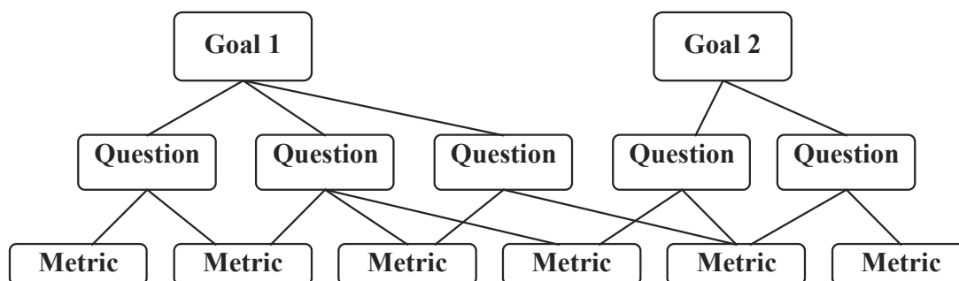
Figure 6.2.: Hierarchical Structure of the Goal Question Metric Approach [172]
