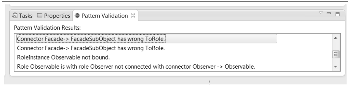
Figure 4.11.: An Example of Structural Check of the Façade Pattern in a PCM System Model
