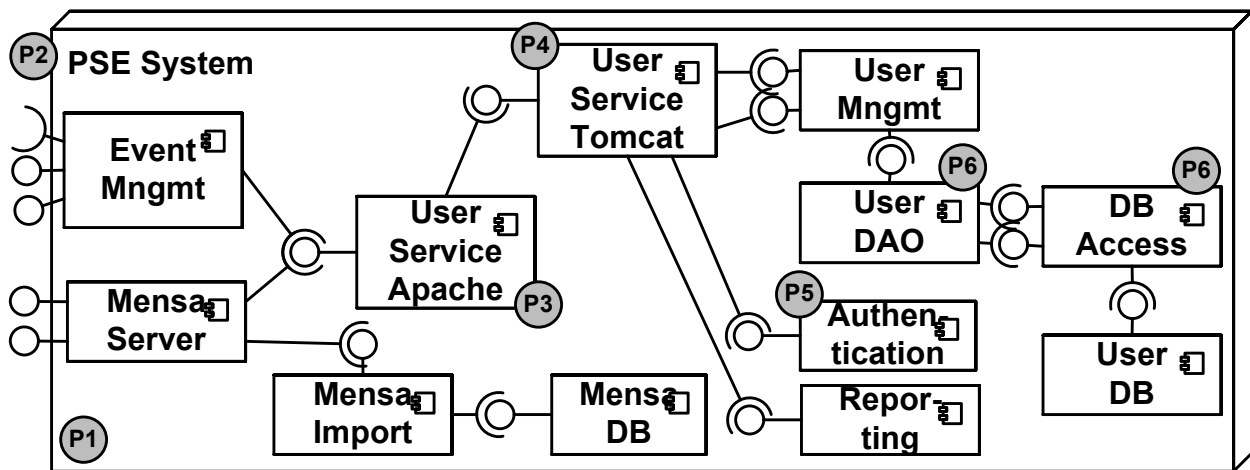
Figure 6.4.: System View of the PSE Architecture with Marked Pattern Positions (P)
