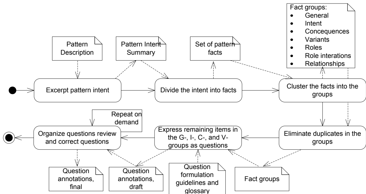
Figure 4.20.: A Process to Add Questions to a Pattern
