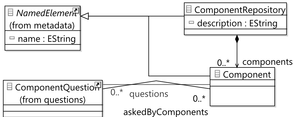
Figure 4.35.: Components Meta-Model Package
