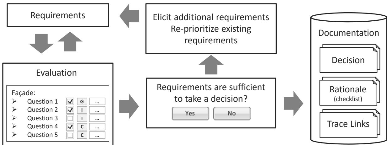
Figure 3.14.: Schematic Representation of Process to Document Trace Links
