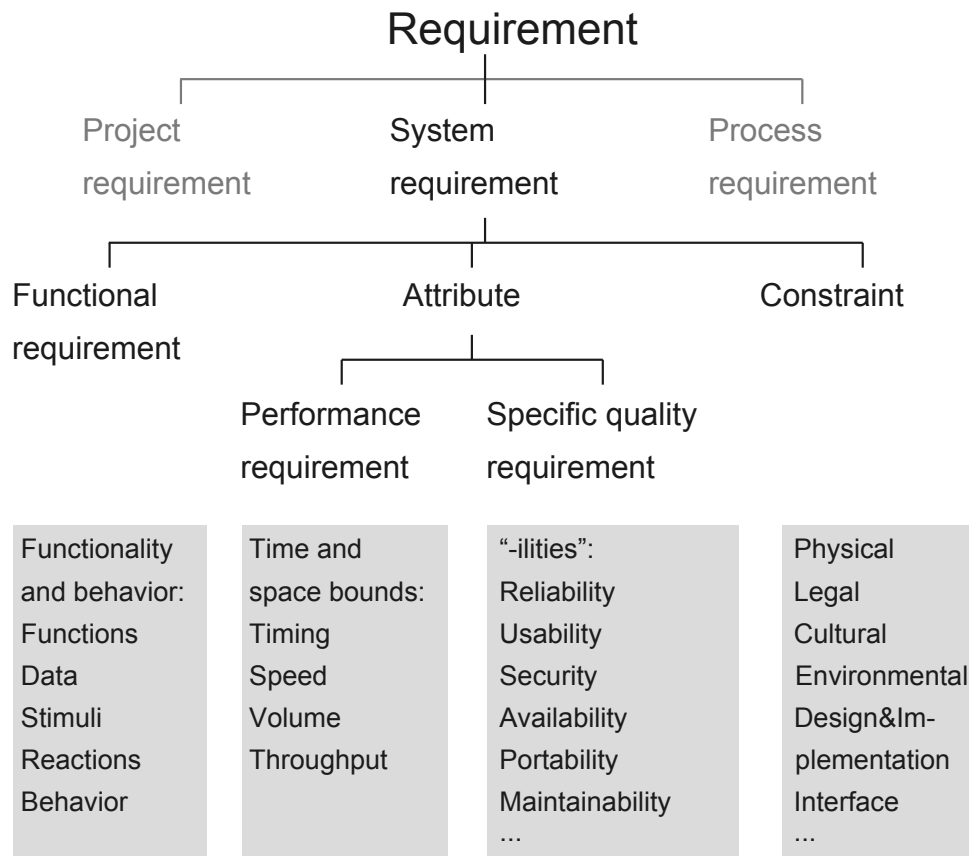
Figure 2.3.: A Concern-based Taxonomy of Requirements [104]
