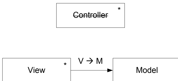
Figure 4.14.: An Example of Roles and Connectors Representation for the Variant of Model View Controller Pattern
