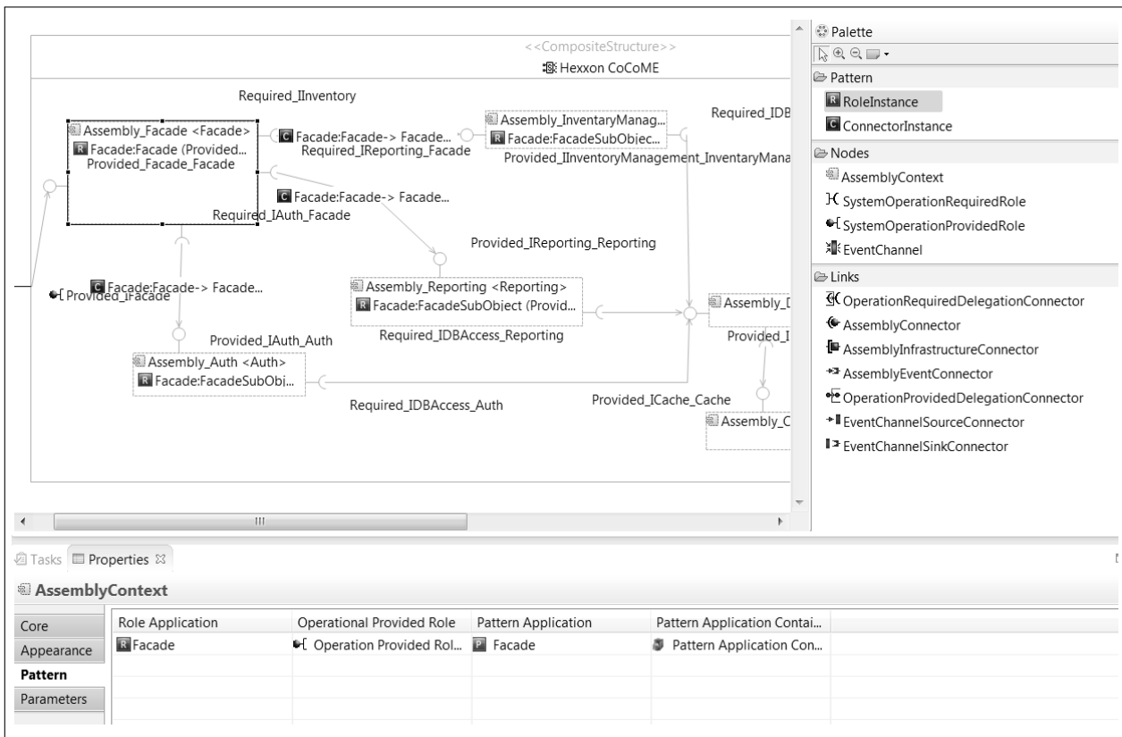
Figure 4.10.: An Example of Instantiation of the Façade Pattern in a PCM System Model (Repetition from Section 3)
