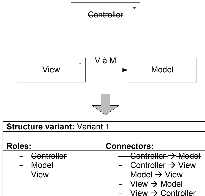
Figure 4.17.: An Example of a Textual Representation for the Model View Controller Pattern Variant
