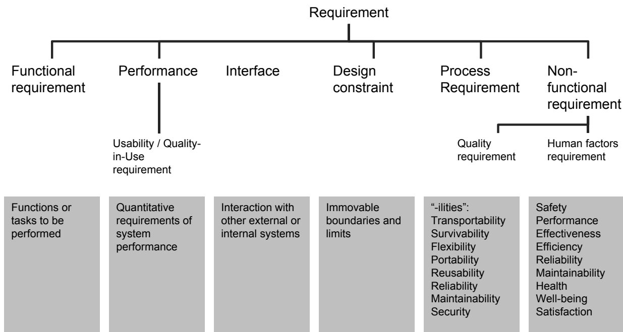
Figure 2.4.: An IEEE Standard Taxonomy of Requirement Types (Abstracted from Textural Description in [102])
