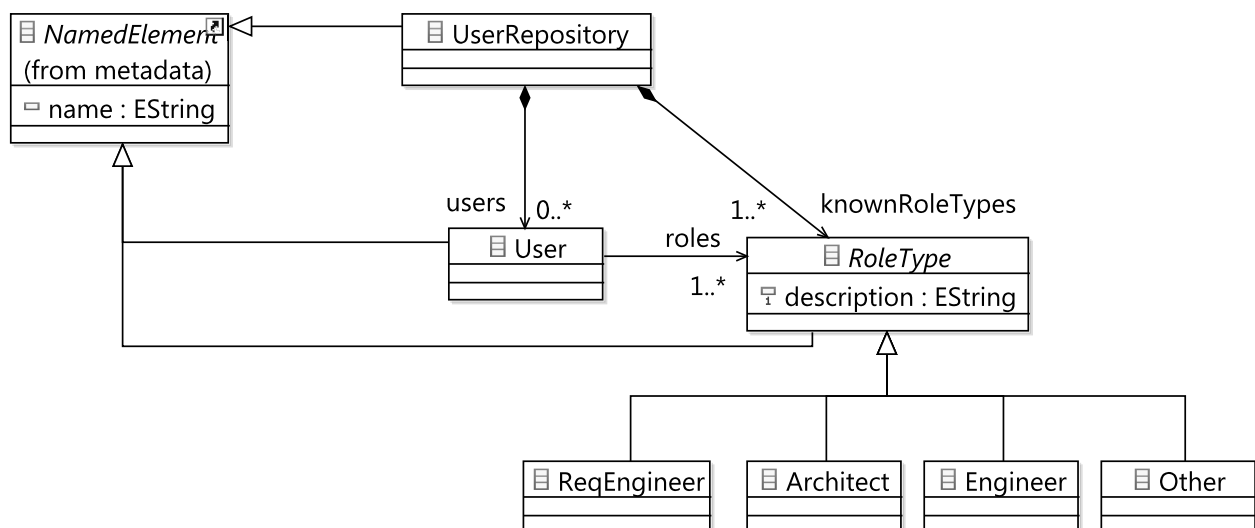
Figure 4.28.: Users Meta-Model Package
