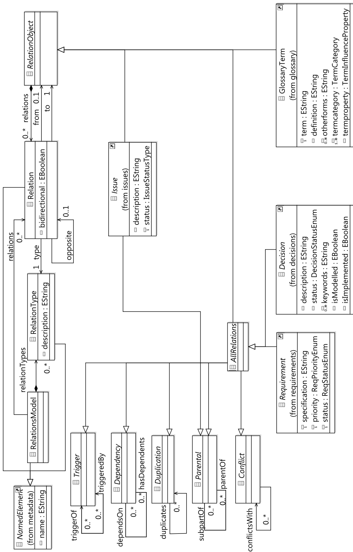
Figure 4.39.: Relations Meta-Model Package
