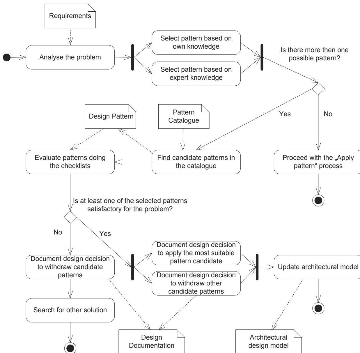
Figure 3.7.: Activity Diagram of Select Between Similar Patterns Use Case
