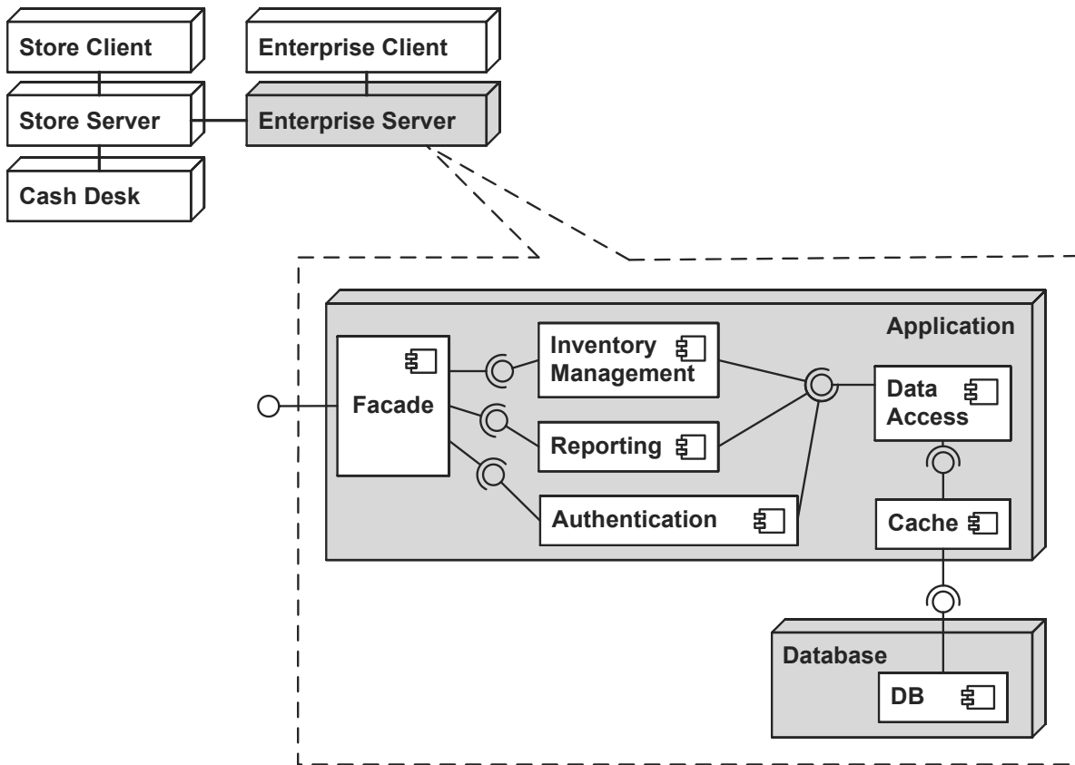
Figure 3.21.: Hexxon CoCoME Architecture of the Enterprise Server (Adopted from [2])
