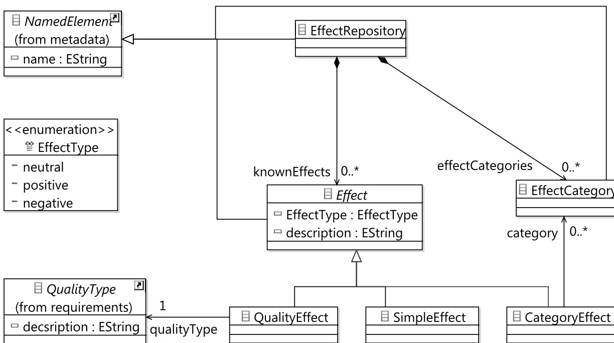
Figure 4.27.: Effects Meta-Model Package
