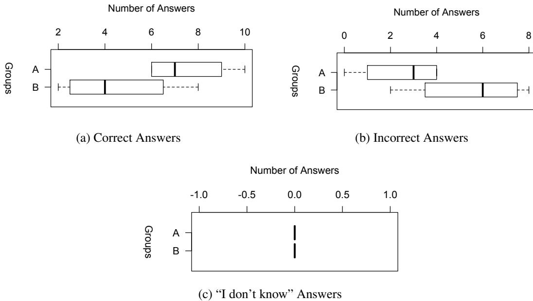
Figure 6.7.: Boxplots to Pattern Selection
