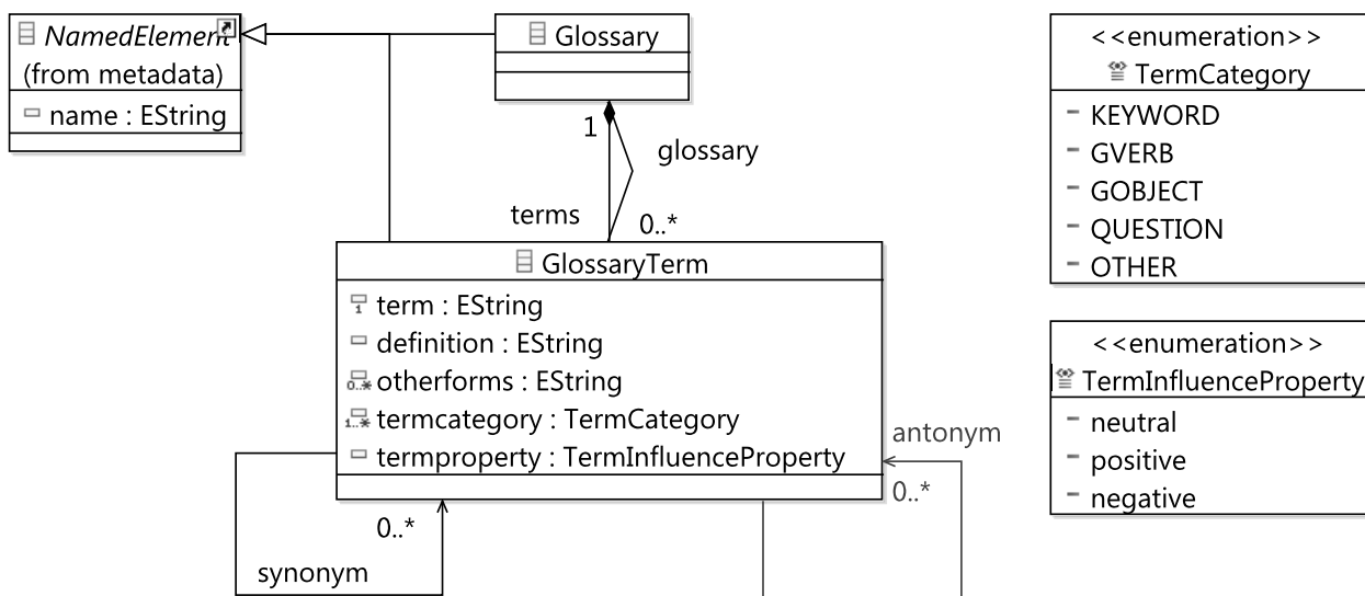
Figure 4.29.: Glossary Meta-Model Package
