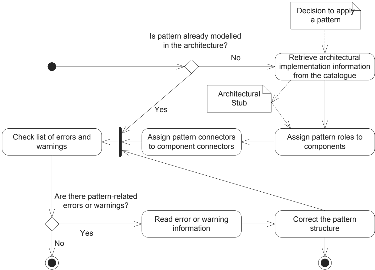
Figure 3.13.: Activity Diagram of Check Architectural Implementation Violations Use Case
