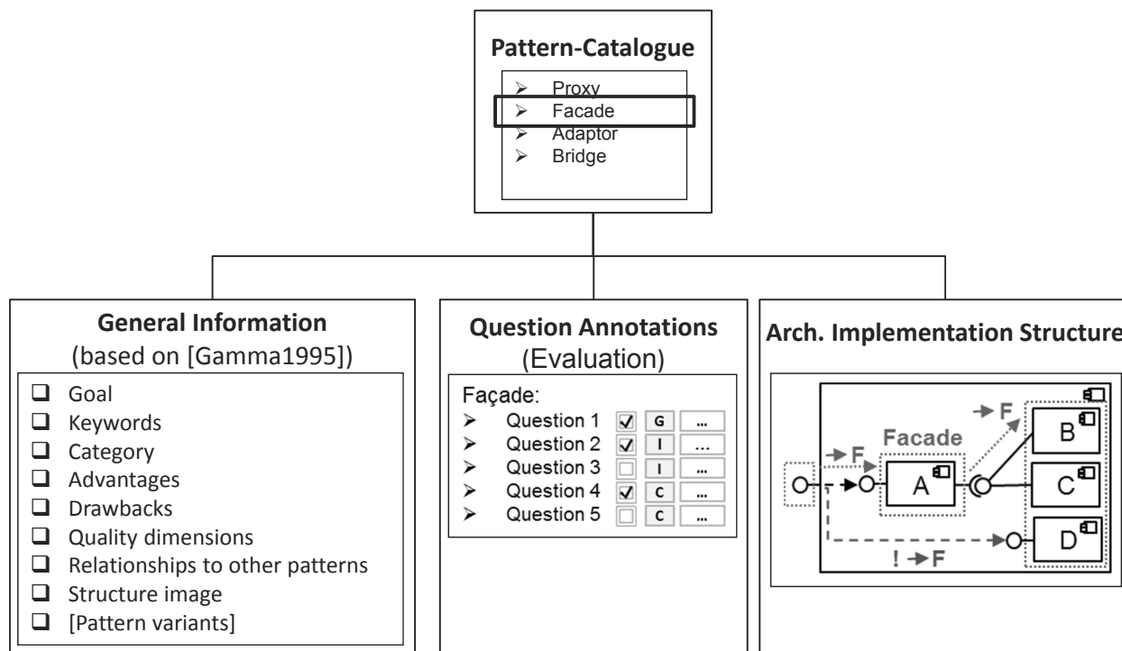
Figure 4.1.: Overview of the Catalogue Structure
