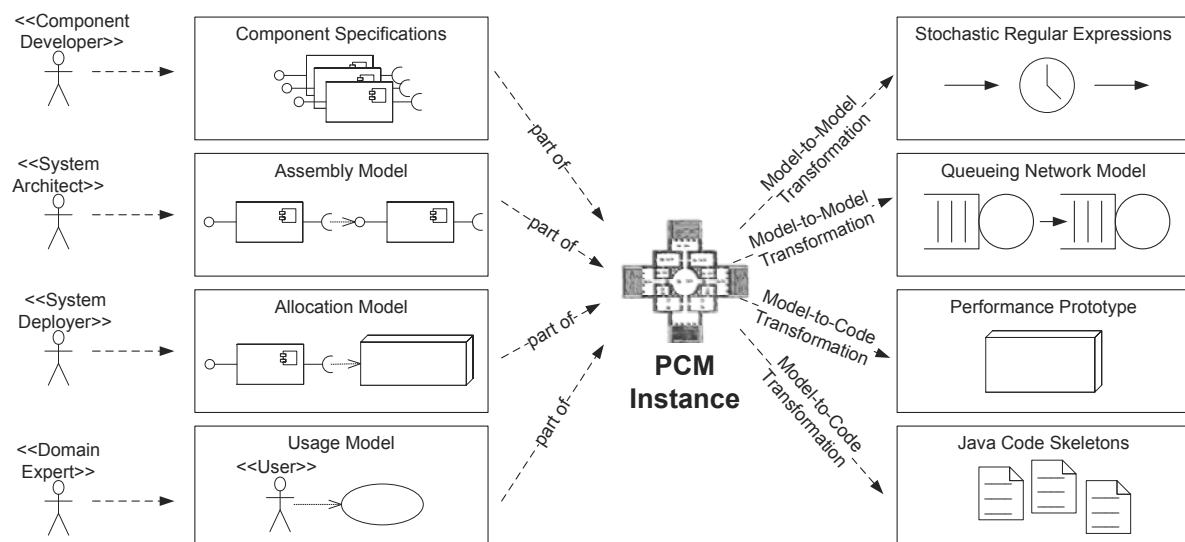
Figure 2.12.: The Overview of the PCM Approach [152]
