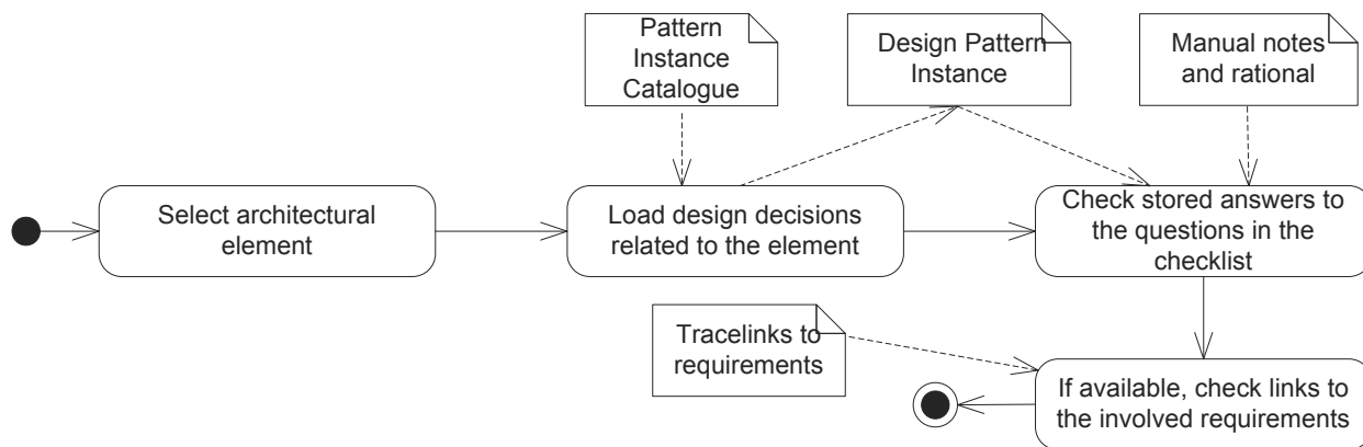
Figure 3.12.: Activity Diagram of Understanding of Rationale of Architectural Elements Use Case
