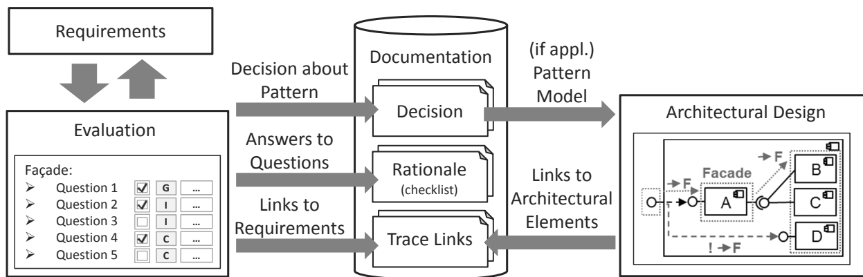
Figure 3.15.: Schematic Representation of Information Sources for Trace Link Documentation
