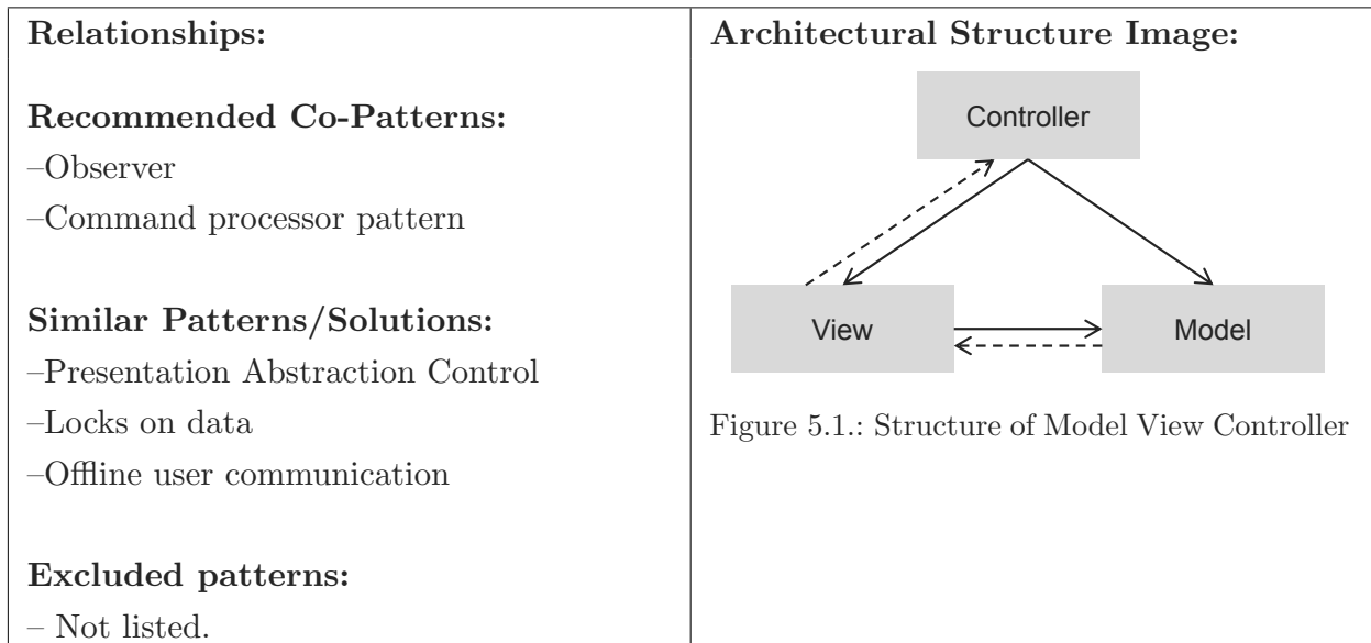
Figure 4.6.: An Example of Relationships and a Structural Image of an AM3D Pattern Catalogue Entry for Model View Controller Pattern
