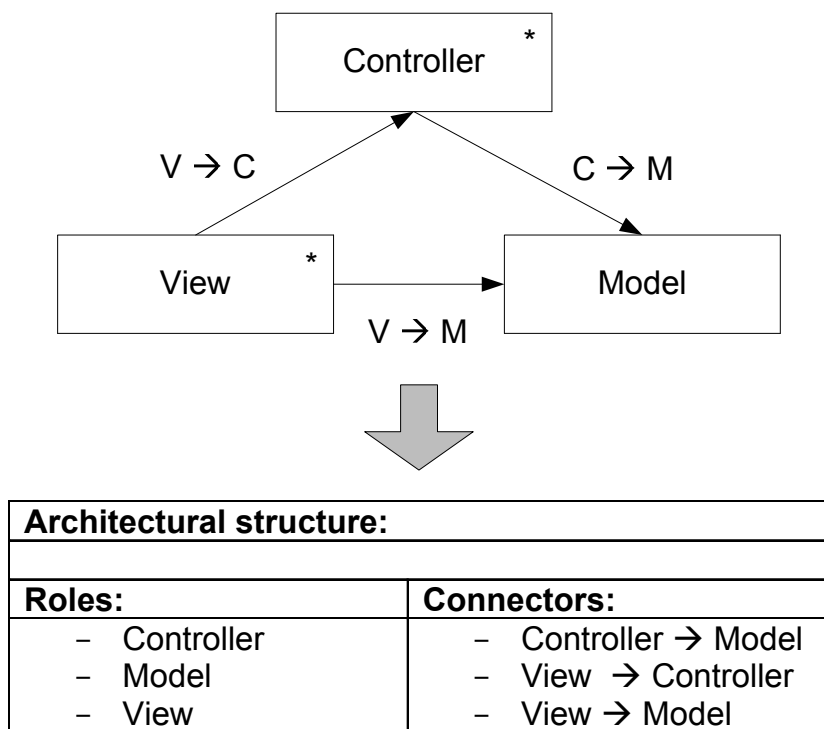
Figure 4.16.: An Example of a Textual Representation for the Model View Controller Pattern
