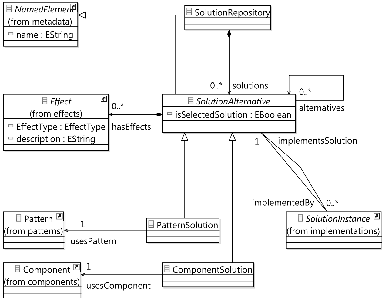
Figure 4.32.: Solutions Meta-Model Package
