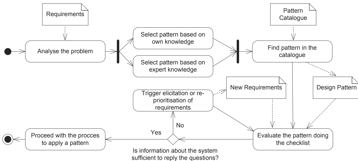
Figure 3.8.: Activity Diagram of Requirements Elicitation and prioritization Use Case
