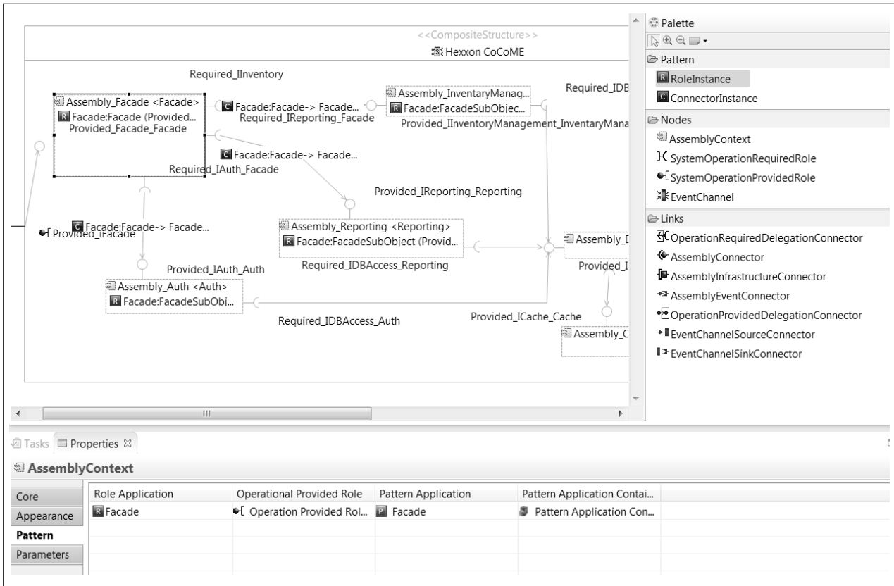
Figure 3.23.: Instantiation of the Façade Pattern in a PCM System Model
