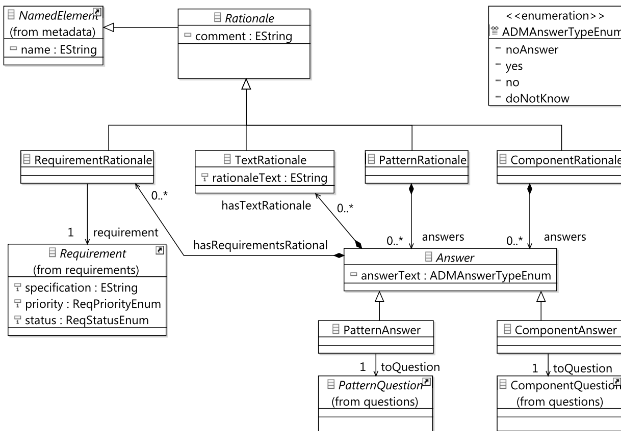
Figure 4.38.: Rationales Meta-Model Package
