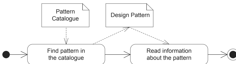
Figure 3.5.: Activity Diagram for Gaining Information About Pattern Use Case
