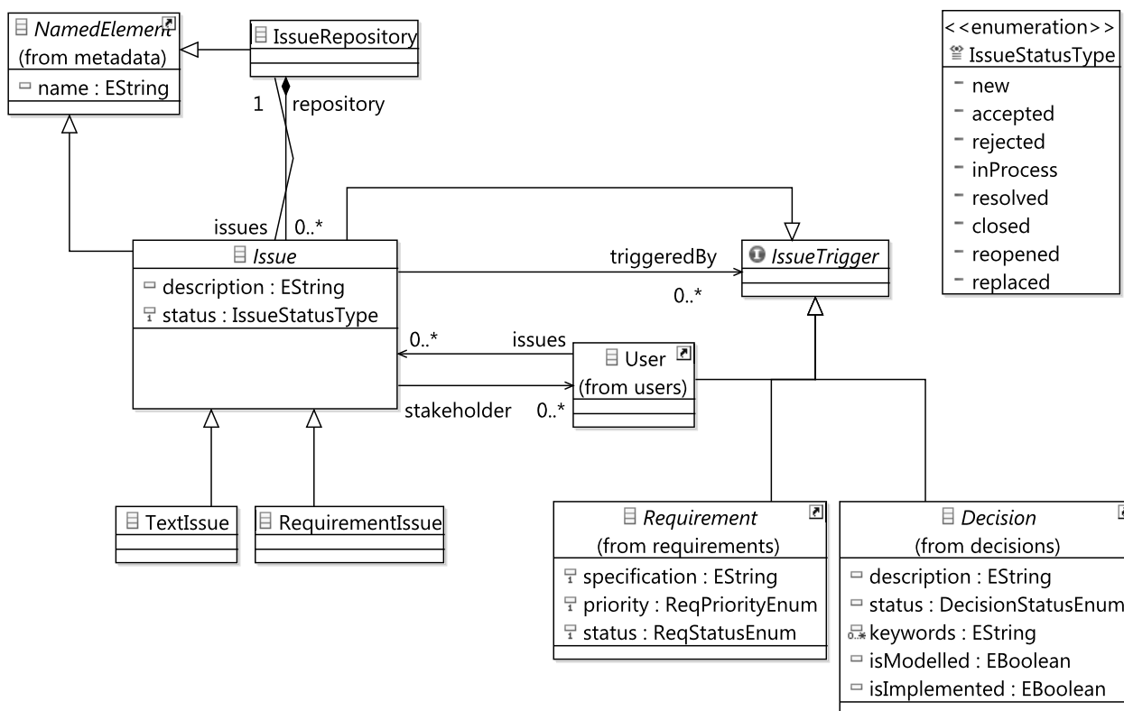
Figure 4.31.: Issues Meta-Model Package
