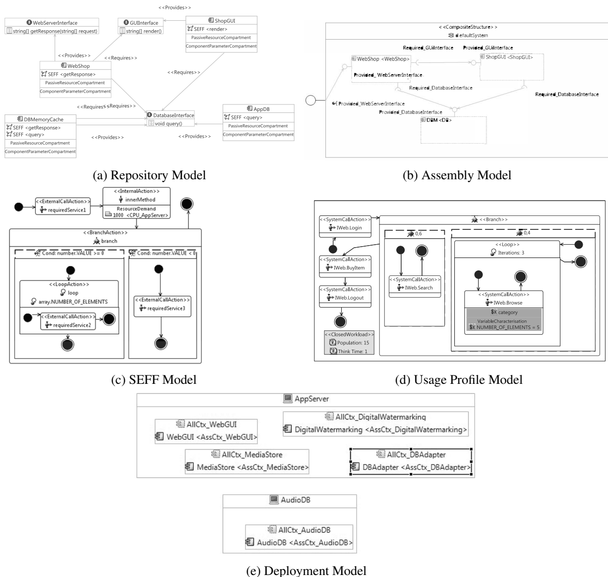
Figure 2.13.: PCM Model Views [152, 154]
