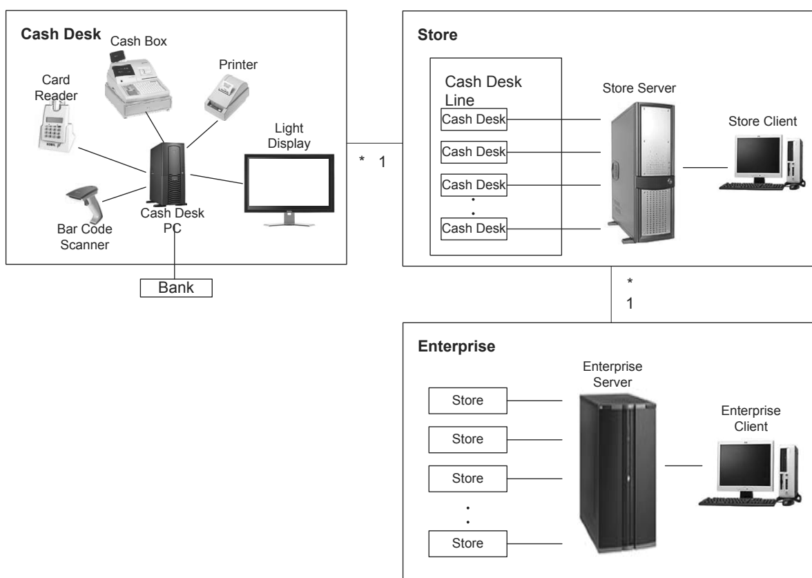
Figure 2.14.: Overview of the CoCoME System (Adopted from [155])
