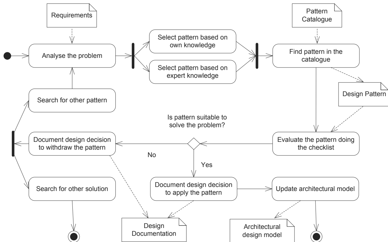
Figure 3.6.: Activity Diagram of Pattern Application Use Case
