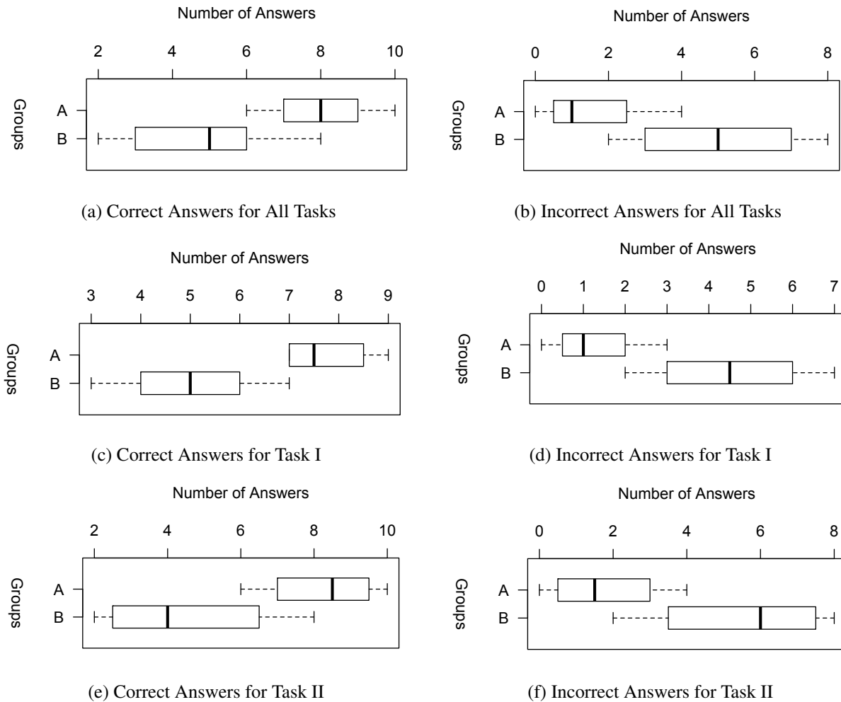
Figure 6.10.: Boxplots to Pattern Re-Evaluation
