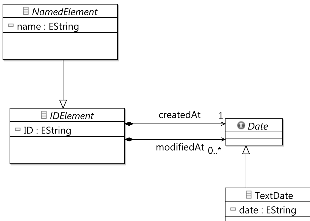
Figure 4.26.: Metadata Meta-Model Package
