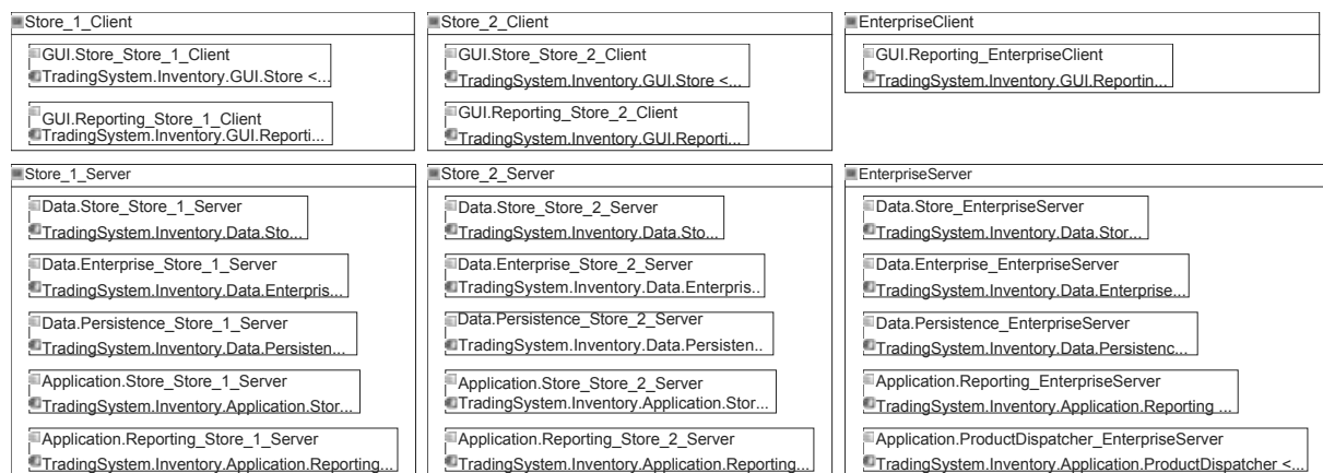
Figure 2.17.: Deployment Model of the CoCoME Architecture in PCM System View [158]
