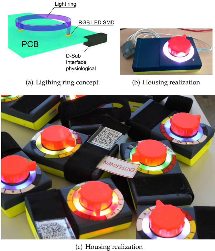
Figure 5.14: Housing and lighting system - first wearable prototype
