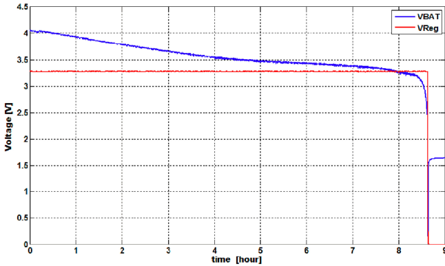
Figure 5.15: Discharge curve first wearable prototype
