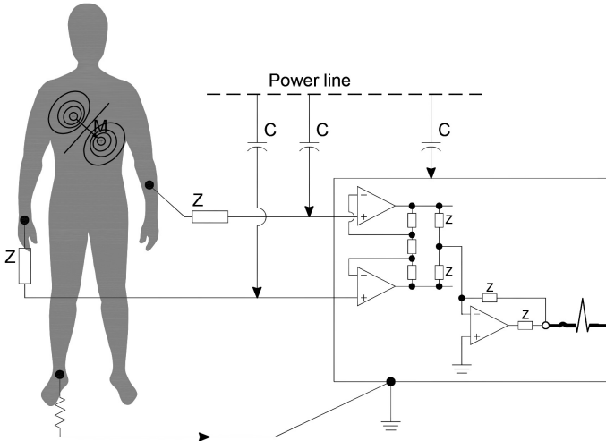
Figure 2.13: Electrocardiograph [Web09]
