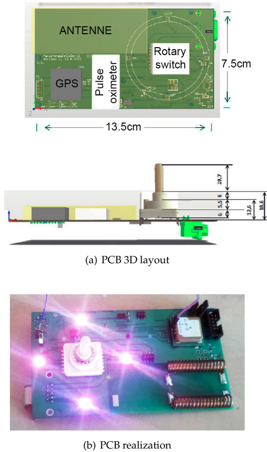
Figure 5.12: PCB first waerable prototype
