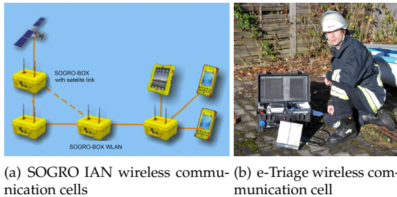
Figure 3.3: IAN wireless communication cells of projects SOGRO and e-Triage [EL12, AKGM + 11]
