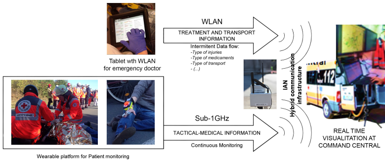
Figure 6.1: Developed IAN for MCI with wearable platform for continuous monitoring of patients
