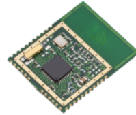
Figure 5.4: IMST RF module
