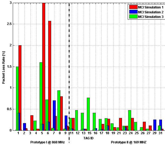
Figure 6.5: Packet loss rate for both wearable prototypes
