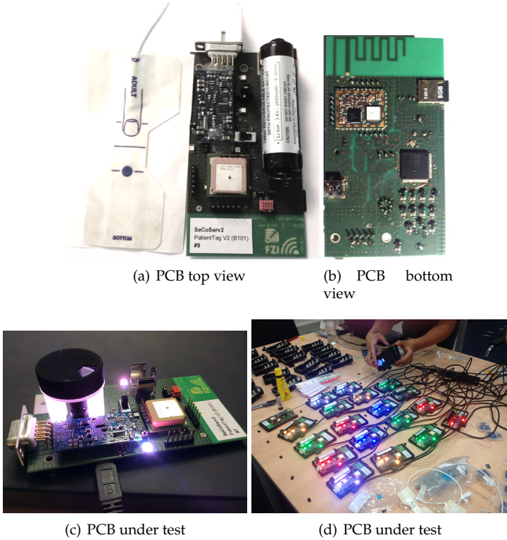
Figure 5.16: PCB realization for the second prototype
