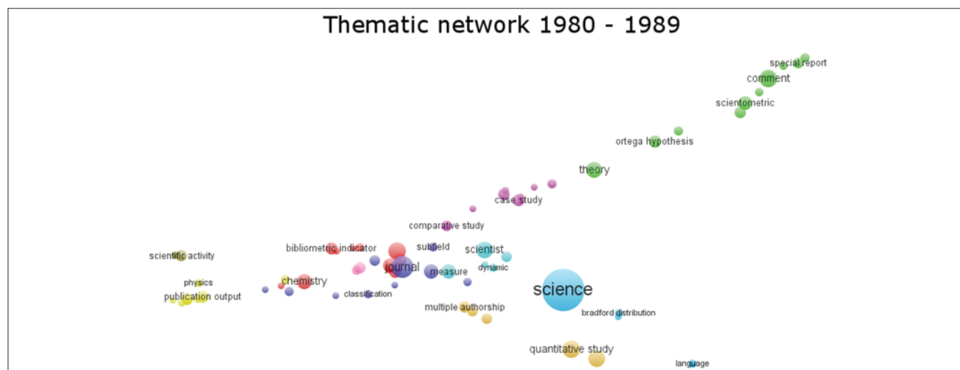
Figure 4: Thematic network 1980-1989
