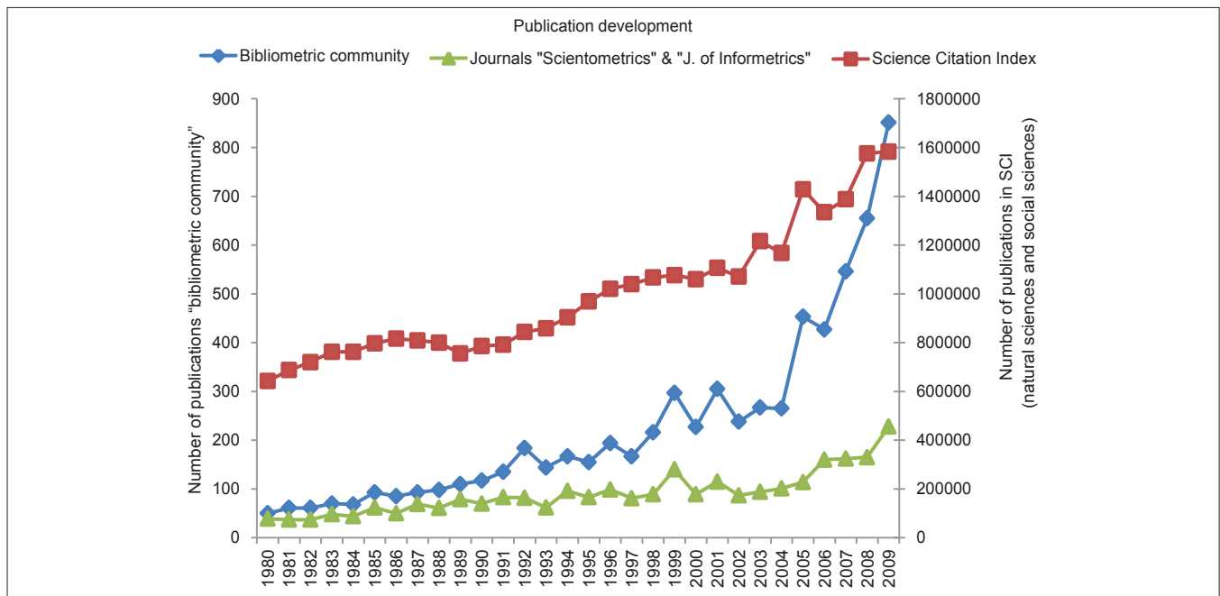
Figure 1: Publication development
