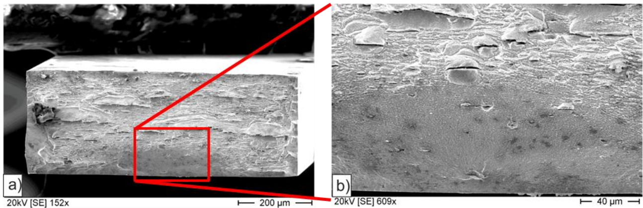
Figure 8. Fracture surface of t-HPT-10 (a) whole fracture surface (b) crack initiation area at the surface without nonmetallic inclusion and fatigue fracture surface.
