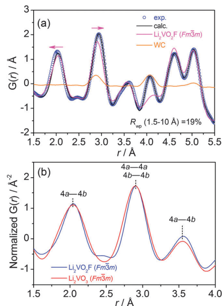
Fig. 3 (a) Experimental and calculated (using Rietveld average structure model) atomic PDF profile for \text{Li}_2\text{VO}_2\text{F} , U_{\text{iso}} (\text{\AA}^2) parameters for Li, V, O and F are 0.0024, 0.0122, 0.0128 and 0.1721, respectively. (b) Modelled PDF profiles for two Fm\bar{3}m phases with oxo and oxofluoro anion ligands in the r -range of 1.5–4 \text{\AA} .
