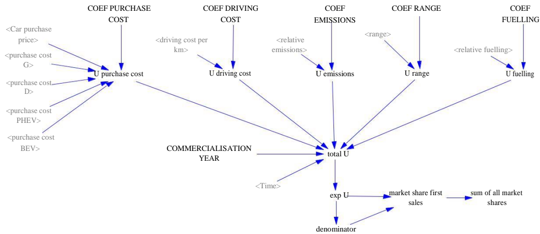
Figure 9 – Structure of the module “Technology Choice” Source: own work using Vensim®
