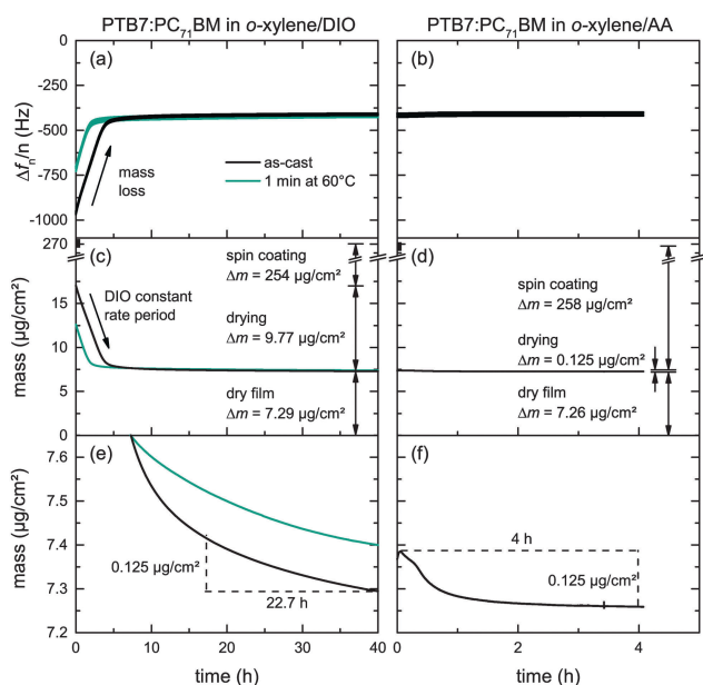
Fig. 5 Drying characteristics of PTB7:PC 71 BM at 25 \text{ }^\circ\text{C} cast from o -xylene/DIO and o -xylene/AA (2% v/v). (a and b) QCM measurements after spin coating. The changes in the resonance frequencies reflect mass loss. (c and d) Drying curves calculated from the QCM frequency change using the Sauerbrey equation. Whereas only very little mass loss is observed for o -xylene/AA films, o -xylene/DIO films show a constant initial mass decrease, characteristic of evaporation of the additive at the vapor-liquid interface. (e and f) Zoom into the relevant mass regime of the falling rate period of the drying curve, where the mass loss is determined by the diffusion of the additive inside the PTB7:PC 71 BM matrix. AA diffuses faster than DIO.
