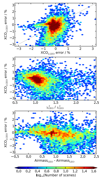
Figure 11. Relative aerosol and cirrus induced XCO_2 forward model errors (retrieved/true – 1) found by the GEO configuration as a function of the relative XCO_2 errors (retrieved/true – 1) in LEO configuration (upper panel), the ratio of \chi^2 in GEO and LEO configuration (middle panel), and the difference between slant airmass in GEO and LEO configuration (lower panel). Thereby, \chi^2 is calculated via \frac{1}{N_{DFS}} \sum_i \frac{(y_{i,meas} - y_{i,mod})^2}{\sigma_i^2} where the sum is over all detector pixels i , y_{i,meas} and y_{i,mod} are the measured and the modelled radiance, \sigma_i is the noise error, and N_{DFS} is the number of degrees of freedom for signal. Slant airmass is calculated via 1/\cos(SZA) + 1/\cos(VZA) with solar zenith angle SZA and viewing zenith angle VZA. The color scale shows logarithmic occurrence. Note that the scale of residual XCO_2 errors is inflated by a factor 1.5 compared to Fig. 10 to cover the more challenging cases.
