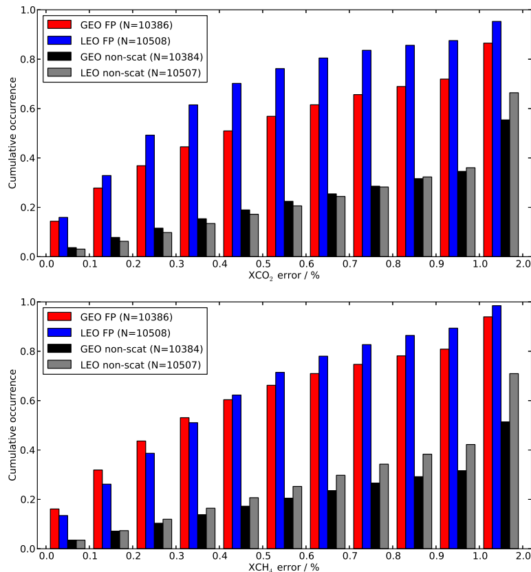
Figure 12. Cumulative relative occurrence of XCO_2 (upper) and XCH_4 (lower) errors for the full-physics (FP) and non-scattering (non-scat) retrievals mimicking a LEO or a GEO satellite as indicated by the legend. Number N of successful retrievals as indicated by the legend. Only non-scattering retrievals that pass the corresponding full-physics retrievals are taken for the counting. Full-physics quality filters screen non-convergent behavior, ocean surfaces, VZA > 70^\circ , SZA > 70^\circ , and SNR-limited dark scenes in SWIR-3 ( \text{albedo} \times \cos(SZA) / \pi < 0.005 ).
