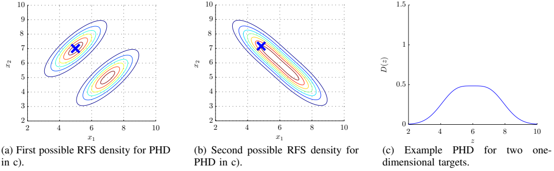
Fig. 1: Example 1: A PHD for two one-dimensional targets and two possible RFS densities. The MMOSPA estimates for the RFS densities (blue crosses) do not coincide.
