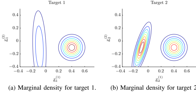
Fig. 3: Illustration of the (four-dimensional) joint density for two two-dimensional targets used in the evaluation: Intuitively, one target is approximately at location [-0.1, -0.1]^T and the other one is at [0.4, -0.1]^T . Also note that the correlations are not visible from the marginal densities. The correlations exclude the case that the two targets are at the same location. We use \underline{x}_1^{(1)} and \underline{x}_2^{(2)} to denote the first and second component of the vector \underline{x}_1 (same notation for \underline{x}_2 ).
