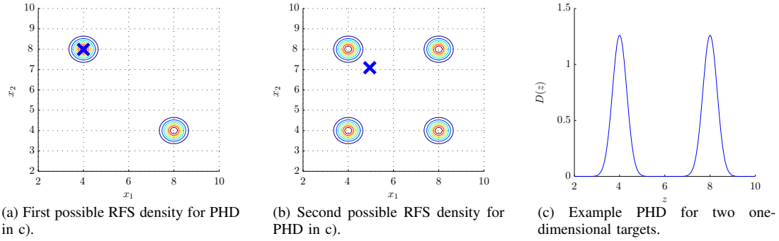
Fig. 2: Example 2: A PHD for two one-dimensional targets and two possible RFS densities. The MMOSPA estimates for the RFS densities (blue crosses) are significantly different.
