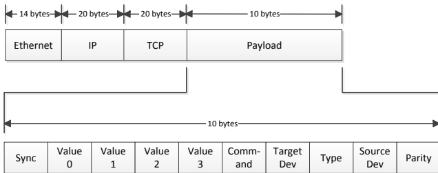
Figure 6. Structure of a GLORIA telecommand data packet encapsulated in a TCP/IP frame. The synchronisation byte is followed by four optional-value bytes and by the command byte, indicating which action to take. In addition, the target device as well as the source device are included in the packet. The type byte indicates how the four value bytes should be interpreted as shown in Table 2.
