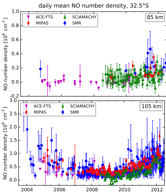
Figure 4. NO time series comparison as in Fig. 3 for 32.5° S.
