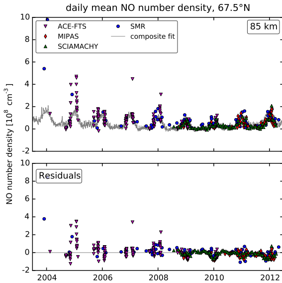
Figure 11. NO time series regression results at 67.5^\circ N, 85 km. The upper panel shows the individual time series and the composite regression fit using all data simultaneously. The lower panel shows the individual residuals with respect to the composite fit.
