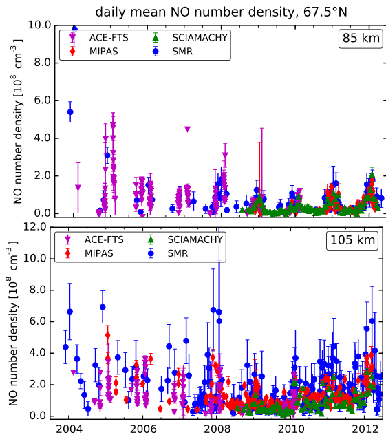
Figure 3. NO time series comparison of all four instruments at 67.5° N, for 85 km (top) and 105 km (bottom). The error bars indicate the statistical 95 % confidence interval of the daily zonal mean.
