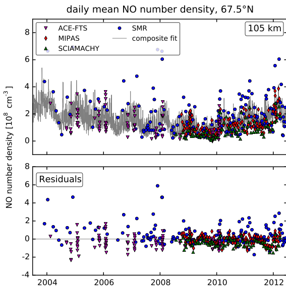
Figure 12. NO time series regression results at 67.5^\circ N, 105 km, as in Fig. 11.
