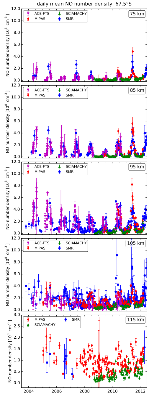
Figure B2. NO time series comparison of all four instruments at 67.5° S, for 75 km, 85 km, 95 km, 105 km, and 115 km (from top to bottom).
