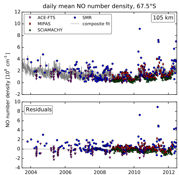
Figure 14. NO time series regression results at 67.5^\circ S, 105 km, as in Fig. 11.
