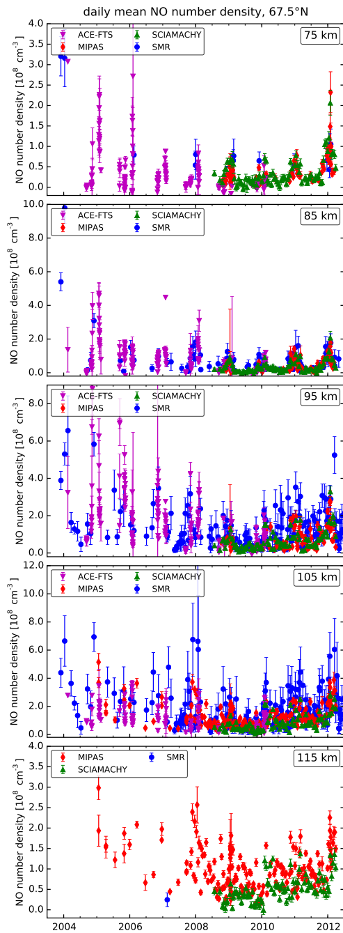
Figure B1. NO time series comparison of all four instruments at 67.5° N, for 75 km, 85 km, 95 km, 105 km, and 115 km (from top to bottom).
