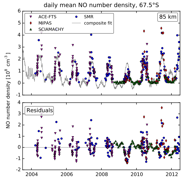
Figure 13. NO time series regression results at 67.5^\circ S, 85 km, as in Fig. 11.
