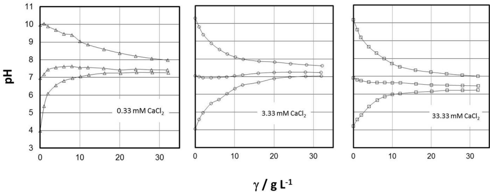
Figure 16. Potentiometric mass titrations of ACF2944 (Ca-form) at different ionic strengths: I_c (mol/dm 3 ): 0.001 ( \Delta ), 0.01 ( \circ ), and 0.1 ( \square ) \text{CaCl}_2 ; t=20^\circ\text{C} .
