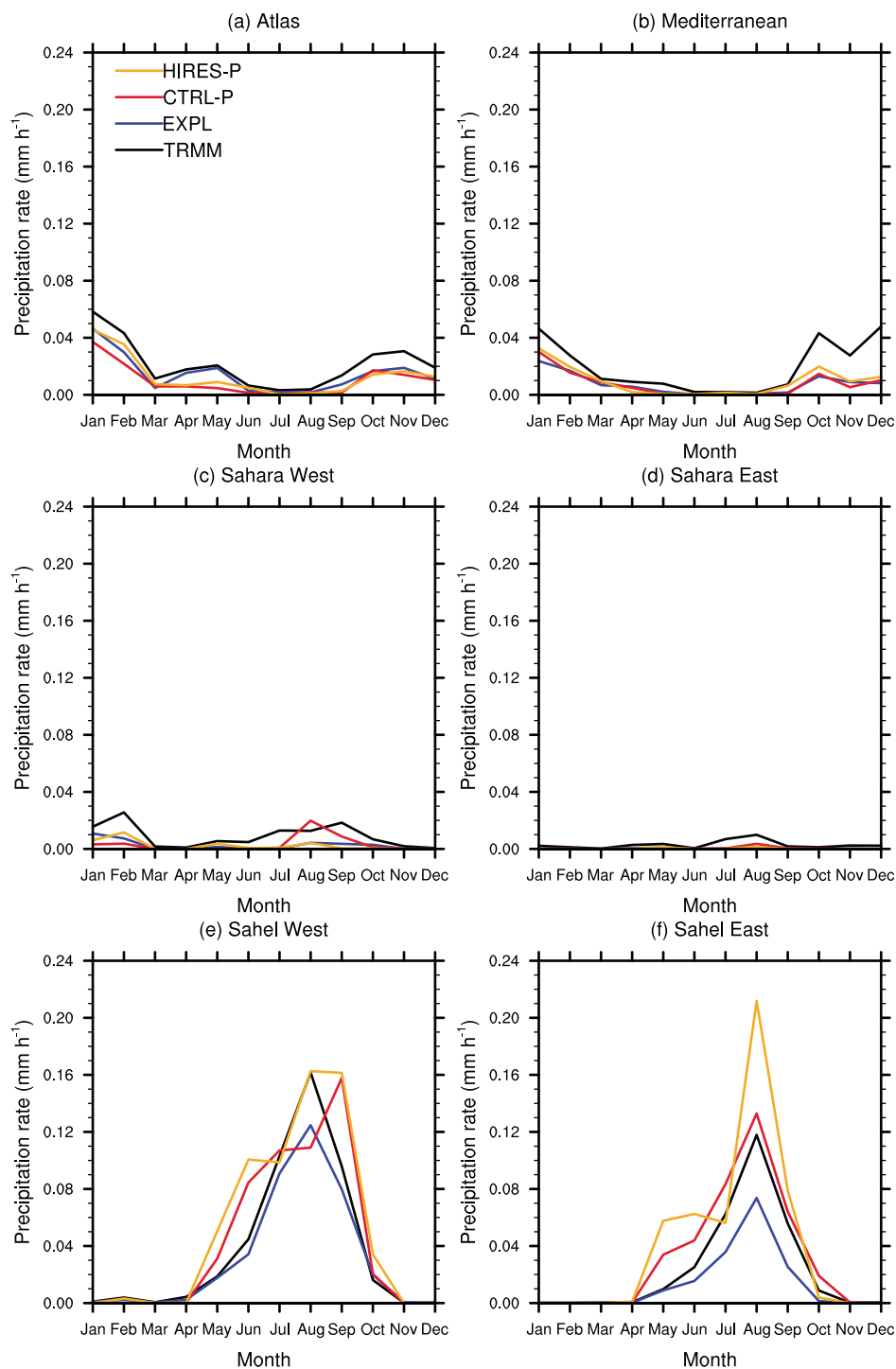
Figure 5. Seasonal cycle in precipitation rate averaged over each area marked by a box in Figure 4 in the TRMM-3B42 observation product and in the EXPL, CTRL-P, and Hires-P model runs (Table 1).
