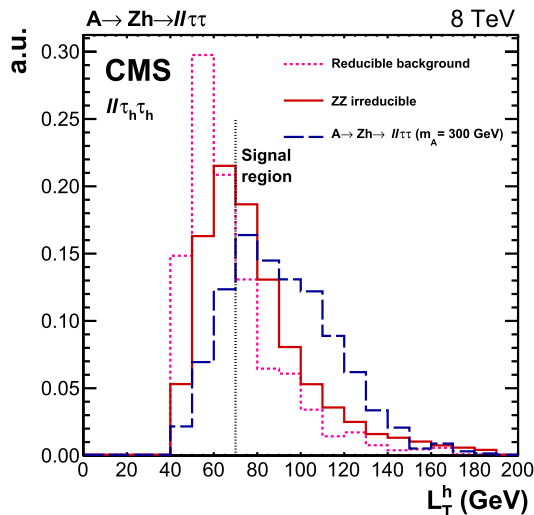
Fig. 2. Distribution of the variable L_T^h for events in the ll\tau_h\tau_h final state. The reducible background is estimated from data, instead the ZZ irreducible background from simulation.
