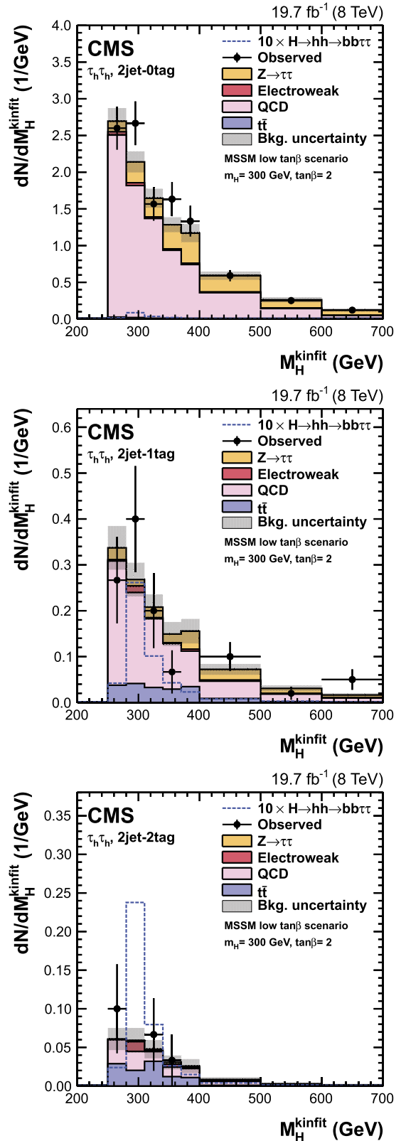
Fig. 5. Distributions of the reconstructed four-body mass with the kinematic fit after applying mass selections on m_{\tau\tau} and m_{bb} in the \tau_h \tau_h channel. The plots are shown for events in the 2jet-0tag (top), 2jet-1tag (middle), and 2jet-2tag (bottom) categories. The expected signal scaled by a factor 10 is shown superimposed as an open dashed histogram for \tan\beta = 2 and m_H = 300 GeV in the low \tan\beta scenario of the MSSM. Expected background contributions are shown for the values of nuisance parameters (systematic uncertainties) obtained after fitting the signal plus background hypothesis to the data.
