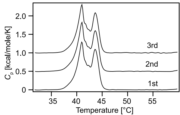
FIG. 4. Differential scanning calorimetry of D-Gb3 suspension recorded at a heating rate of 10°C/h yielding a main transition enthalpy of \Delta H = 4.7 kcal/mol. Successive heating scans exhibited no hysteresis. Each of the scan is separated by an offset of 0.5 kcal/mol/K in a vertical direction for the clarity.
