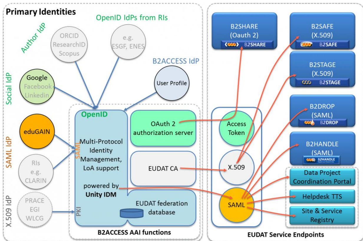
Figure 2.3: EUDAT architecture
