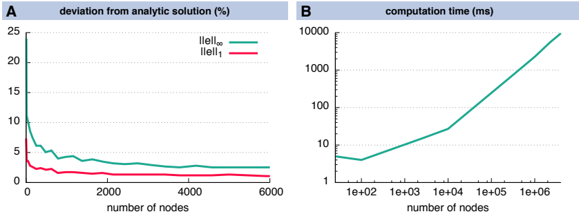
Figure 8.7: Deviation of the fast marching solution from the analytic solution of a radial wave (A). Excitation spread was computed on quadratical planar meshes composed of right-angled triangles. The mean error \|e\|_1 and the maximum error \|e\|_\infty was evaluated for different numbers of nodes. The dependence of the computation time for one complete activation cycle on the number of nodes (B) was dominated by the linear part of \mathcal{O}(N \log N) .
