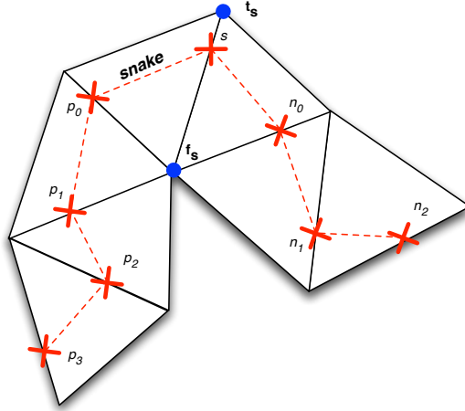
Figure 8.2: Geometric snake on a triangular mesh. The snake segments run on the surface of the triangles from snaxel to snaxel. Each snaxel is constrained to its supporting edge. Snaxel s is supported by the edge running from \mathbf{f}_s to \mathbf{t}_s and directly connected to its predecessor \mathbf{p}_0 and its successor \mathbf{n}_0 .
