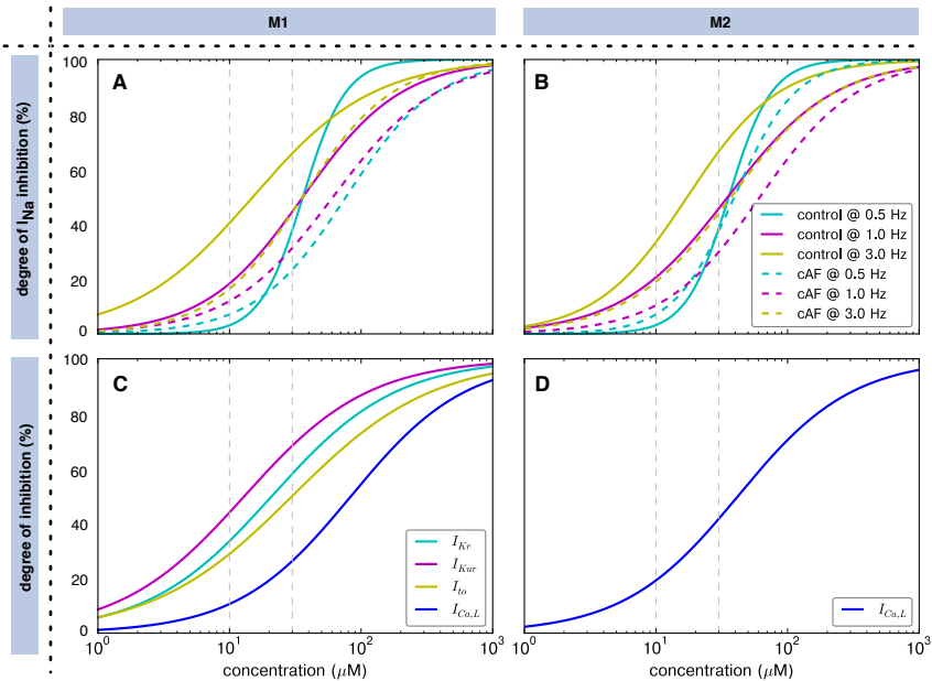
Figure 6.8: Dose response of veranakalant induced I_{Na} block depending on the pacing frequency and the substrate in M1 (A) and M2 (B) (cf. Table 6.3). The vertical lines indicate the concentration span covered in the study by Wetter et al. [376]. The frequency and substrate independent degree of block of other cardiac ion currents is shown in (C) for M1 and (D) for M2.
