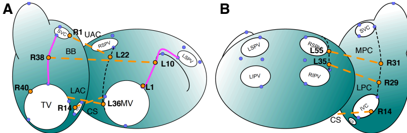
Figure 7.9: Schematic course of the IACs (dashed orange lines) connecting the start points in the RA and the end points in the LA directly. The RA and LA extension of BB is indicated by the magenta line. The dashed black lines represent auxiliary paths used to locate start and end points (orange) of the IACs. Blue points represent the 22 landmarks points. (A) shows the anterior aspect, (B) the posterior aspect.
