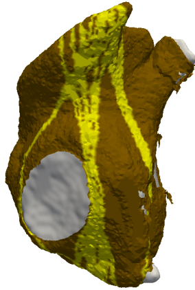
Figure 8.4: Example of an AFLut vulnerability map. The vulnerable paths are marked in yellow on the brown substrate of the RA; the blood pool is indicated in gray. Several paths run from the septal side of the TV to the RAA.
