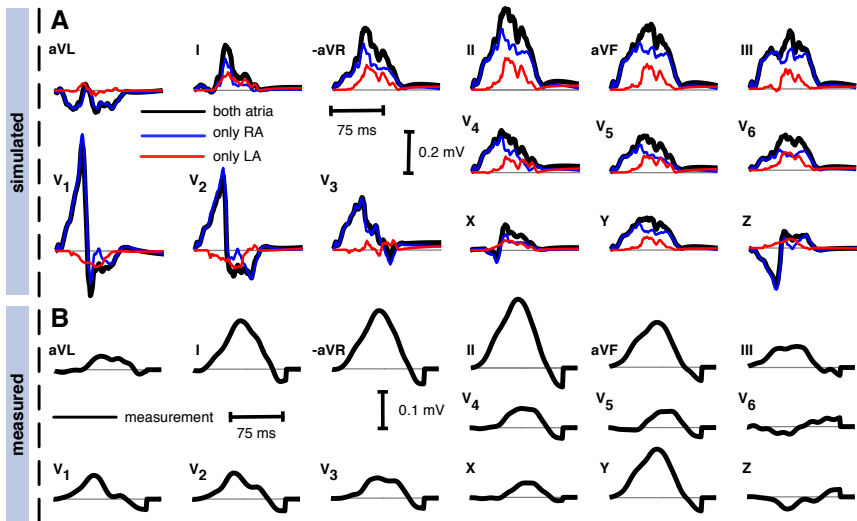
Figure 9.2: ECGs obtained through simulation using model #5 (A) and measurement in subject #5 (B). The iso-potential line is indicated by a thin grey line. In (A), the blue traces correspond to the right atrial P-wave whereas the the red ones stem from sources in the LA. LA and RA P-waves add up to the regular P-wave represented by the black traces.
