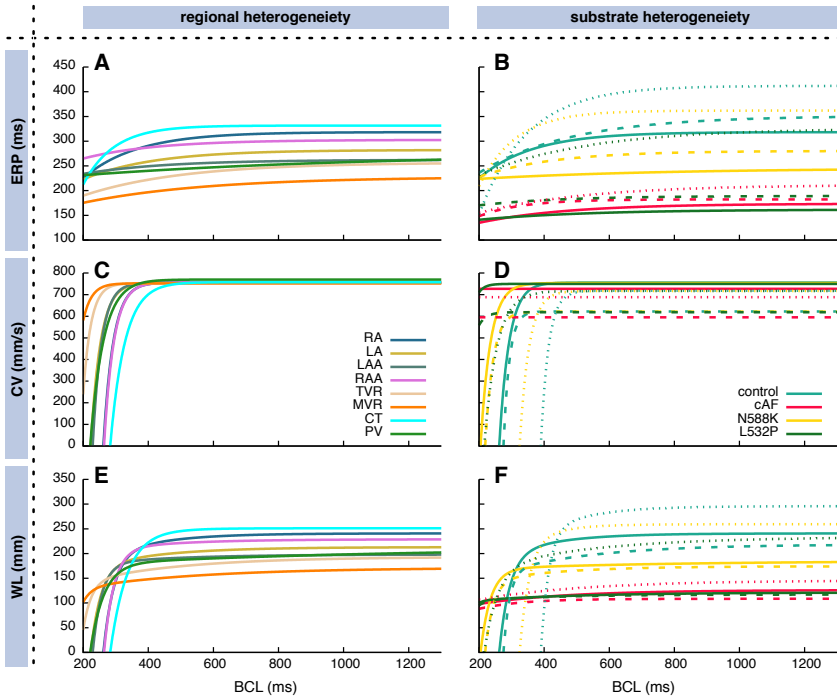
Figure 8.6: Fitted exponential restitution curves of ERP (A), (B) and CV (C), (D), as well as the WL as the product of the former measures (E), (F) for different anatomical regions in the atria (A), (C), (E) and different substrates (B), (D), (F). In (B), (D), and (F), the dashed lines represent the respective substrates under the influence of 2.3 \mu\text{M} amiodarone whereas the dotted lines represent the influence of 0.21 \mu\text{M} dronedarone. Exponential curves according to Equation (8.1) were used to fit the output of monodomain tissue strand simulations. The coefficients are listed in Table 8.1.
