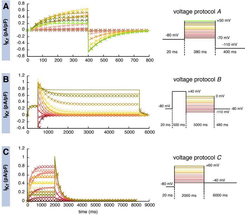
Figure 4.17: Resulting currents using the parameters estimated by the multivariate metamodelling approach. Solid lines indicate synthetic I_{K_r} input currents used for parameter estimation. Crosses represent the best fit obtained (not every sample shown for clarity reasons). The voltage protocols used to generate the input data and to challenge the ion current model are shown on the right part of each panel.
