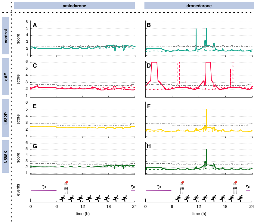
Figure 6.7: Circadian variation of the total score (Figure 6.6) along the trajectories through the BCL-concentration space representing a typical day (Figure 6.2 and Figure 6.3). The antiarrhythmic drugs amiodarone (A), (C), (E), and (G) and dronedarone (B), (D), (F), and (H) were assumed to be administered together with food (solid lines) or without (dashed lines) resulting in different bioavailability of the agents. The gray, dash-dotted lines indicate the baseline score at zero drug concentration. Resulting scores are shown in four different substrates: control (A)+(B), cAF induced remodeling (C)+(D), hERG mutation L532P (E)+(F), and hERG mutation N588K (G)+(H). The lower panels indicate times of sleep, drug (and possible food) intake, as well as phases of elevated heart rate representing physical activity.
