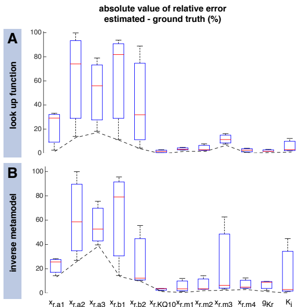
Figure 4.20: Distribution of the relative error of the estimated parameters for the three voltage protocols A, B, and C and the I_{K_r} input data. (A) shows the results obtained by the look up function, whereas (B) shows the results yielded by the inverse metamodel. The dashed line interpolates the minimum values linearly.
