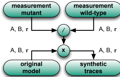
Figure 5.1: Transfer of measured currents into synthetic traces used to estimate parameters. Exponential coefficients were estimated for mutant and WT measured traces, as well as the output of the Courtemanche et al. current formulation using the default parameters [49] and the same voltage protocol as applied during wet-lab experiments. The ratio between mutant and WT coefficients was then multiplied with the coefficients of the original model output in order to generate synthetic traces representing the effect of the mutation in the model environment.
