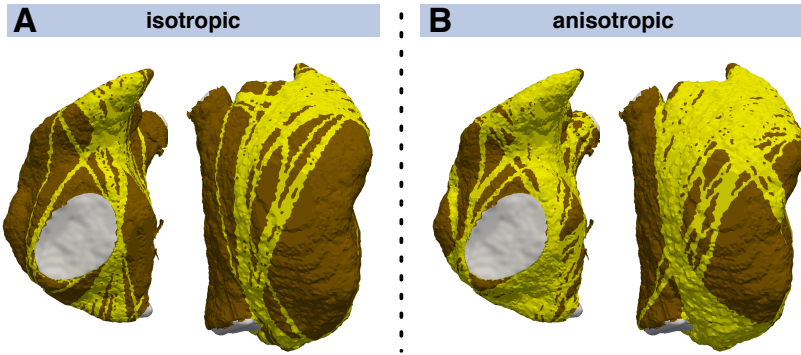
Figure 8.13: Influence of anisotropic conduction on a vulnerability map in the RA. Vulnerable paths are marked in yellow on the brown RA myocardium; the blood pool is indicated in gray. While the latest activation coincided in the isotropic (A) and anisotropic model (B), anisotropy lead to a higher number of vulnerable paths. The heterogeneous CV definitions are detailed in the text.
