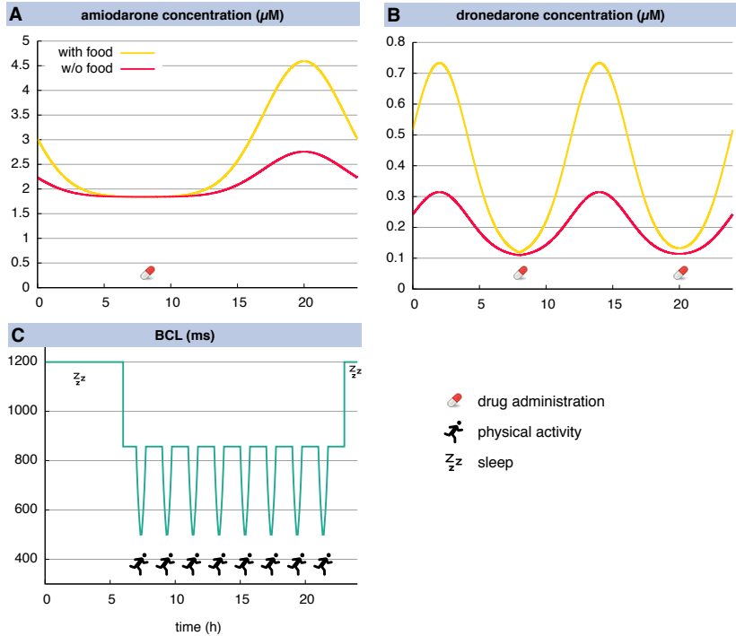
Figure 6.2: Course of the drug concentrations over a typical day modeled in the pharmacokinetic scenarios for amiodarone (A) and dronedarone (B) with and without concomitant food intake, as well as the circadian BCL course including sleep, rest, and phases of physical activity (C).
