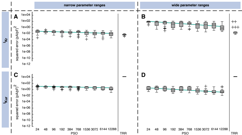
Figure 4.4: Sum of squared errors achieved by pure PSO and pure TRR optimization for synthetic I_{K_r} ((A) and (B)) and I_{K_{ur}} ((C) and (D)) data. The number of particles N for PSO was varied. In (A) and (C), narrow parameter ranges were used whereas in (B) and (D) the search space was wider. Box plots represent 25 experiments each; the green lines indicate linear regressions of the median values in the graph coordinate system.
