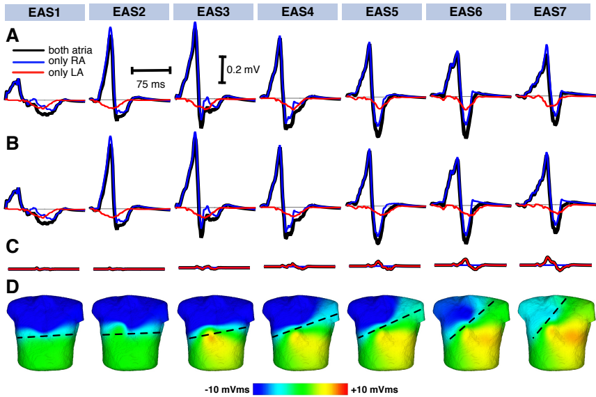
Figure 10.2: P-waves in ECG lead V_1 (A-B) and body surface potential integral maps (D) in model #5 for varying earliest activates sites EAS1 to EAS7 in the RA. The left (red) and blue (right) atrial P-waves add up to the regular P-wave represented by the black traces. The iso-potential line is indicated by a thin grey line. Four IACs were present in (A), whereas the two posterior connections (MPC and LPC) were non-conductive in (B). The difference of ECGs caused by the non-conductive posterior IACs shown in (C) reveals that only the LA P-wave is affected and a more pronounced effect for more inferior EASs. The dashed line in (D) indicates the perceived iso-potential line, which rotates counter-clockwise from EAS1 to EAS7.
