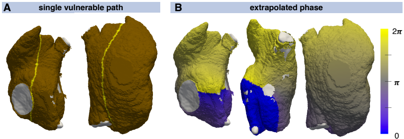
Figure 8.19: Individual vulnerable paths in the RA (A) were extrapolated to the whole RA in phase domain (B) by applying the eikonal-diffusion approach with the path from (A) as a Dirichlet boundary condition.
