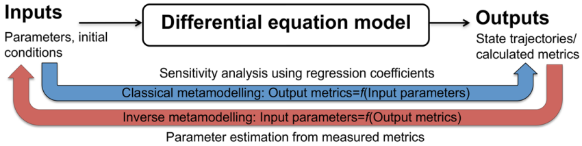
Figure 4.15: Basic concept of classical and inverse metamodelling. Classical (forward) metamodelling predicts the output of the detailed differential equation model using the input parameters aiming at a sensitivity analysis based on the regression coefficients of the metamodel. Inverse metamodelling on the other hand estimates the input parameters based on the output. In this case, the input is composed of the parameters of the detailed model and the output is represented by the measurements. Figure from [213].
