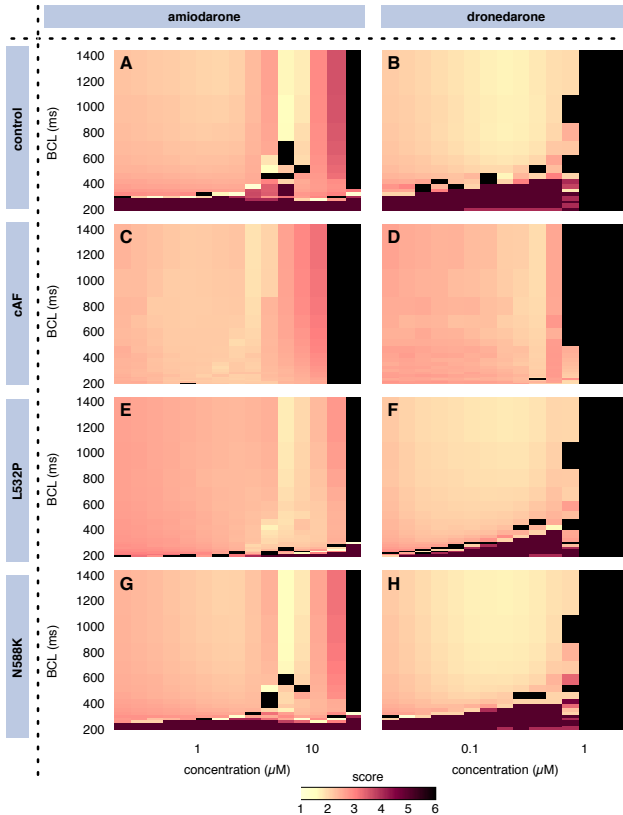
Figure 6.6: Total score resulting from amiodarone (A), (C), (E), and (G) and dronedarone (B), (D), (F), and (H) administration in the four different substrates control (A)+(B), cAF induced remodeling (C)+(D), hERG mutation L532P (E)+(F), and hERG mutation N588K (G)+(H). Scores range from 1 (best) to 6 (worst). The total score is based on the individual scores for AP category (see Figure 6.4), CV, \Delta APD_{90}/\Delta DI , TI, ERP/ERP 0 , APD 50 /APD 50,0 , and VW/VW 0 . In case one of the individual scores of the markers evaluated to 5.5 or worse, or two markers yielded 5.0 or worse, the total score 6 was assigned. Otherwise, the mean of the seven individual scores was considered.
