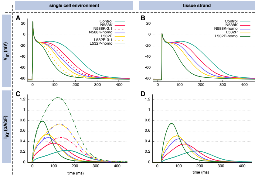
Figure 5.4: APs simulated in the single cell environment (A) and the one-dimensional tissue strand of coupled cells (B) and the corresponding I_{Kr} courses (C) and (D). Dashed lines in (A) represent heterozygous models with 75% mutant channel share. Dash-dotted lines in (C) represent I_{Kr} during AP clamp experiments using the AP of the control model as voltage protocol. The BCL was 1000 ms for all simulation.
