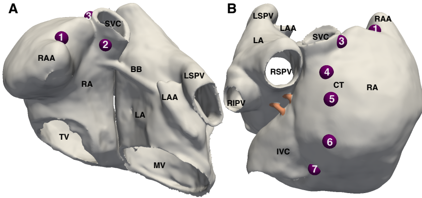
Figure 10.1: Position of the earliest activated sites EAS1 to EAS7 in the RA exemplar visualized on bi-atrial model #5. Anterior view in (A), posterior view in (B). Besides the EAS, RAA, LAA, TV, MV, SVC, IVC, left (L) and right (R), superior (S) and inferior (I) pulmonary veins (PV), CT and BB are indicated for orientation.
