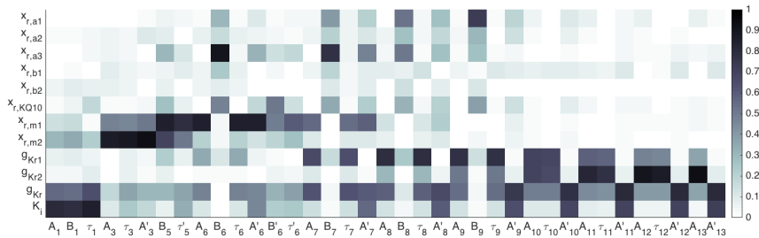
Figure 4.18: Sensitivity of output variables to the parameters of the Courtemanche et al. I_{Kr} formulation and voltage protocol A in terms of regression coefficients. A threshold of 70% of the maximum value selected 37 of the 78 output variables. The subscript of the output variable refers to the voltage trace. A , B , and \tau are the exponential coefficients determined for the first phase of each voltage trace, whereas A' , B' , and \tau' represent the second phase. Output variables were selected based on the cumulated sensitivity with respect to all model parameters.
