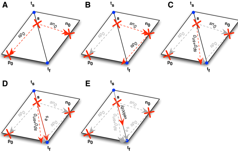
Figure 8.3: Concept of the snaxel velocity calculation for order N=1 and isotropic tissue properties. Snaxel s is connected to its first order neighbors p_0 and n_0 (A). The sum of the connecting vectors s p_0 and s n_0 (B)+(C) is projected onto the supporting edge e_s (D). The projection is scaled by the conduction velocity in order to obtain the velocity of the snaxel (E).
