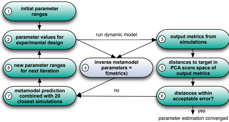
Figure 4.16: Multivariate metamodeling pipeline. After the initial parameter ranges are set in step 1, steps 2-8 are iteratively repeated until the termination criterion in step 6 is met. Step 8 zooms successively into interesting parameter ranges. Figure concept from [213].
