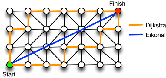
Figure 3.4: Comparison of Dijkstra's algorithm and the solution of the eikonal equation regarding the shortest path between two nodes on a triangular mesh. Dijkstra's algorithm considers only edges of the mesh as segments of the path yielding non-unique results that deviate significantly from the geometrical shortest path between the two nodes. The eikonal approach interpolates activation times considering all adjacent nodes yielding a better result on the same mesh.
