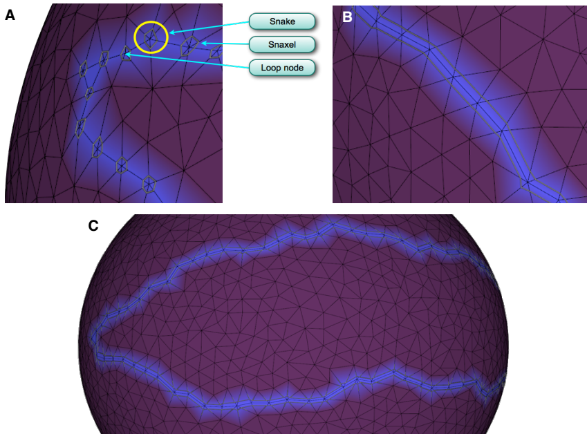
Figure 8.11: Initialization of a geometric snake along a loop (blue band). Initially, a micro-snake is established around each loop node (A). Snake segments are represented by thin grey tubes. Enforcing the constraints regarding the maximum number of snaxels per edge lead to two consistently oriented snakes (B), (C). Only the shorter snake was considered for constriction while the longer one was disregarded.
