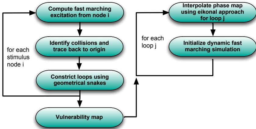
Figure 8.5: Overview of the algorithm to compute vulnerability maps (left) and optionally transfer the AFLut scenarios to dynamic simulations (right).
