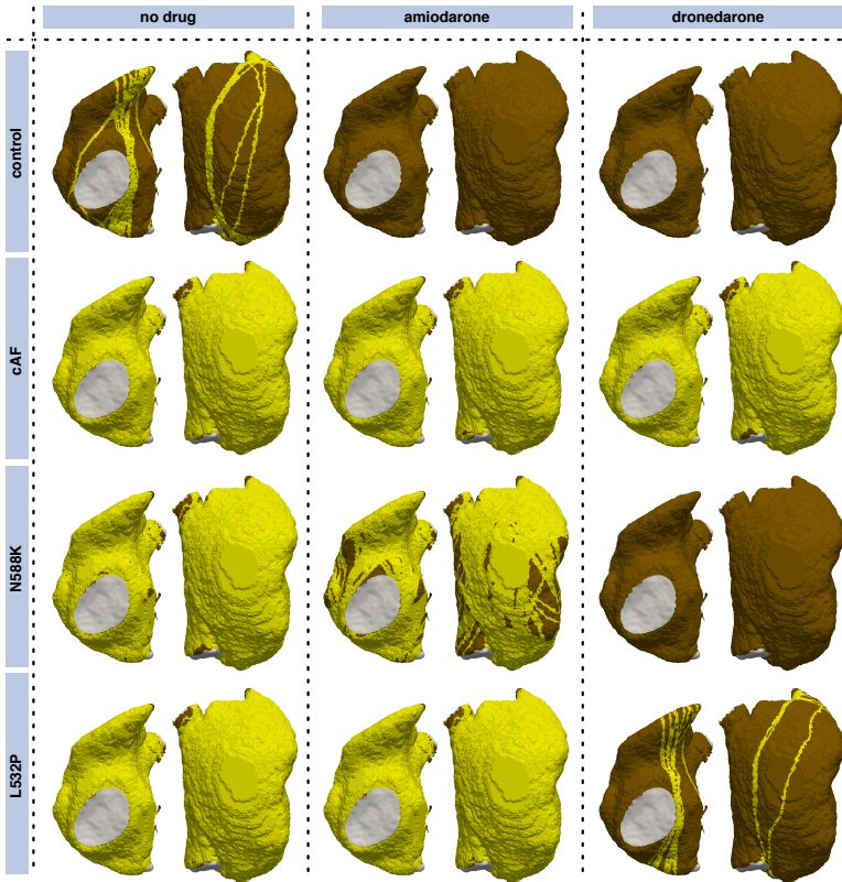
Figure 8.16: Vulnerability maps of the RA for combinations of different substrates and pharmacological agents. In contrast to Figure 8.15, only the ERP was modeled substrate-specific, thus only considering differences in repolarization.
