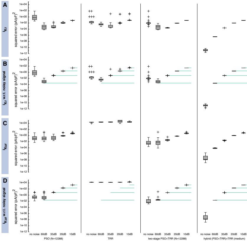
Figure 4.12: Sensitivity of the sum of squared error to noise in synthetic I_{Kr} ((A) and (B)) and I_{Kur} ((C) and (D)) data using pure PSO, pure TRR, two-stage (PSO+TRR) and hybrid (PSO+TRR)+TRR optimization. The squared error was measured with respect to the original, non-noisy data in (A) and (C). In (B) and (D), the error was measured with respect to the noisy data and the horizontal lines indicate the sum of squared differences between the noisy input data and the ground-truth input data. Parameters were restricted to the wide ranges. Box plots represent 25 experiments.
