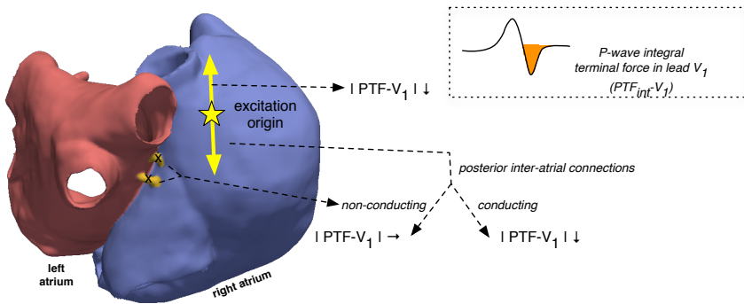
Figure 10.5: In conclusion, the results presented in this chapter show that a shift of the EAS towards both more superior/anterior and more inferior locations causes lower absolute values of PTF-V_1 . If the posterior IACs are non-conductive, a shift towards more inferior locations does not affect PTF-V_1 significantly.
