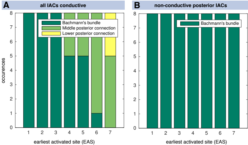
Figure 10.3: Distribution of the IAC conducting the earliest LA breakthrough for varying earliest activated sites EAS1 to EAS7 in the RA in the model population ( n=8 ). In (A), four IACs were present, whereas the two posterior IACs (MPC and LPC) were non-conductive in (B).
