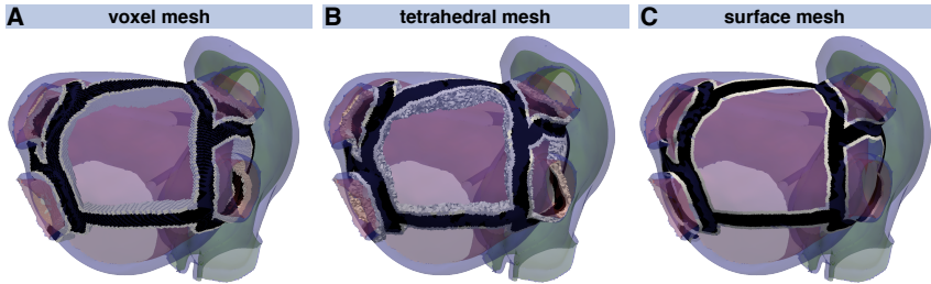
Figure 7.12: Resulting ablation by applying pattern G in model #4. The core lesion with a radius of 2 mm (black) is surrounded by a border zone with a width of 1 mm (white) in the semi-transparent biatrial model. Transmural ablation was applied in the voxel grid (A) and the volumetric tetrahedral mesh (B) revealing the different mesh structures at the interface between the border zone and LA myocardium. In the triangular surface mesh (C), ablation was applied to the epicardial side.
