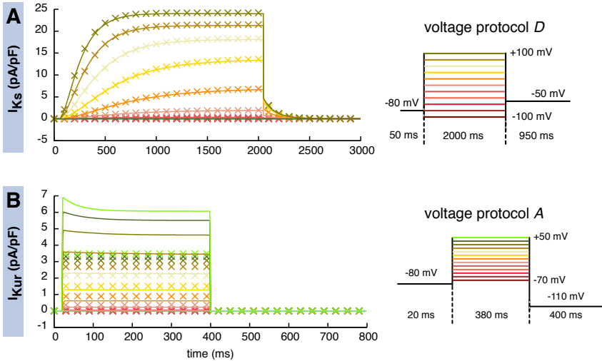
Figure 4.21: Resulting currents using the parameters estimated by the multivariate meta-modeling approach. Solid lines indicate synthetic I_{Ks} (A) and I_{Kur} (B) input currents used for parameter estimation. Crosses represent the best fit obtained (not every sample shown for clarity reasons). The voltage protocols used to generate the input data and to challenge the ion current model are shown on the right part of each panel.
