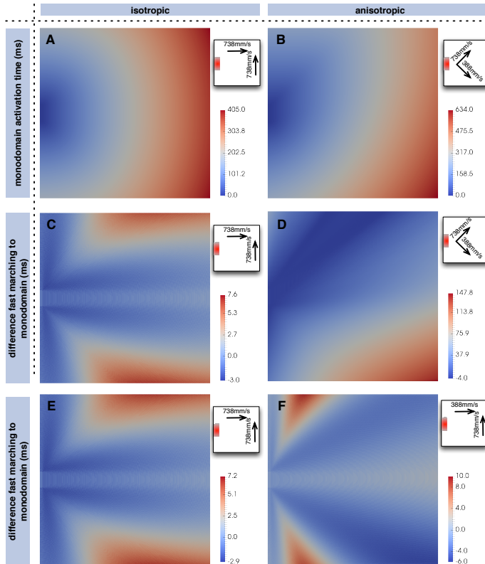
Figure 8.8: Monodomain activation times of almost radial waves in the isotropic (A) and an anisotropic case (B) on quadratic tissue patches with 30 cm side length. Fast marching activation was later for nodes along the diagonal in both ordered (C) and randomly oriented right-angled triangles (E). The deviation was larger for anisotropy 45^\circ to the main triangle orientation axes (D) compared to myocyte orientation aligned with the right angled edges of the triangles (F). Excitation was triggered from the red area in the schematic representation in the top right corner of each panel. Note the different scales of the color bars.
