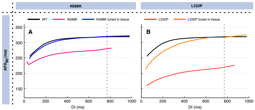
Figure 6.11: Restitution of the APD_{90} for WT and mutant atrial myocytes. The multi-channel blockers (see Table 6.5) were optimized at a BCL of 1000 ms corresponding to the vertical dashed line and applied to the hERG mutant cells at BCLs between 200 ms and 1300 ms.
