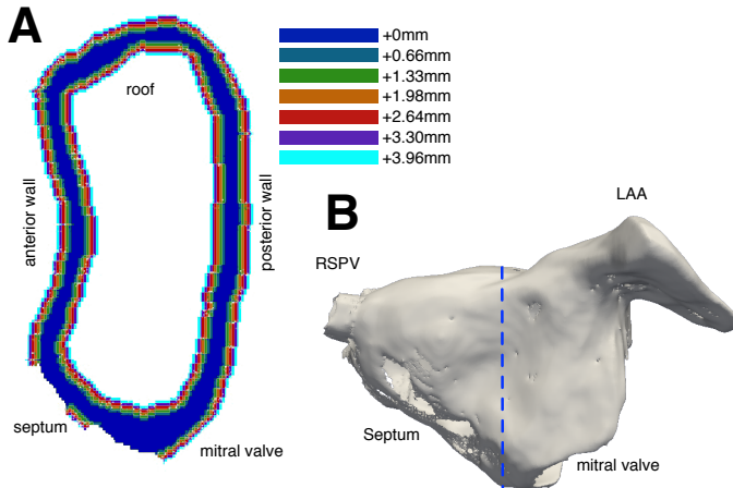
Figure 11.1: Cross section through the LA wall of model #3 with different levels of wall thickening coded by the color (A). The cross section is aligned along the dashed blue line in (B).
