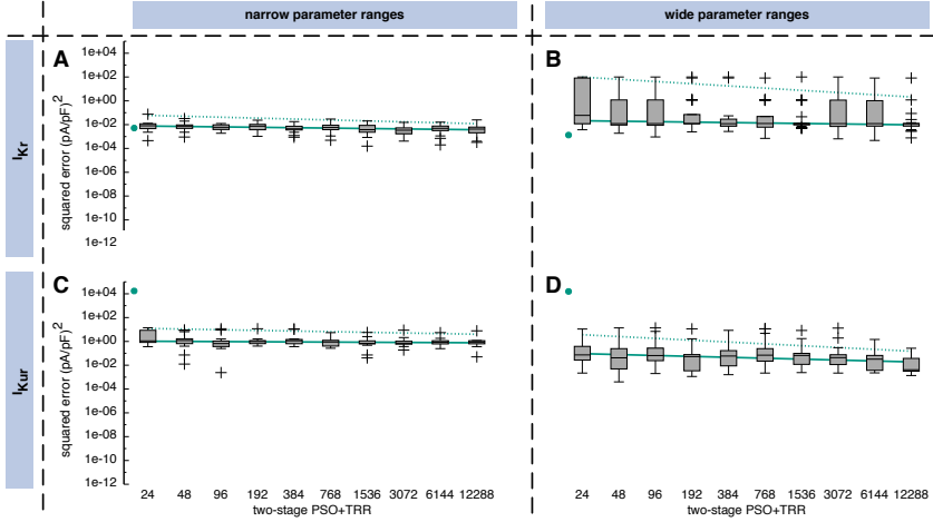
Figure 4.7: Sum of squared errors achieved by two-stage PSO+TRR optimization for synthetic I_{K_r} (A) and (B) and I_{K_{ur}} (C) and (D) data. The number of particles N was varied. In (A) and (C), narrow parameter ranges were used whereas in (B) and (D) the search space was wider. Box plots represent 25 experiments each. The green lines indicate linear regressions of the median values in the graph coordinate system. The green dot on the left of each panel represents the median of pure TRR optimization, the dotted green lines represent linear regressions of the median values of pure PSO (compare Figure 4.4).
