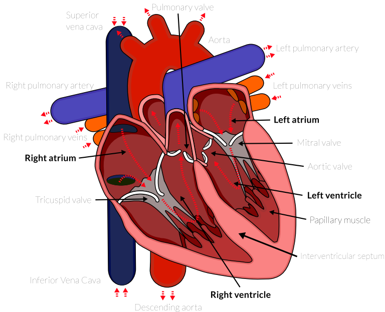
Figure 2.1: The human heart and the great vessels. Blood flow is indicated by dashed red arrows. Reproduced from [15] with permission.
