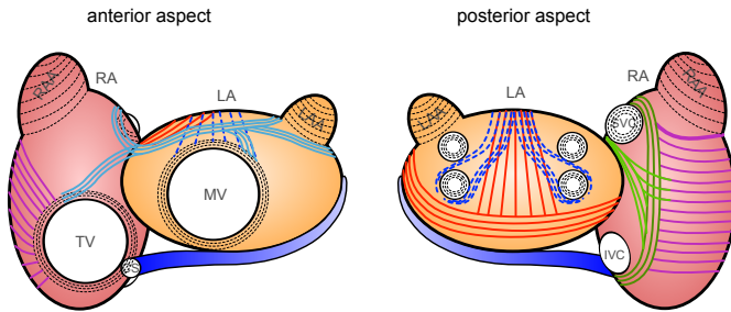
Figure 2.2: Schematic representation of the major muscular bundles in the atria. Blue: septo-atrial bundle in the subendocardium, red: septo-pulmonary bundle in the subepicardium, light blue: BB, green: CT, pink: PMs, black: circular myocyte orientation around the appendages, as well as vessel and valve orifices, blue CS. Reproduced from [23] with permission.
