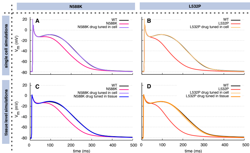
Figure 6.10: AP curves from single cell (A)+(B) and tissue level (C)+(D) simulations obtained using WT and hERG mutation cell models. The optimized multi-channel blockers given in Table 6.5 were applied to mutant myocytes to restore the WT AP. In (A) and (B), the WT APs are partly covered by those of the mutant models under drug influence. In (C) and (D), the APs obtained by tissue level optimization partly cover the single cell optimization result, additionally.
