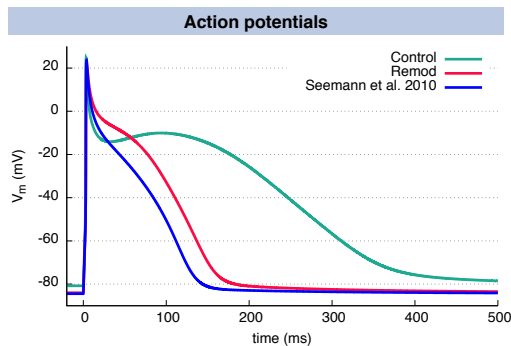
Figure 5.8: AP of an atrial myocyte under cAF remodeling conditions (red) in comparison to control (green). The blue curve represents the setup by Seemann et al. [291].
