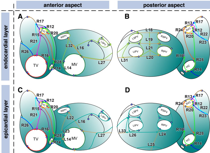
Figure 7.2: Schematic course of the paths along which myocyte orientation was annotated. In the LA, the paths in the endocardial layer ((A) and (B)) and the epicardial layer ((C) and (D)) were annotated using two distinct set of rules, whereas the paths did not differ between layers in the RA. Different colors represent distinct tissue classes. Blue points represent the 22 initial landmarks. Dashed lines were only used to compute the location of auxiliary points and not used to align myocyte orientation. (A) and (C) show the anterior aspect, (B) and (D) the posterior aspect. Figure based on supervised student’s work [388].
