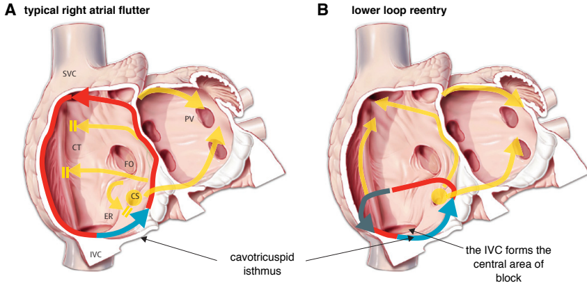
Figure 2.5: Paths maintaining AFlut in the RA (red arrows). Flutter is sustained along the TV annulus in typical flutter (A). Both atrioventricular annuli have been removed for clearer visualization. The blue arrow indicates the cavotricuspid isthmus representing the crucial narrowest part in typical AFlut (A) and lower loop reentry (B). Yellow arrows indicate pathways activating the atrial myocardium but not driving the flutter. The dark gray arrow in (B) indicates a zone of slow conduction allowing to sustain the flutter along the shorter circuit compared to (A) where the CT forms a line of functional block in transverse direction. Reproduced from [62] with permission from the publisher.
