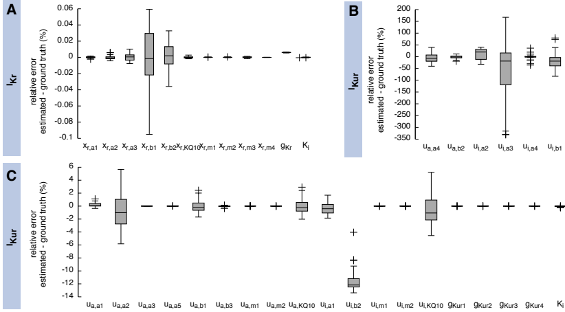
Figure 4.11: Relative error of the estimated parameters using synthetic I_{Kr} (A) and I_{Kur} (B)+(C) data and the hybrid (PSO+TRR)+TRR approach in the high configuration. Parameter deviations were normalized to their ground truth values. Note the different scales. I_{Kur} parameters were split in high deviation (B) and low deviation (C) groups. Box plots represent 25 experiments.
