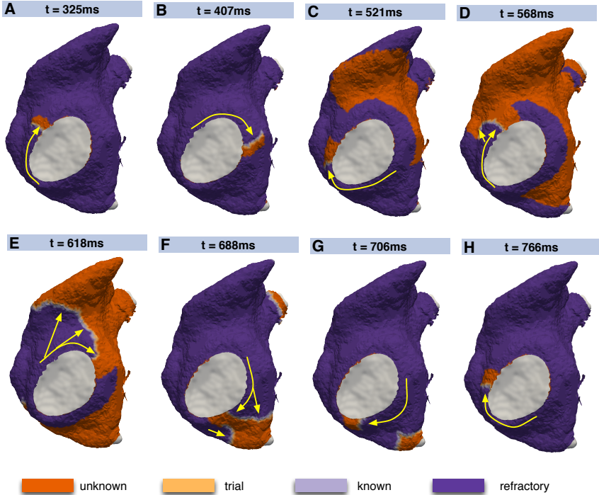
Figure 8.20: Dynamic fast marching simulation with AFLut around the TV. Every second cycle, tissue towards the RAA was non-refractory (D) and excited by the dominant flutter path (E). Wavefronts collided in the CS region (F) such that only the dominant flutter path around the TV was still active and driving reentry (H). The blood pool is indicated in gray.
