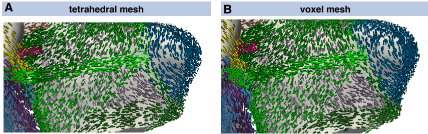
Figure 7.5: Close up of the annotated myocyte orientation in the BB region in model #4 represented by cylinders superimposed on the smoothed blood pool shown in grey. The two-layer architecture is clearly visible. Endocardial orientation cylinders are shown in grey while the epicardial ones are colored in green. The tissue class labels in both the tetrahedral mesh (A) and the structured voxel grid (B) are encoded by color. Figure based on supervised student’s work [388].
