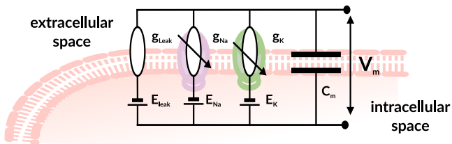
Figure 3.1: Equivalent electric circuit of a giant squid axon according to Hodgkin and Huxley [152]. Under physiological conditions, the Nernst potential for potassium is negative whereas those for sodium and leak are positive. Adapted from [15] with permission.
