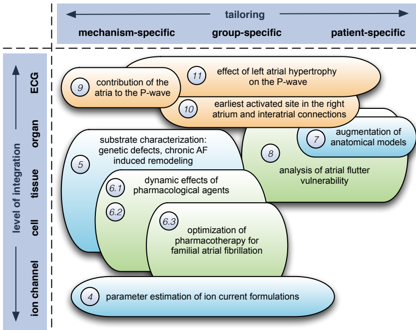
Figure 12.1: Classification of the projects presented in this thesis regarding the level of integration and regarding the type of tailored therapy benefiting from the results. Colors indicate the area of improvement: diagnosis (orange), model development and comprehension of pathomechanisms (blue), and atrial fibrillation therapy (green). Numbers refer to the corresponding chapters of this thesis.
