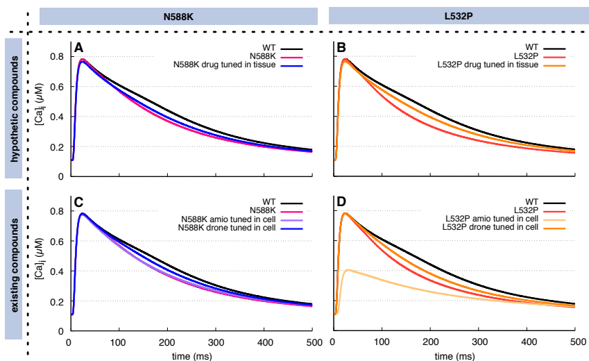
Figure 6.12: Calcium transients observed during APs in the N588K (A)+(C) and L532P (B)+(D) hERG mutant cells. In (A) and (B), the optimized hypothetical multi-channel blockers were administered, whereas amiodarone and dronedarone were administered at optimized concentrations in (C)+(D).
