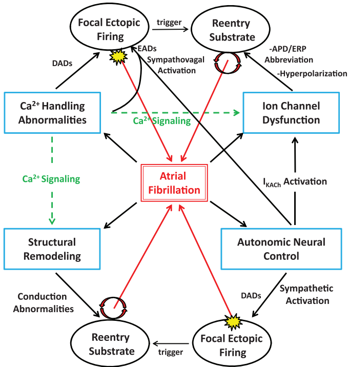
Figure 2.7: Mechanisms contributing to the initiation and perpetuation of AF by affecting the arrhythmia-initiating trigger and the arrhythmia-sustaining substrate. Abbreviations: delayed afterdepolarization (DAD), early afterdepolarization (EAD), action potential duration (APD), effective refractory phase (ERP). Reproduced from [72] with permission from the publisher.
