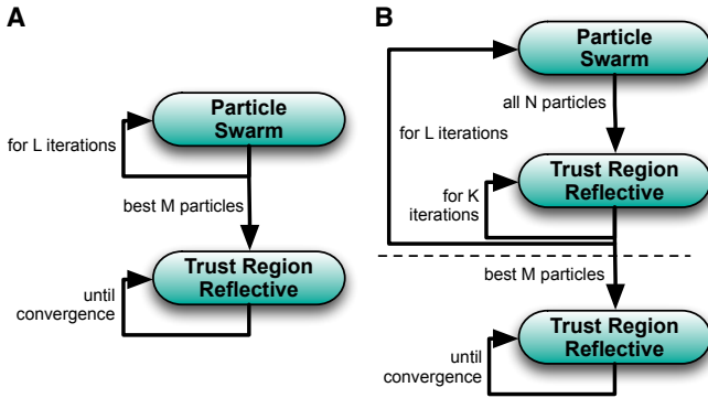
Figure 4.3: Flow chart of the two-stage PSO+TRR algorithm (A) and the hybrid (PSO+TRR)+TRR algorithm (B). The steps above the horizontal, dashed line in (B) are referred to as hybrid (PSO+TRR) .
