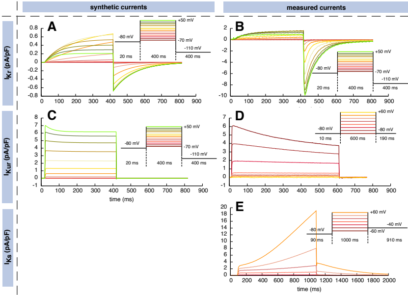
Figure 4.1: Synthetic ((A) and (C)) and measured ((B), (D), and (E)) input current data used to estimate parameters together with the corresponding voltage protocols. (A) and (B) show I_{Kr} , (C) and (D) show I_{Kur} , (E) shows I_{Ks} .
