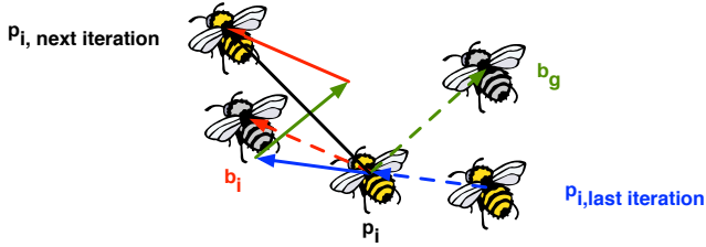
Figure 4.2: Basic principle of the PSO. Each particle with its position \mathbf{p}_i experiences attracting forces towards the best position found so far by the entire swarm \mathbf{b}_g , the best position found so far by itself \mathbf{b}_i , and an inertia force defined by the difference between the current position \mathbf{p}_i and the one in the last iteration \mathbf{p}_{i, \text{last iteration}} . These three forces are weighted using uniformly distributed numbers \in [0,1] and added vectorially to obtain the position for the next iteration ( \mathbf{p}_{i, \text{next iteration}} ).
