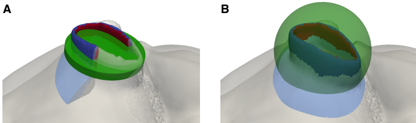
Figure 7.3: Annotation of the PVs. If non-labeled tissue (blue) was found within the green cylinder in (A), an outwards-oriented PV was assumed to be present. The PV was cut open for visualization reasons within the semi-transparent LA wall in (A) but not in (B). All elements within the green sphere in (B) were labeled as PV tissue. Figure based on supervised student's work [388].
