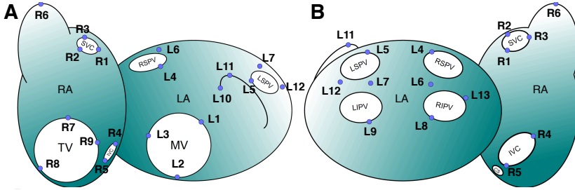
Figure 7.1: Schematic representation of the 22 landmark points (blue) given in Table 7.1. R1 to R9 are located in the RA, L1 to L13 are located in the LA. (A) shows the anterior aspect, (B) the posterior aspect. Figure based on supervised student's work [388].
