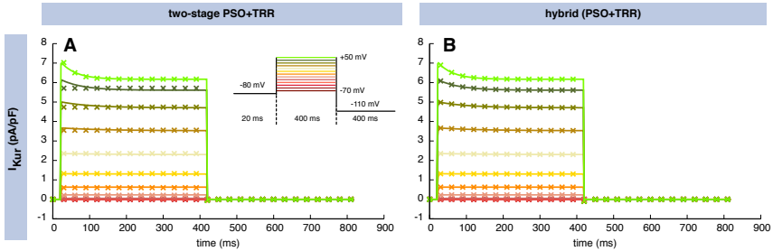
Figure 4.14: Resulting I_{Kur} curves using the parameters estimated by the two-stage PSO+TRR (A) and the hybrid (PSO+TRR) approach in the medium setup (B) together with the corresponding voltage protocols. Solid lines indicate synthetic input currents used for parameter estimation. Crosses represent the worst fit obtained using the respective approach and the wide parameter ranges (every 15 th sample is shown). Differences are most pronounced for step voltages between +20 mV and +40 mV.
