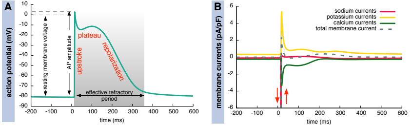
Figure 2.4: The course of the transmembrane voltage V_m during a cardiac action potential with its different phases (A) and the membrane currents carried by the different ions (B). The sodium current reaches an amplitude of \approx -70 pA/pF. The calcium exchange with the sarcoplasmic reticulum is not considered. Courses were computed using the Courtemanche et al. model [49]. Figure inspired by [50].
