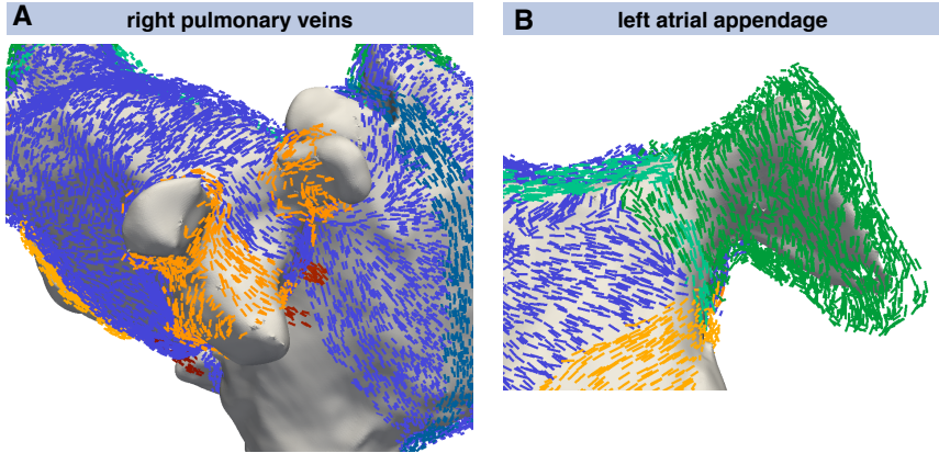
Figure 7.7: Close up of the annotated myocyte orientation in the RPV (A) and LAA (B) region of model #3. The color of the lines aligned with myocyte orientation encodes the annotated tissue class. The smoothed endocardial surface is shown in grey. The two RIPVs were annotated together (A). The L-shaped LAA was completely labeled with the right tissue class and myocyte orientation was modeled approximately circumferential.
