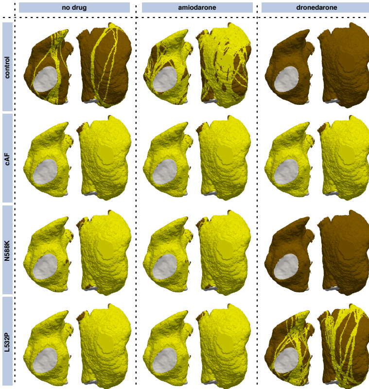
Figure 8.15: Vulnerability maps of the RA for combinations of different substrates and pharmacological agents. Besides a control substrate representing healthy myocytes, a cAF remodeled substrate (neglecting changes of cell-to-cell coupling), and two hERG mutations were evaluated. Standard concentrations of the antiarrhythmic agents amiodarone ( 2.3 \mu\text{M} ) and dronedaron ( 0.21 \mu\text{M} ) were administered in the center and right columns. Vulnerable paths are marked in yellow on the brown RA myocardium; the blood pool is indicated in gray.
