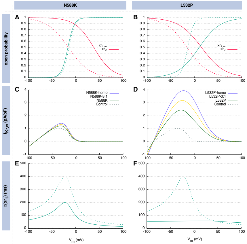
Figure 5.3: Voltage dependency of gate open probabilities of the homozygous mutant model (A)+(B), dashed lines represent the control model. The x_{r1} gate is the classical ODE gate defined by Equation (A.3) to Equation (A.6), while x_{r2} is the instantaneous gate defined in Equation (A.2). Steady-state I_{K_r} of the homozygous and heterozygous mutant models (C)+(D), and time constant \tau of the x_{r1} gate of the homozygous model (E)+(F).
