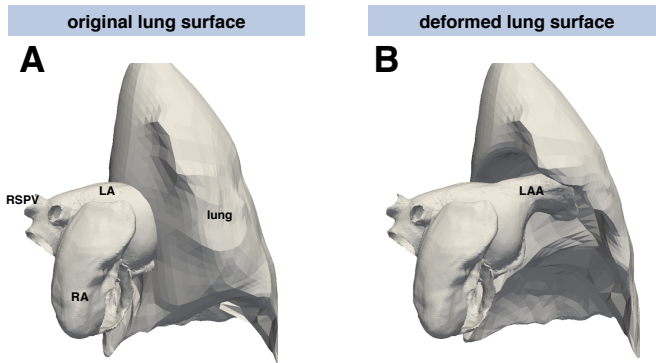
Figure 11.3: The dilated LA intersects with the lobes of the left lung as segmented using the imaging data (A). Therefore, the volume of the left lung was manually reduced to make room for the dilated LA (B). Figure modified from [549].
