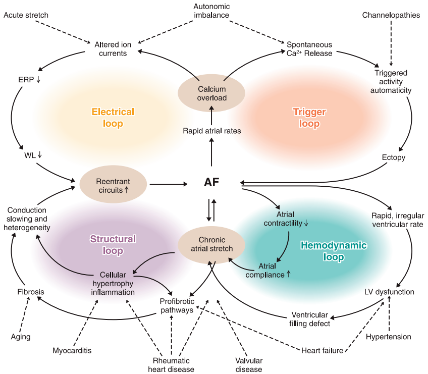
Figure 2.9: Overview of the main driving forces of AF and AF-induced remodeling. Four positive-feedback loops cause the remodeling process. Reproduced from [77] with permission from the publisher.
