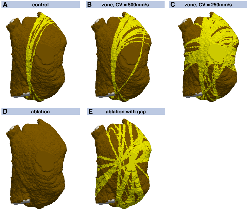
Figure 8.18: Vulnerability maps of the RA for different substrate modifications. Compared, to (A), a zone of slow conduction was assumed (cf. Figure 8.17A) in (B)+(C). A circular ablation lesion was introduced in (D) (cf. Figure 8.17B). In (E), a gap in the ablation lesion was modeled on the central posterior wall (cf. Figure 8.17C).
