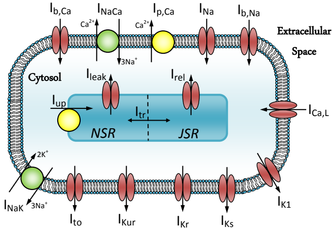
Figure 3.2: Schematic representation of the Courtemanche et al. model of human atrial myocytes [49]. Ion channels (red), pumps (green), and transporters (yellow) allow the exchange of ions between the intracellular space (cytosol), the extracellular space and the calcium subspaces (NSR and JSR). Reproduced from [155] with permission.
