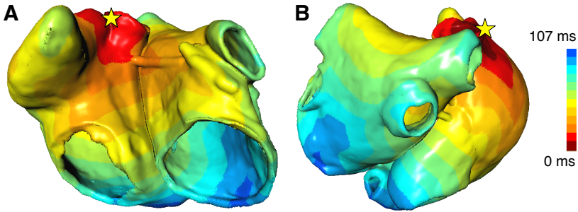
Figure 9.1: Local activation times resulting from the excitation propagation simulation using model #5. Excitation originated from the junction of the SVC and the RAA indicated by the yellow star. Anterior view in (A), posterior view in (B).
