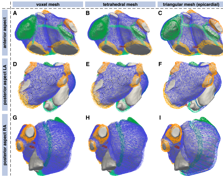
Figure 7.4: Annotated myocyte orientation in a volumetric voxel mesh ((A), (D), and (G)), a tetrahedral mesh ((B), (E), and (H)), as well as a triangular mesh of the epicardial surface ((C), (F), and (I)) of model #5. The color of the lines aligned with myocyte orientation encodes the annotated tissue class. The smoothed endocardial surface is shown in grey. The distinct endocardial and epicardial two layer architecture can e.g. be seen in the posterior wall region and at the junction with the inferior PVs in (D) and (E) (dashed circles). In (F), no crossing fibers are present as only the epicardial layer is present. The orientation along the IACs introduced in Section 7.2 are already annotated in green (BB) and red (remaining IACs).
