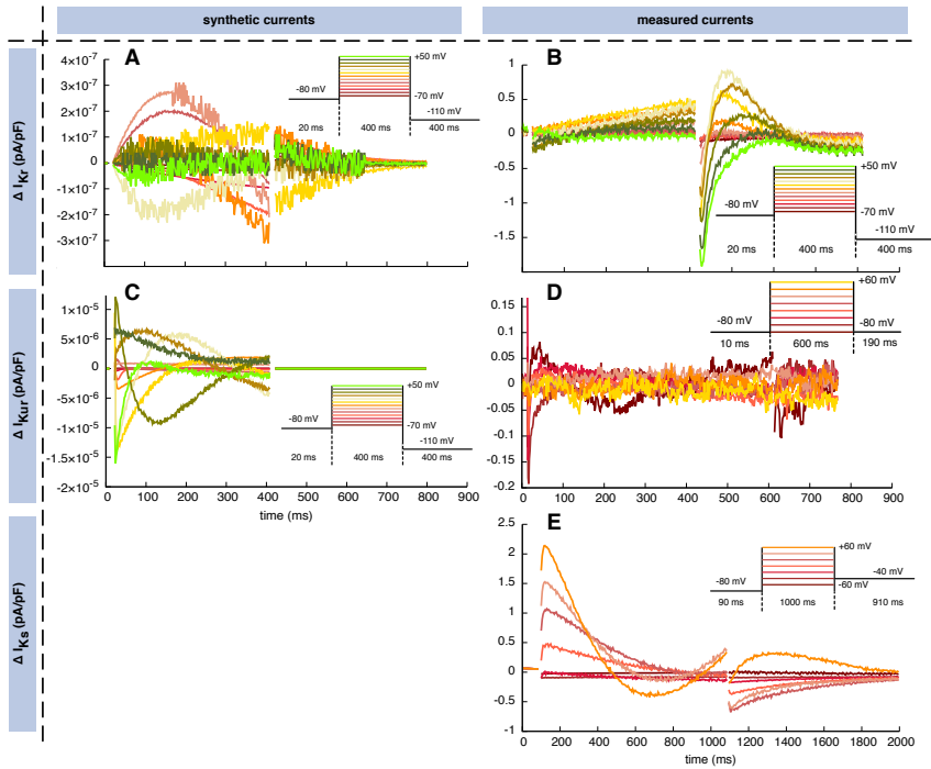
Figure 4.10: Resulting difference between the input currents and the model output using the estimated parameters. The best fit obtained using the high setup of the hybrid (PSO+TRR)+TRR approach is shown. Samples directly adjacent to voltage steps were ignored in the cost function for the optimization and not plotted. (A) and (B) show I_{Kr} , (C) and (D) show I_{Kur} , (E) shows I_{Ks} together with the corresponding voltage protocols.
