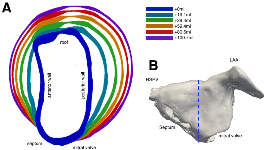
Figure 11.2: Cross section through the LA wall of model #3 with different levels of dilation coded by the color and induced by pressure overload (A). The cross section is aligned along the dashed blue line in (B).
