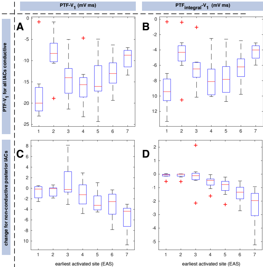
Figure 10.4: P-wave terminal force (PTF- V_1 , (A+C)) and P-wave integral terminal force (PTF integral - V_1 , (B+D)) for varying earliest activated sites EAS1 to EAS7 in the RA. In (A+B), four IACs were present, (C+D) show the difference when the two posterior connections were non-conductive. Note the different scales of the panels.
