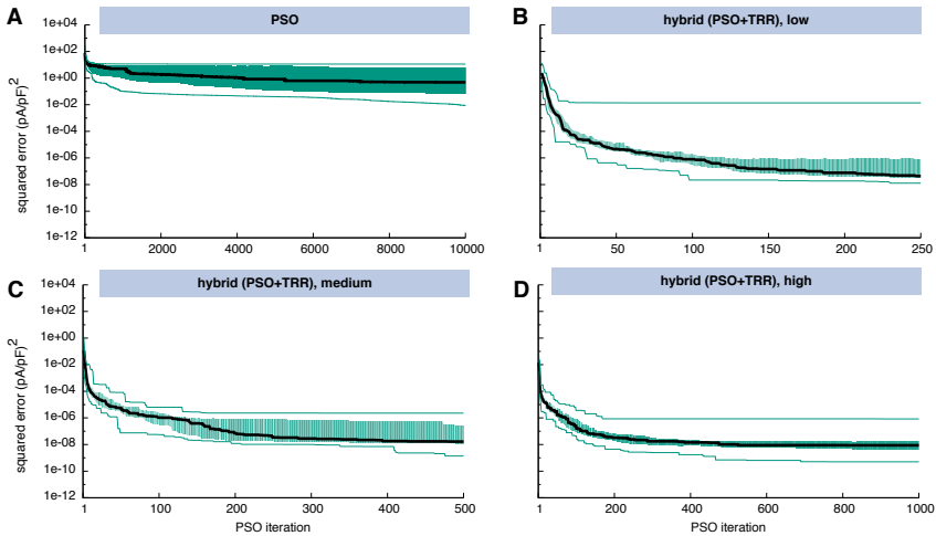
Figure 4.6: Sum of squared errors convergence behavior of pure PSO (A) and hybrid (PSO+TRR) (B-D) for synthetic I_{Kur} data. 25 experiments using the wide parameter ranges were performed. The black line indicates the median, the green lines the minimum and the maximum. The green area covers the two central quartiles. The number of particles N , the number of PSO iterations L , and the number of inner TRR iterations K was increased from low (B) via medium (C) to high (D).
