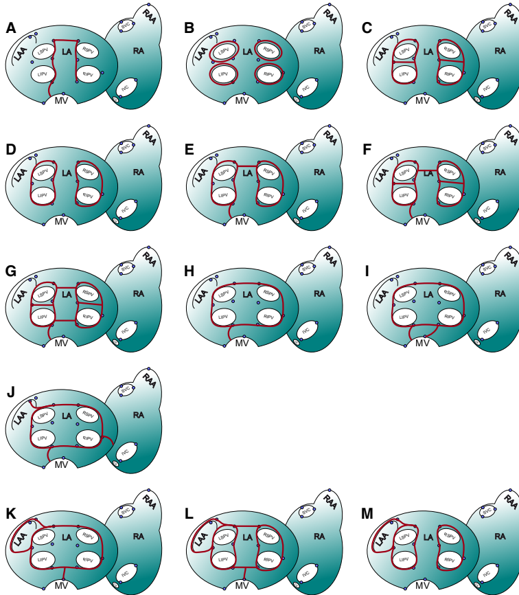
Figure 7.11: Schematic representation of the standardized ablation patterns provided by the automatic algorithm and defined in Table 7.7. Patterns A to J are based on [411], patterns K to M are based on [412]. Figure based on supervised student's work [388].
