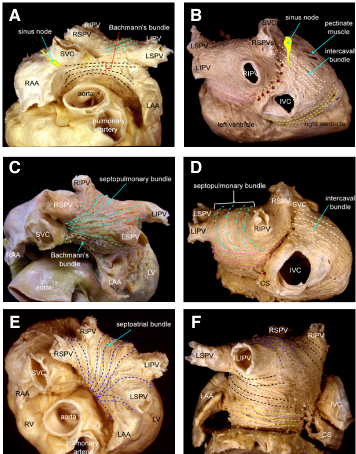
Figure 2.3: Major muscular bundles in the atria indicated by dashed lines overlaid on photographs of human atrial dissections. Stars indicate bundles bridging the interatrial groove. Reproduced from [23] with permission.
