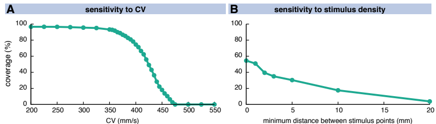
Figure 8.14: Sensitivity of the vulnerable paths to changes of the CV (A) and the stimulus point density (B). The CV was altered in a homogeneous, isotropic setup causing different degrees of RA coverage by vulnerable paths for a fixed stimulus density of 1 mm. In (B), the distance between stimulus points was varied for a fixed CV of 425 mm/s.
