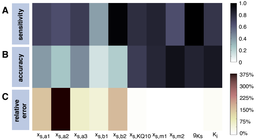
Figure 4.22: Maximum sensitivity (regression coefficients) across the 66 output variables to the parameters of the Courtemanche et al. I_{Ks} formulation (A) as well as parameter prediction accuracy ( R^2 ) in (B) using voltage protocol D (see Figure 4.21A). (C) shows the absolute value of the relative error between the estimated and the ground truth parameters for the results yielded by the look up function.
