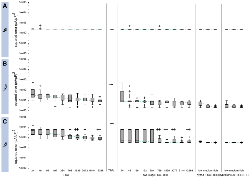
Figure 4.13: Sum of squared errors achieved by pure PSO or TRR, two-stage PSO+TRR , hybrid (PSO+TRR) and hybrid (PSO+TRR)+TRR optimization for measured I_{K_r} (A), I_{K_{ur}} (B) and I_{K_s} (C) data. Parameter values were restricted to the wide range. Note the different scaling compared to Figure 4.4, Figure 4.7, and Figure 4.8. For the one-stage and two-stage PSO approaches the number of particles N was varied. For the hybrid approaches, the number of particles N , the number of PSO iterations L and the number of inner TRR iterations K was increased from low via medium to high . Box plots represent 25 experiments each; the dashed lines indicate linear regressions of the median values in the graph coordinate system.
