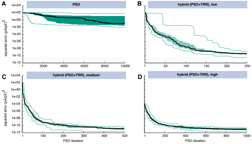
Figure 4.5: Sum of squared errors convergence behavior of pure PSO (A) and hybrid (PSO+TRR) (B-D) for synthetic I_{Kr} data. 25 experiments using the wide parameter ranges were performed. The black line indicates the median, the green lines the minimum and the maximum. The green area covers the two central quartiles. The number of particles N , the number of PSO iterations L , and the number of inner TRR iterations K was increased from low (B) via medium (C) to high (D).
