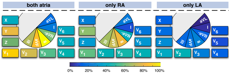
Figure 9.5: Projection intensity of the combined and separated simulated P-waves onto the different ECG and VCG leads. The color encodes the median ( n=8 ) integral of absolute values (P-wave area), which were normalized to the maximum lead in the regular P-wave for each model ( V_1 for #5, II for all other models). Values for the LA and the RA add up to the value for both atria.
