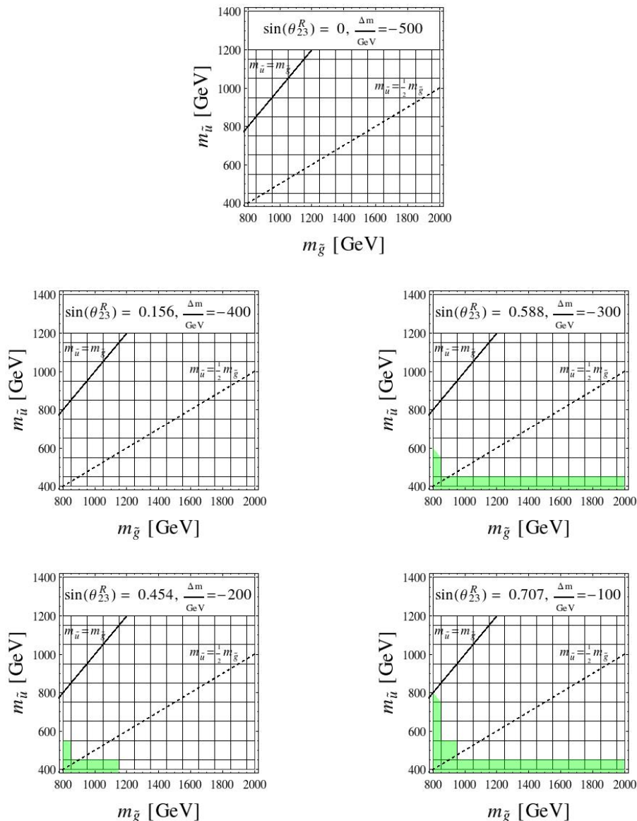
Figure 7. Sensitivity of the ATLAS charm-squark search of ref. [41] for different values of the \Delta m and \theta_{23}^R parameters (the exact values being indicated in the top bar of each subfigure). The excluded regions are shown in green in the (m_{\tilde{u}}, m_{\tilde{g}}) plane, where m_{\tilde{u}} is the mass of the lightest squark (a stop-like squark here since \Delta m < 0 ). The upper panel describes the reference scenario in which the lightest squark is a pure stop state and the scharm is almost decoupled.
