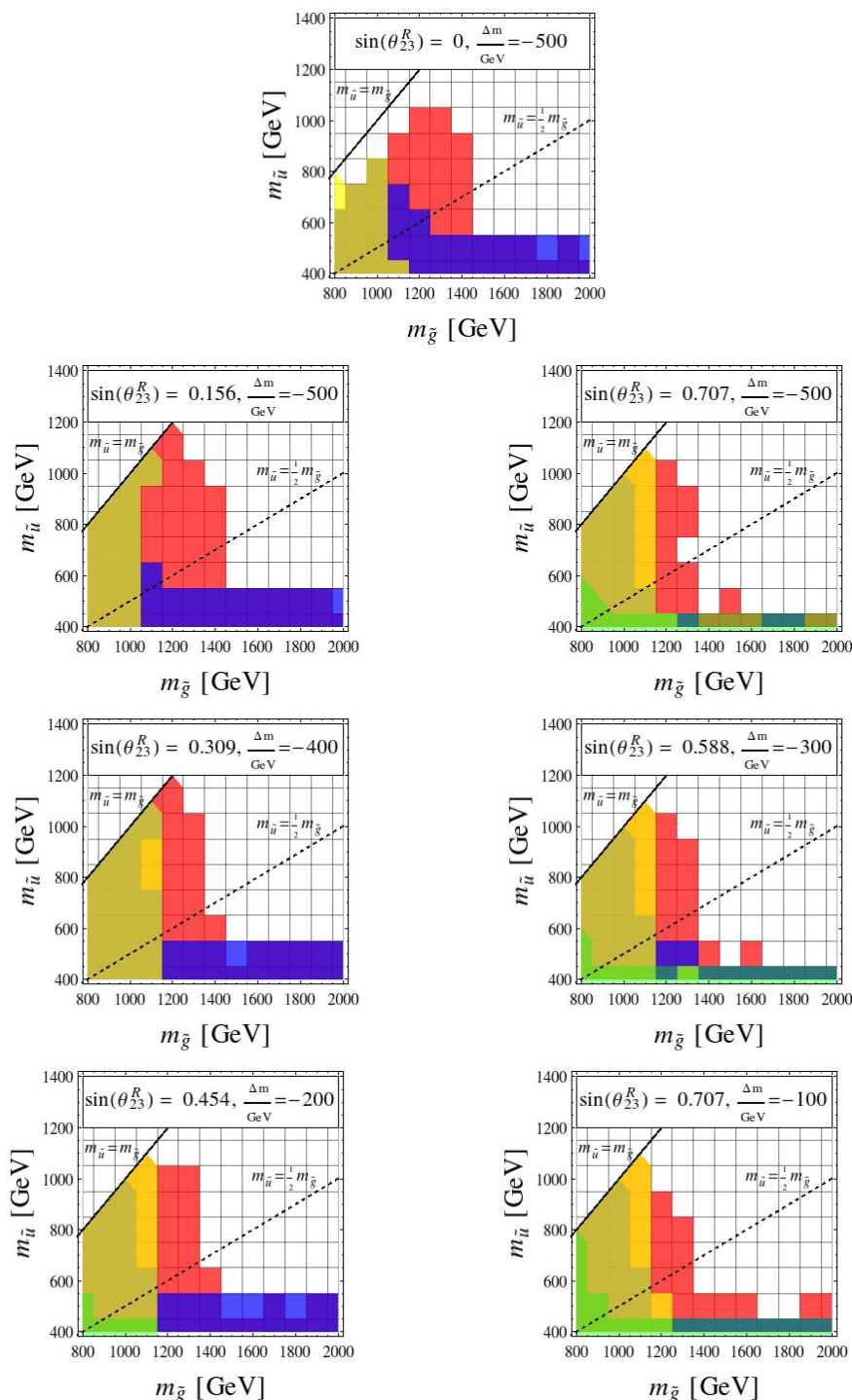
Figure 9. Sensitivity of all four searches pursued in this work for different values of the \Delta m and \theta_{23}^R parameters (the exact values being indicated in the top bar of each subfigure). The excluded regions related to the ATLAS-SUSY-2013-04, CMS-SUS-13-011, CMS-SUS-13-012 and ATLAS-SUSY-2014-03 are respectively shown in red, blue, yellow and green in the (m_{\tilde{u}}, m_{\tilde{g}}) plane, where m_{\tilde{u}} is the mass of the lightest squark (a stop-like squark here since \Delta m < 0 ). The upper panel describes the reference scenario in which the lightest squark is a pure stop state and the scharm is almost decoupled.
