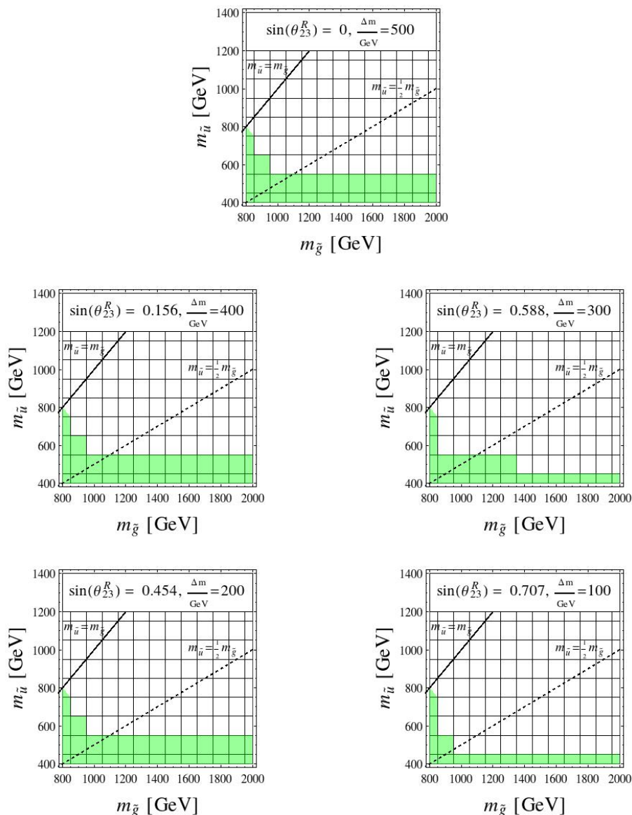
Figure 8. Sensitivity of the ATLAS charm-squark search of ref. [41] for different values of the \Delta m and \theta_{23}^R parameters (the exact values being indicated in the top bar of each subfigure). The excluded regions are shown in green in the (m_{\tilde{u}}, m_{\tilde{g}}) plane, where m_{\tilde{u}} is the mass of the lightest squark (a scharm-like squark here since \Delta m > 0 ). The upper panel describes the reference scenario in which the lightest squark is a pure scharm state and the stop is almost decoupled.
