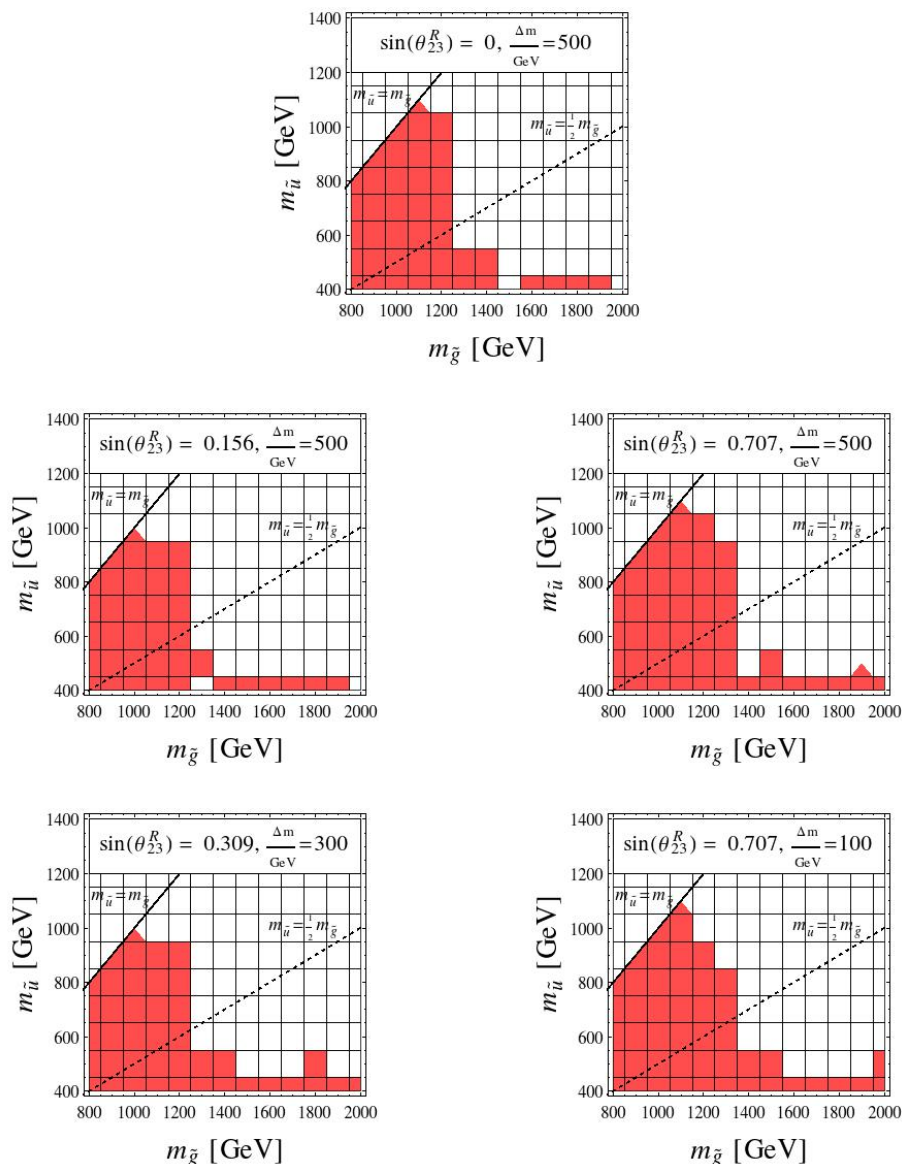
Figure 2. Sensitivity of the ATLAS multijet + \cancel{E}_T + lepton veto search of ref. [39] for different values of the \Delta m and \theta_{23}^R parameters (the exact values being indicated in the top bar of each subfigure). The excluded regions are shown in red in the (m_{\tilde{u}}, m_{\tilde{g}}) plane, where m_{\tilde{u}} is the mass of the lightest squark (a scharm-like squark here since \Delta m > 0 ). The upper panel describes the reference scenario in which the lightest squark is a pure scharm state and the stop is almost decoupled.
