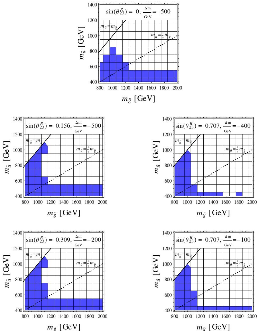
Figure 3. Sensitivity of the CMS stop search in the single lepton mode of ref. [38] for different values of the \Delta m and \theta_{23}^R parameters (the exact values being indicated in the top bar of each subfigure). The excluded regions are shown in blue in the (m_{\tilde{u}}, m_{\tilde{g}}) plane, where m_{\tilde{u}} is the mass of the lightest squark (a stop-like squark here since \Delta m < 0 ). The upper panel describes the reference scenario in which the lightest squark is a pure stop state and the scharm is almost decoupled.
