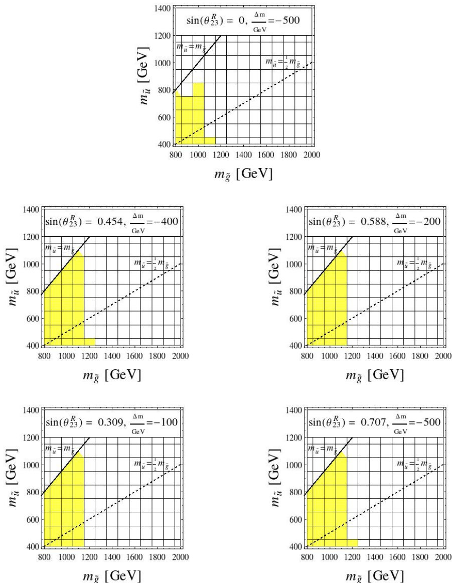
Figure 5. Sensitivity of the CMS supersymmetry search in the multijet plus missing energy channel of ref. [40] for different values of the \Delta m and \theta_{23}^R parameters (the exact values being indicated in the top bar of each subfigure). The excluded regions are shown in yellow in the (m_{\tilde{u}}, m_{\tilde{g}}) plane, where m_{\tilde{u}} is the mass of the lightest squark (a stop-like squark here since \Delta m < 0 ). The upper panel describes the reference scenario in which the lightest squark is a pure stop state and the scharm is almost decoupled.
