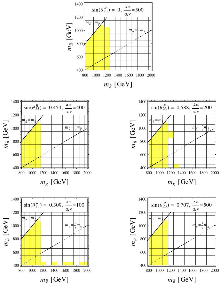
Figure 6. Sensitivity of the CMS supersymmetry search in the multijet plus missing energy channel of ref. [40] for different values of the \Delta m and \theta_{23}^R parameters (the exact values being indicated in the top bar of each subfigure). The excluded regions are shown in yellow in the (m_{\tilde{u}}, m_{\tilde{g}}) plane, where m_{\tilde{u}} is the mass of the lightest squark (a scharm-like squark here since \Delta m > 0 ). The upper panel describes the reference scenario in which the lightest squark is a pure scharm state and the stop is almost decoupled.
