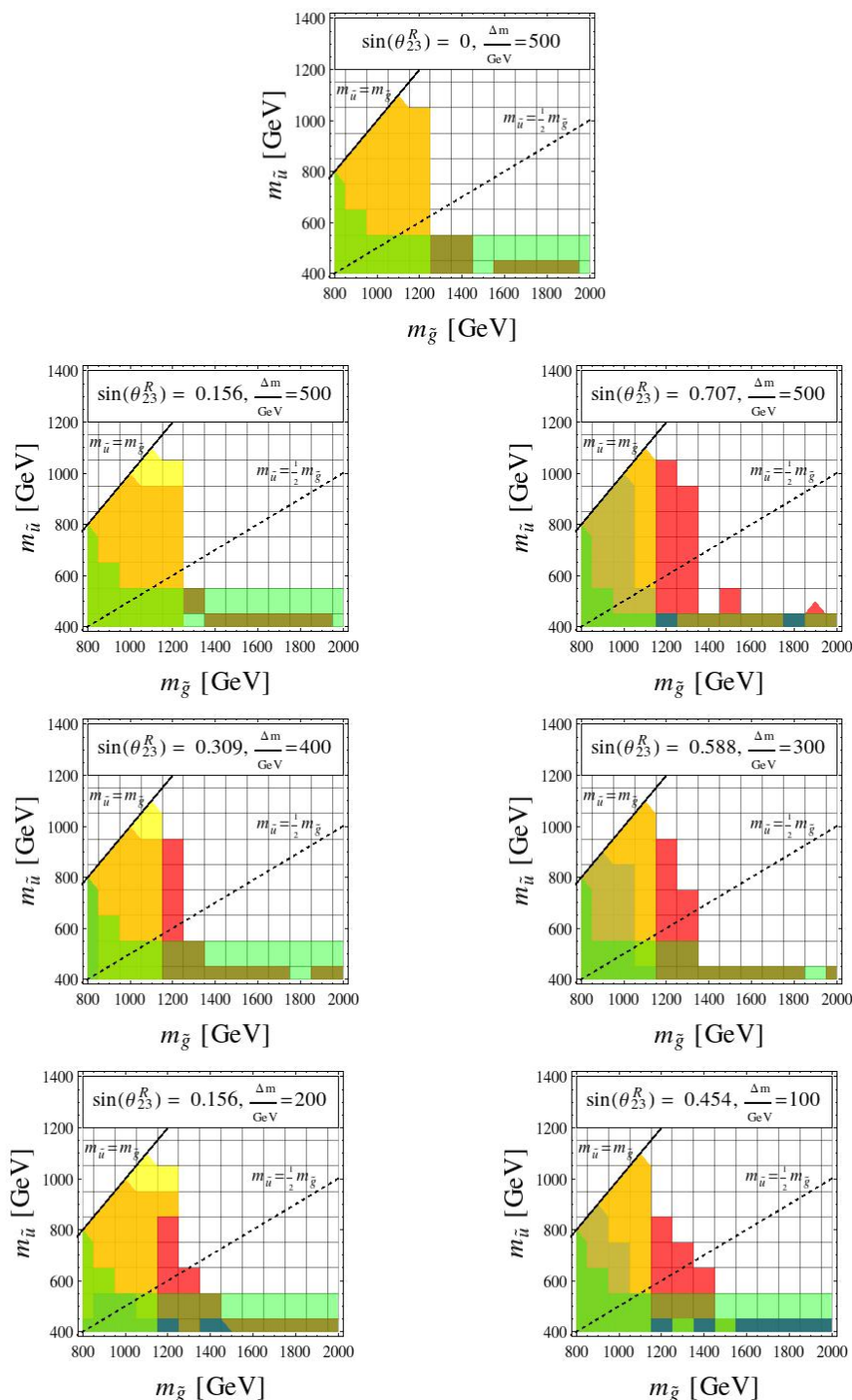
Figure 10. Sensitivity of all four searches pursued in this work for different values of the \Delta m and \theta_{23}^R parameters (the exact values being indicated in the top bar of each subfigure). The excluded regions related to the ATLAS-SUSY-2013-04, CMS-SUS-13-011, CMS-SUS-13-012 and ATLAS-SUSY-2014-03 are respectively shown in red, blue, yellow and green in the (m_{\tilde{u}}, m_{\tilde{g}}) plane, where m_{\tilde{u}} is the mass of the lightest squark (a scharm-like squark here since \Delta m > 0 ). The upper panel describes the reference scenario in which the lightest squark is a pure scharm state and the stop is almost decoupled.
