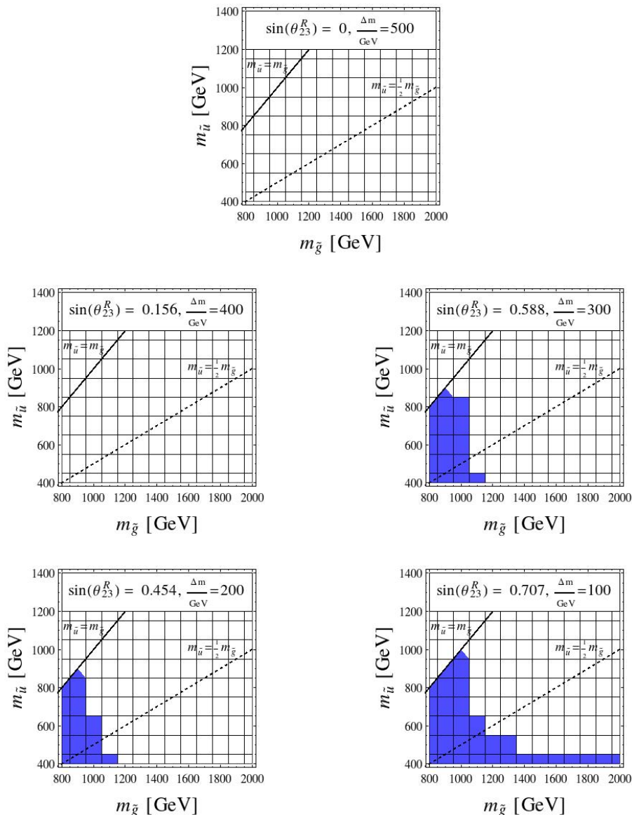
Figure 4. Sensitivity of the CMS stop search in the single lepton mode of ref. [38] for different values of the \Delta m and \theta_{23}^R parameters (the exact values being indicated in the top bar of each subfigure). The excluded regions are shown in blue in the (m_{\tilde{u}}, m_{\tilde{g}}) plane, where m_{\tilde{u}} is the mass of the lightest squark (a scharm-like squark here since \Delta m > 0 ). The upper panel describes the reference scenario in which the lightest squark is a pure scharm state and the stop is almost decoupled.
