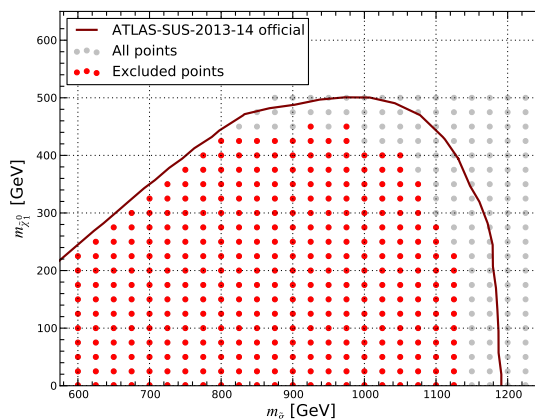
Figure 11. 95% CL exclusion limit for gluino-stop off-shell scenarios presented as contours in the gluino-neutralino mass plane. We compare results obtained with MADANALYSIS 5 (dots) to the official ATLAS results (solid line).
