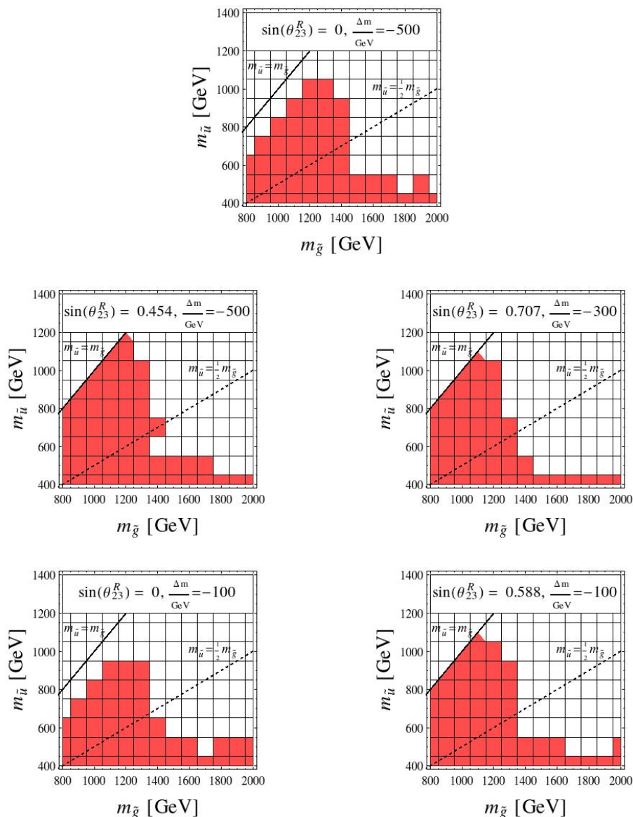
Figure 1. Sensitivity of the ATLAS multijet + \cancel{E}_T + lepton veto search of ref. [39] for different values of the \Delta m and \theta_{23}^R parameters (the exact values being indicated in the top bar of each subfigure). The excluded regions are shown in red in the (m_{\tilde{u}}, m_{\tilde{g}}) plane, where m_{\tilde{u}} is the mass of the lightest squark (a stop-like squark here since \Delta m < 0 ). The upper panel describes the reference scenario in which the lightest squark is a pure stop state and the scharm is almost decoupled.
