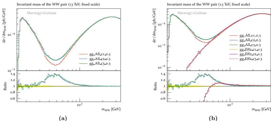
Figure 9. Invariant mass of the W -boson pair for various values of the anomalous couplings for the gg -initiated contributions, at 13 TeV. (a) shows the sum of SM and anomalous contributions. (b) shows the same as (a) but with the pure squared EFT contributions shown in addition. Note that the contributions from the first and second EFT operator, \mathcal{O}_1 and \mathcal{O}_2 , are identical in the pure squared EFT contribution (orange and purple curves), while the interference terms involving \mathcal{O}_1 and \mathcal{O}_2 , respectively, are different, as can be seen in the differences of the red and blue curves, which contain the interference terms. Ratio plots are with respect to gg_All_c1_0.3 ( c_1 = 0.3 , c_2 = c_3 = 0 ).
