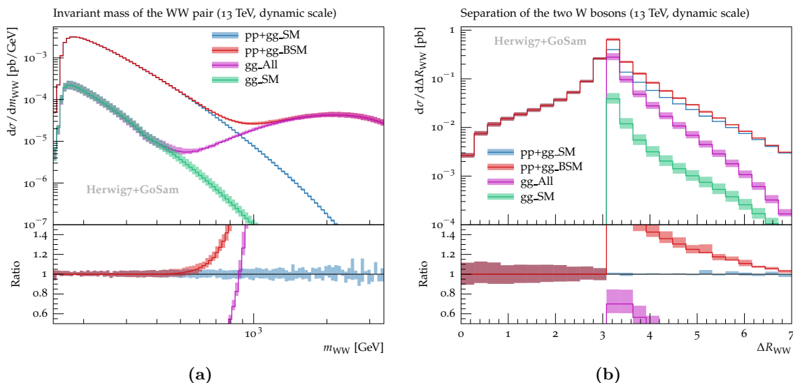
Figure 13. Distributions for (a) invariant mass m_{WW} and (b) separation \Delta R_{WW} of the reconstructed W -boson pair in pp \rightarrow W^+W^- \rightarrow e^+\nu_e\mu^-\bar{\nu}_\mu for the sum of all partonic channels, including the effects of the higher-dimensional operators. pp+gg\_SM includes all partonic channels, i.e. all the quark-initiated channels up to NLO QCD plus the loop-induced SM gg -initiated contribution gg\_SM . pp+gg\_BSM is the same but includes the loop-induced SM+BSM gg -initiated contribution gg\_All instead of just gg\_SM . In addition we show the SM and SM+BSM gg -initiated contributions separately. The shaded bands show the scale-variation uncertainties. Ratio plots are with respect to pp+gg\_SM .
