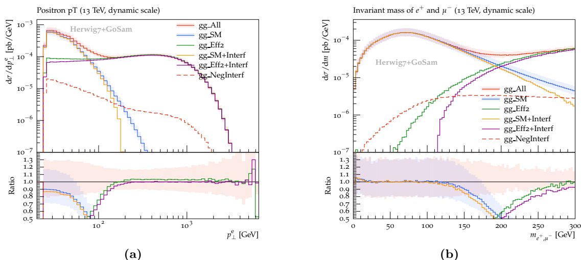
Figure 7. Transverse momentum of the positron (a) and invariant mass of the charged leptons (b), for the gg -initiated contributions. Ratio plots are with respect to gg\_All . The shaded bands show the scale-variation uncertainties.
