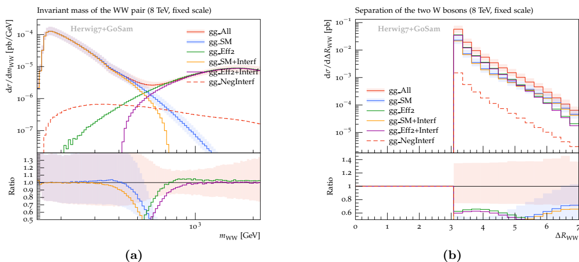
Figure 4. (a) W -boson pair invariant-mass distribution and (b) \Delta R_{WW} distribution for the SM/BSM gg -initiated contributions, at \sqrt{s} = 8 TeV. The shaded bands show the scale-variation uncertainties. Ratio plots are with respect to gg\_All .
