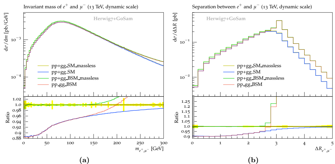
Figure 12. Impact of the top-quark loops on (a) the invariant mass of the charged leptons and (b) \Delta R_{e^+\mu^-} , considering the full pp initial state. Ratio plots are with respect to pp+gg_SM_massless .
