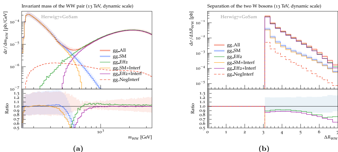
Figure 3. (a) W -boson pair invariant-mass distribution and (b) \Delta R_{WW} distribution for the SM/BSM gg -initiated contributions, at \sqrt{s} = 13 TeV. The shaded bands show the scale-variation uncertainties. Ratio plots are with respect to gg\_All .
