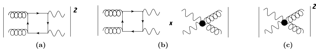
Figure 2. The three types of contributions to the squared matrix element.
