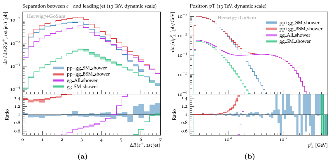
Figure 16. Same as figure 14, now showing the \Delta R_{e+j} and p_{\perp}^e distributions.
