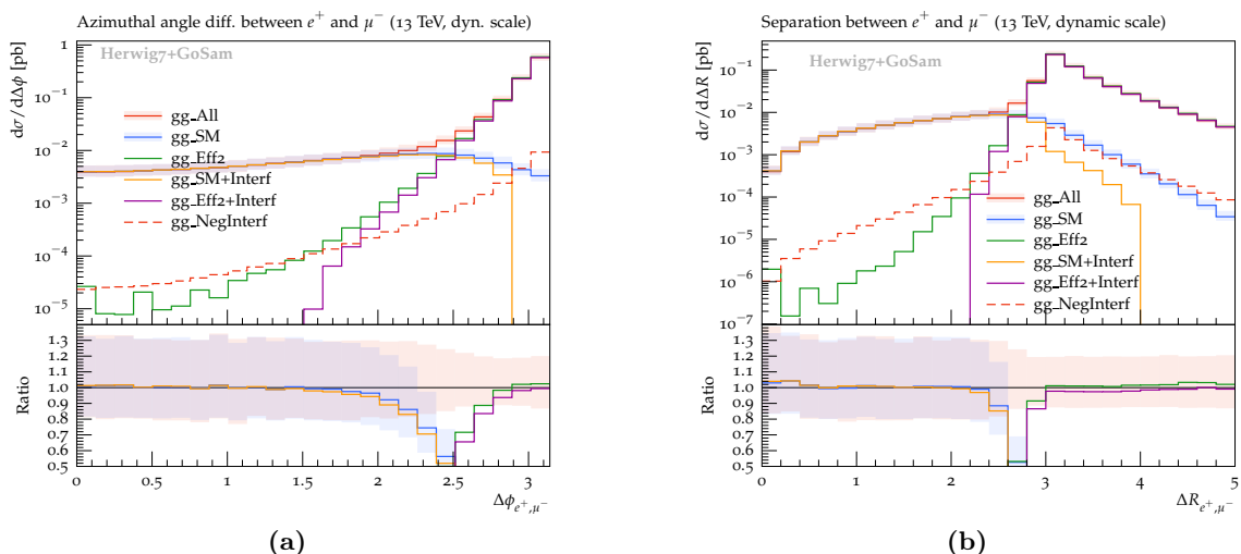
Figure 6. Distributions of (a) relative azimuthal angle \Delta\phi_{e^+\mu^-} (b) and \Delta R_{e^+\mu^-} , for the gg -initiated contributions. Ratio plots are with respect to gg\_All . The shaded bands show the scale-variation uncertainties.
