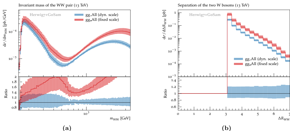
Figure 5. Scale variations, in the case of the gg -initiated contributions, for (a) the invariant-mass distribution of the W -boson pair and for (b) the \Delta R_{WW} distribution. The shaded bands show the scale-variation uncertainties. Ratio plots are with respect to gg\_All (dyn. scale).
