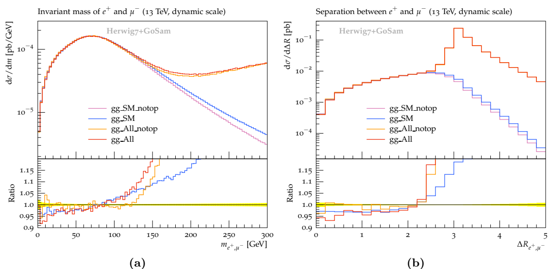
Figure 11. Impact of the top-quark loops on the invariant mass and the R -separation of the charged leptons. The curves labeled _notop show results for which diagrams with top-quarks in the loops have been omitted altogether. Ratio plots are with respect to gg_SM_notop .
