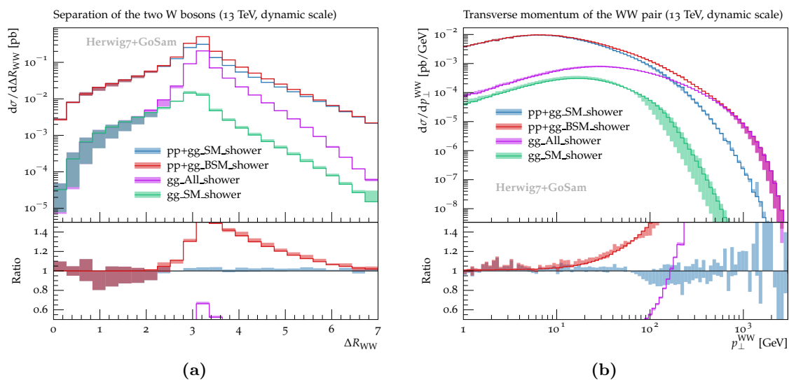
Figure 14. \Delta R_{WW} and p_{\perp}^{WW} distributions for the sum of all partonic channels contributing to pp \rightarrow W^+W^- \rightarrow e^+ \nu_e \mu^- \bar{\nu}_\mu , including \mu_Q variations and effects of the higher-dimensional operators.
