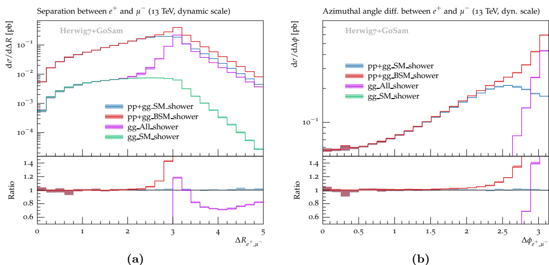
Figure 15. Same as figure 14, now showing the \Delta R_{e^+\mu^-} and \Delta\phi_{e^+\mu^-} distributions.
