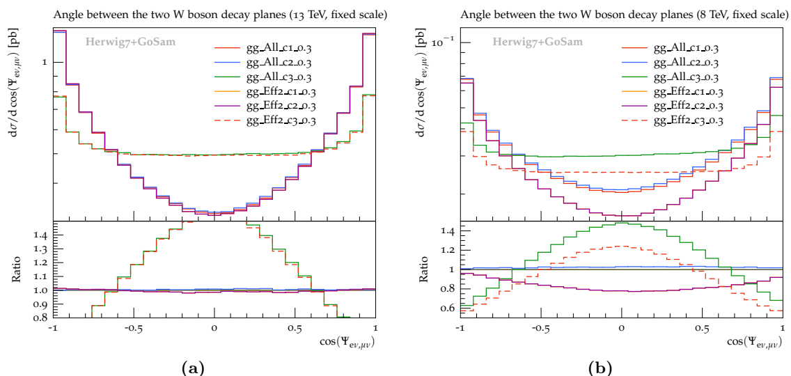
Figure 8. Angle between the W -boson decay planes for (a) 13 TeV and (b) 8 TeV. At both energies a fixed scale of \mu_r = \mu_F = M_W has been used. Ratio plots are with respect to \text{gg\_All\_c1\_0.3} ( c_1 = 0.3, c_2 = c_3 = 0 ). Comparing (a) and (b) we see that the differences to the contributions from the third operator \mathcal{O}_3 are more prominent at 13 TeV compared to 8 TeV. We also note that at 13 TeV the linear term in \mathcal{O}_3 has a bigger effect compared to 8 TeV.
