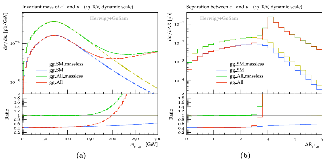
Figure 10. Top-quark mass effects on (a) the invariant mass and (b) the R -separation of the charged leptons. The curves labeled _massless show results for which the masses of the top and bottom quarks in the loops have been set to zero. Ratio plots are with respect to gg_SM_massless . The range in m_{e^+\mu^-} has been limited to 300 GeV here for better visibility of the SM/BSM transition region. We have verified that for very large values of m_{e^+\mu^-} , the yellow and blue curves merge again, as expected.
