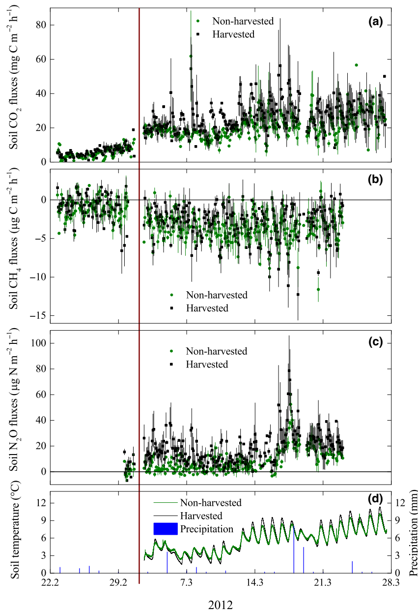
Fig. 1 Soil-atmosphere CO 2 (a), CH 4 (b), and N 2 O (c) exchange rates in a hybrid poplar short-rotation coppice near Sigmaringen, southern Germany, in 2012. Symbols represent mean values \pm standard error ( n = 3 ). The lower panel (d) shows the soil temperature at a depth of 5 cm ( ^{\circ} C) and the daily precipitation (mm). The vertical red line indicates the tree harvest.
