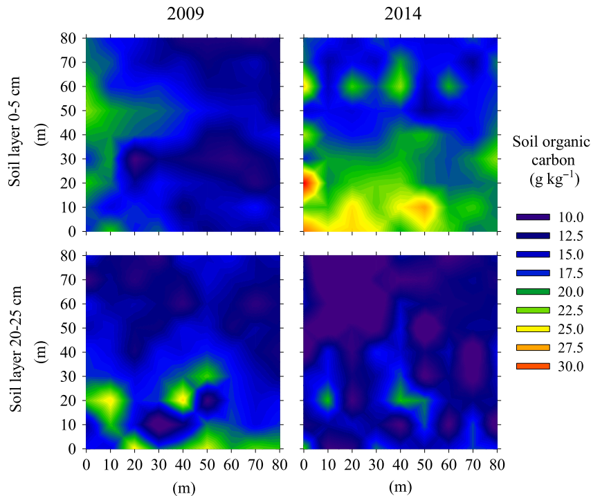
Fig. 3 Spatial distribution of soil organic carbon ( \text{g kg}^{-1} ) in the uppermost 5 cm of the mineral soil (upper panels) and at a 20 to 25 cm depth (lower panels) in a hybrid poplar short-rotation coppice near Sigmaringen, southern Germany, in 2009 (left panels) and 2014 (right panels).
