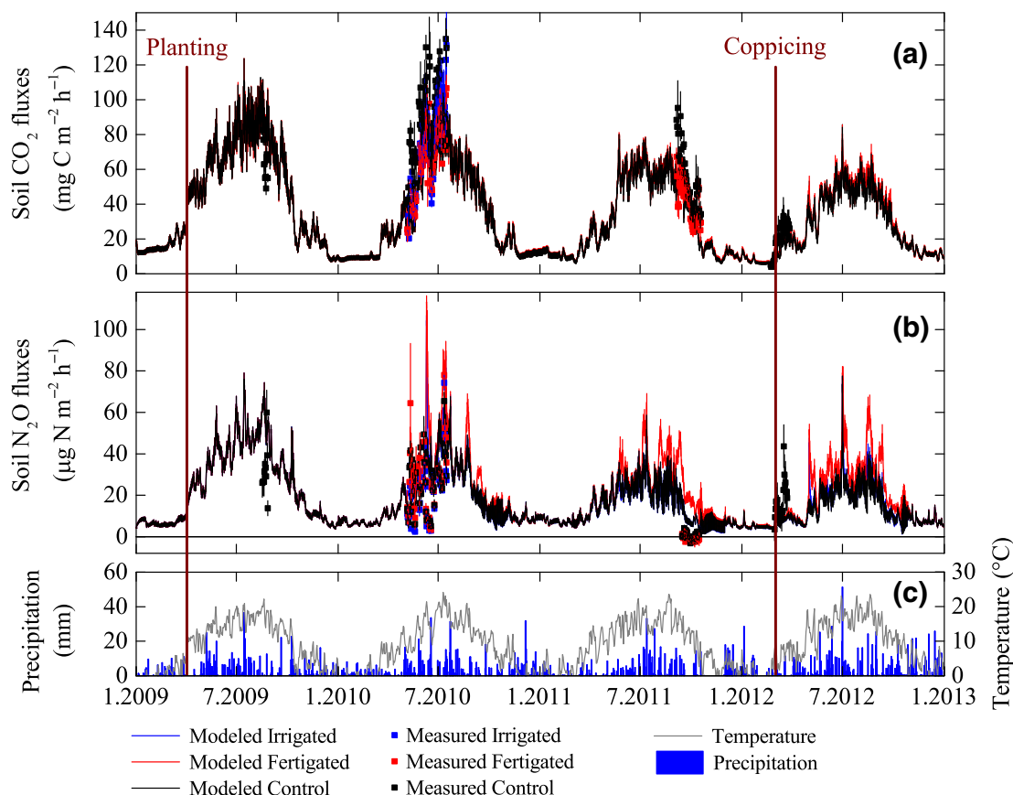
Fig. 2 Soil-atmosphere exchange rates of CO 2 (a) and N 2 O (b) in a hybrid poplar short-rotation coppice near Sigmaringen, southern Germany, as modeled using LandscapeDNDC (mean \pm standard error, n = 8 , daily values) and measured with automatic chambers (mean \pm standard error, n = 3-6 ). Panel (c) shows mean daily air temperature ( ^{\circ} C) and daily precipitation (mm). Brown vertical lines indicate planting and harvesting respectively. Note that irrigation and fertigation started in 2010.
