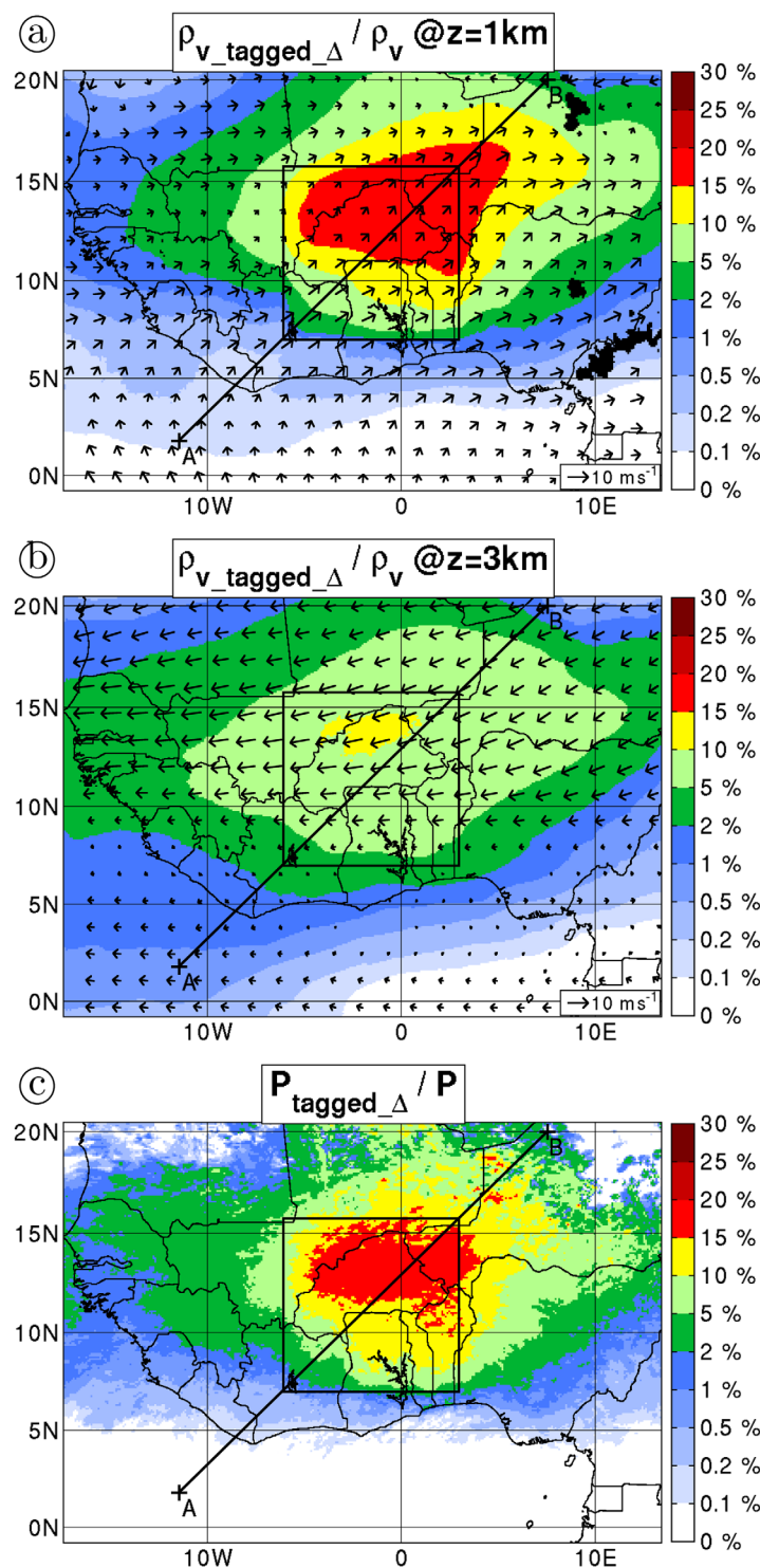
Figure 9. As in Figure 3, except for (a,b) the ratio between the density of tagged water vapor originating from E in domain \Delta , i.e., \rho_{v\_tagged\_Δ} , and the density of total water vapor \rho_v and (c) the ratio between the tagged precipitation originating from E in domain \Delta , i.e., P_{tagged\_Δ} , and total precipitation P . The black square shows the location of domain \Delta .
