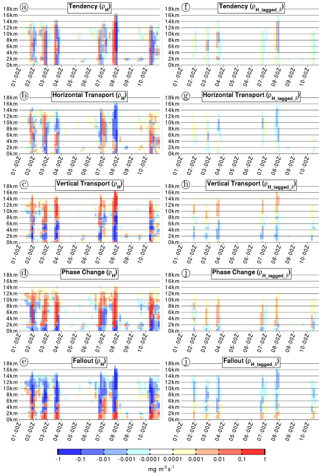
Figure 6. As in Figure 5, except for (a–e) the budget of the density of hydrometeors \rho_H and (f–j) the density of tagged hydrometeors originating from E in domain \delta , i.e., \rho_{H\_tagged\_delta} (obtained by dividing equation (4) by dz ), spatially averaged in domain \delta .
