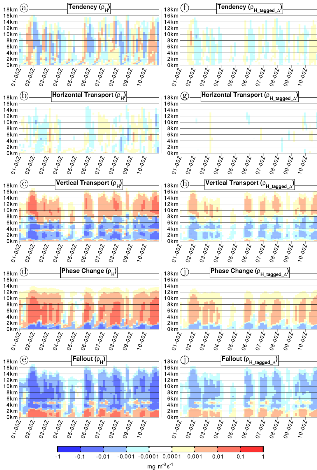
Figure 12. As in Figure 5, except for (a–e) the budget of the density of hydrometeors \rho_H and (f–j) the density of tagged hydrometeors originating from E in domain \Delta , i.e., \rho_{H\_tagged\_Delta} spatially averaged in domain \Delta .
