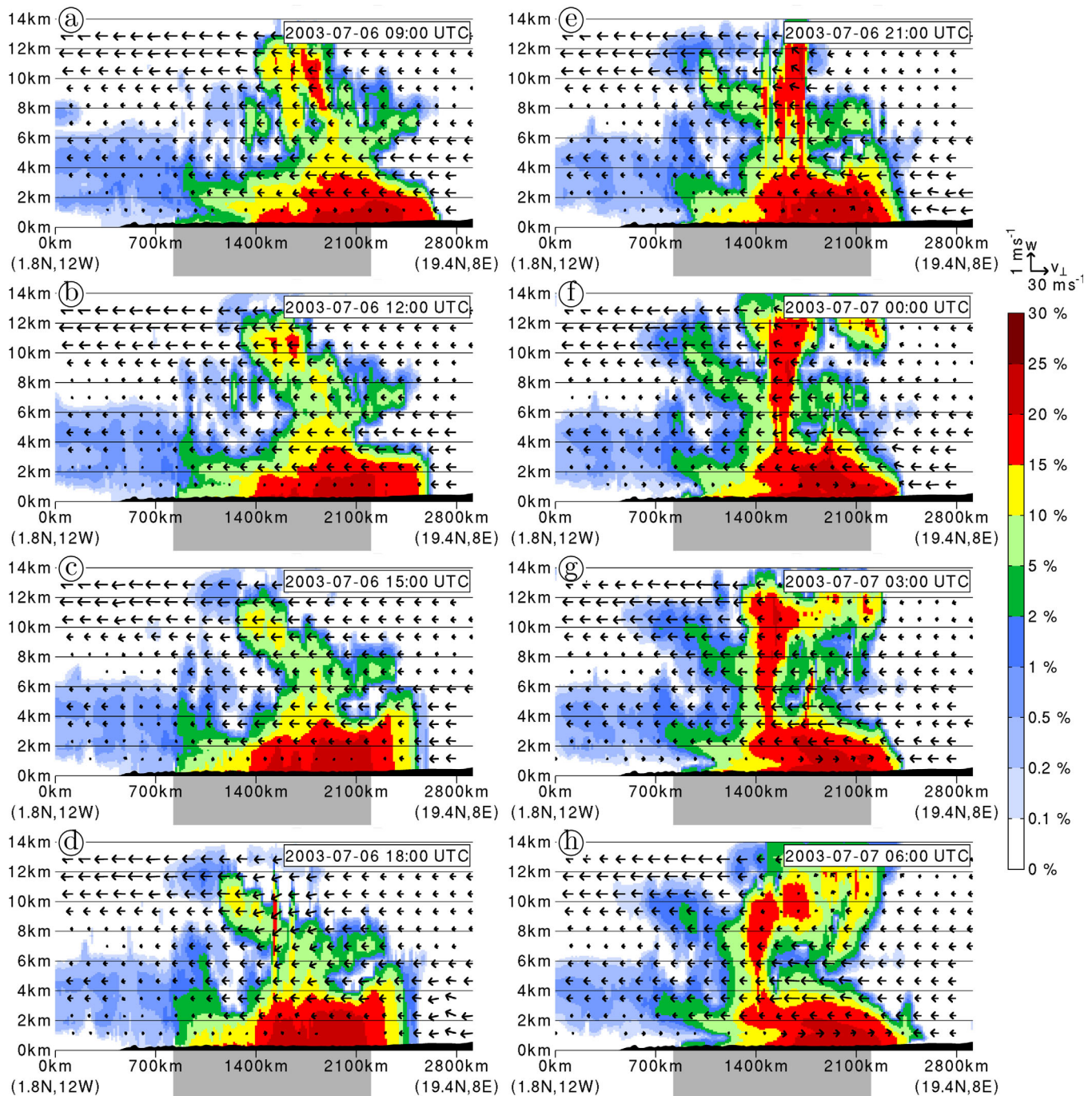
Figure 10. As in Figure 4, except for the ratio between the density of tagged water vapor originating from E in domain \Delta , i.e., \rho_{v\_tagged\_Delta} and the density of total water vapor \rho_v . The grey shade below the horizontal axis gives the location of domain \Delta .
