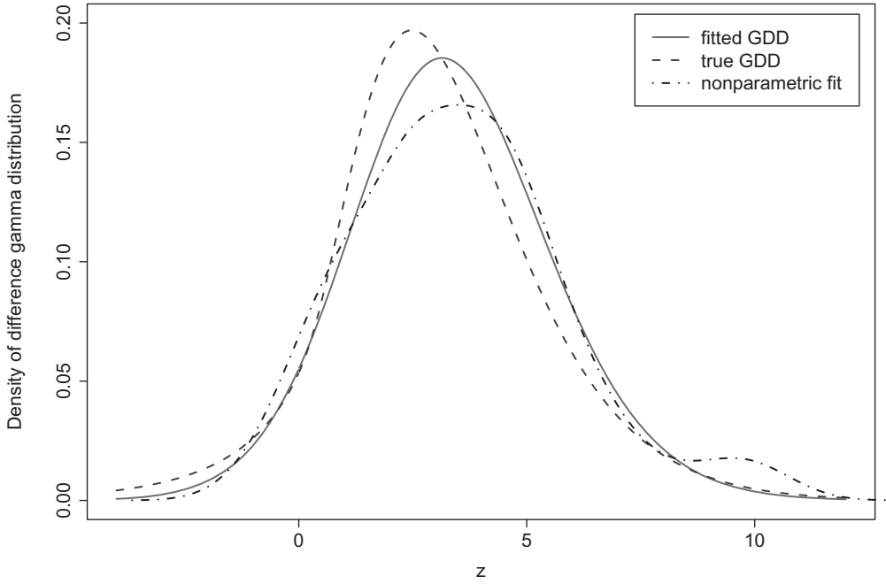
Figure 3. True and fitted GDD density function together with kernel density estimate.
