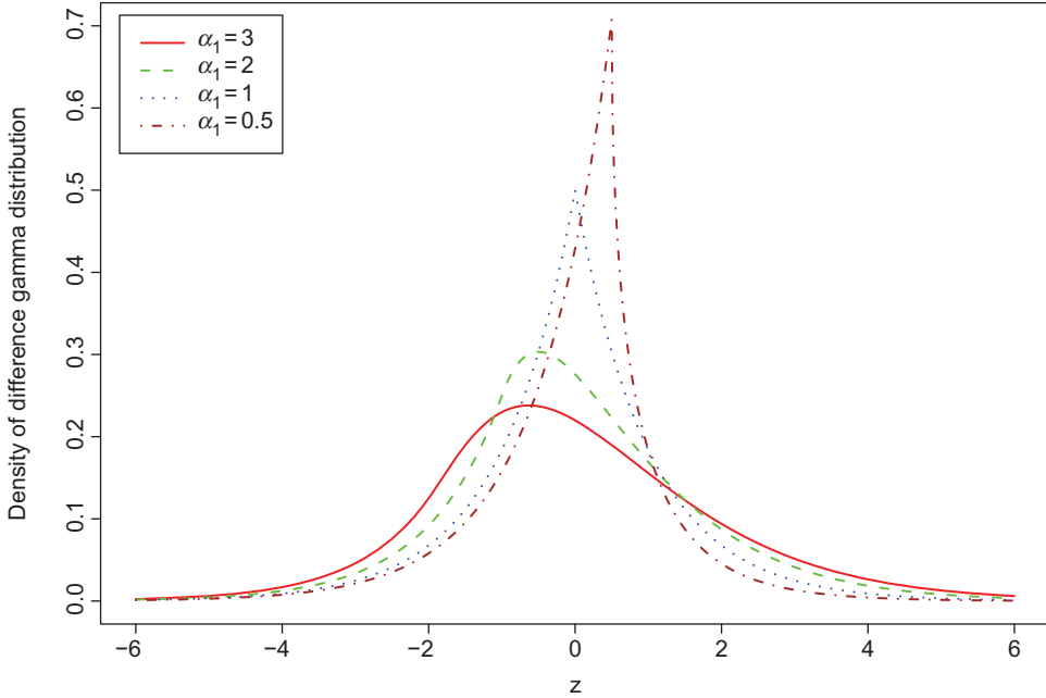
Figure 1. Densities of centred GDDs with \alpha_2 = \beta_1 = \beta_2 = 1 .
