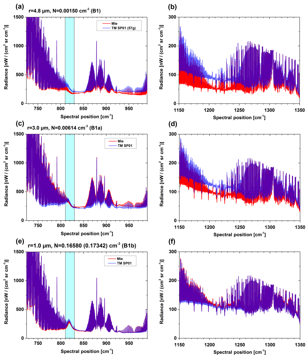
Figure B2. Sensitivity simulations investigating the effect of decreasing mode radii on the simulated spectral signatures of \beta -NAT particles for a T-Matrix scenario with AR = 0.1 (blue) and a corresponding Mie scenario (AR = 1.0, red). (a, b) Large particle mode, size distribution B1. (c, d) Intermediate particle mode, size distribution B1a. (e, f) Small particle mode, size distribution B1b. Numbers above panels (a) , (c) , and (e) indicate corresponding mode radii and particle number densities (see Fig. B1). “TM” corresponds to T-matrix simulation and “SP” to spheroid (numbers indicate AR).
