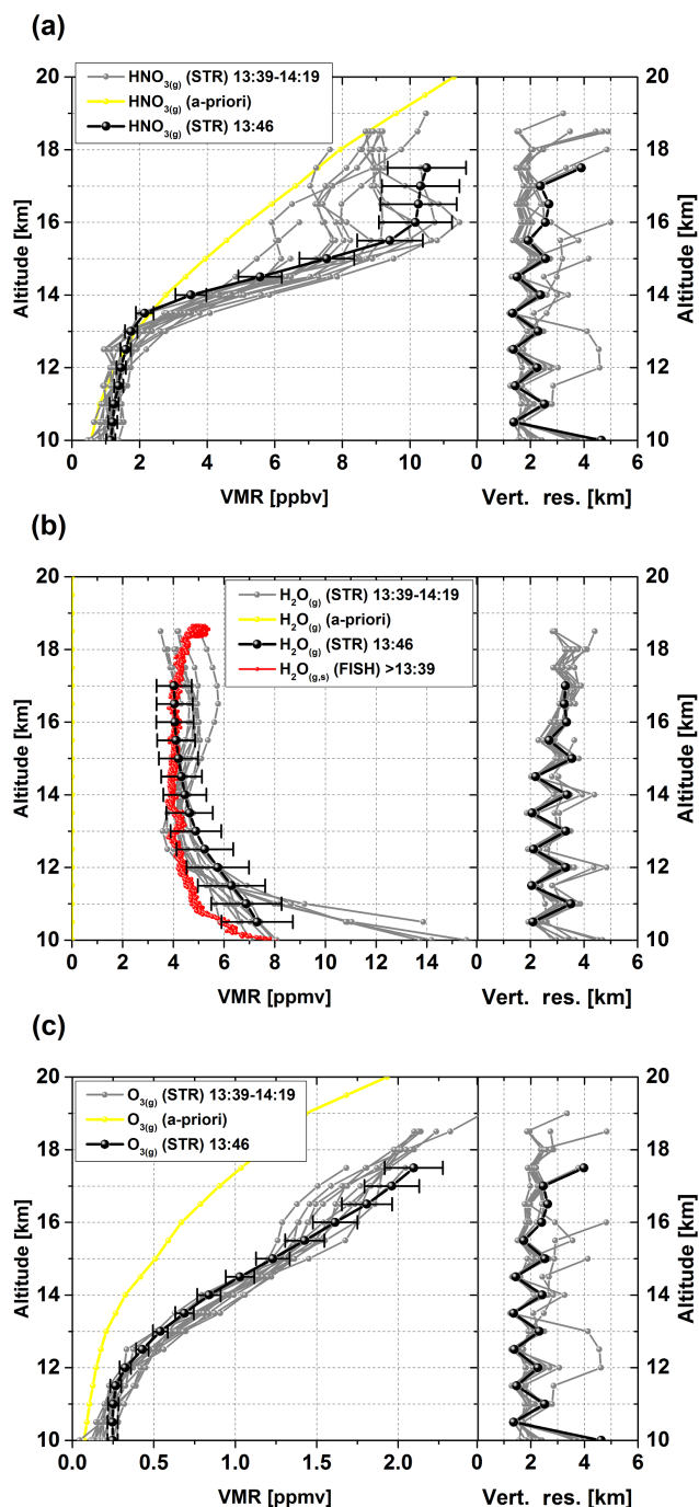
Figure A2. Left panels: vertical profiles of \text{HNO}_{3(\text{g})} , \text{H}_2\text{O}_{(\text{g})} , and \text{O}_3 retrieved from the MIPAS-STR observations during the PSC encounter (grey and black) including initial guess/a priori profiles (yellow; \text{HNO}_{3(\text{g})} and \text{O}_3 : Remedios et al., 2007; \text{H}_2\text{O}_{(\text{g})} : 0 ppmv at all altitudes). For \text{H}_2\text{O} , collocated FISH total \text{H}_2\text{O}_{(\text{g}+\text{s})} measurements during the PSC encounter and the subsequent descent phase are shown for comparison. Right panels: vertical resolutions of MIPAS-STR profiles.
