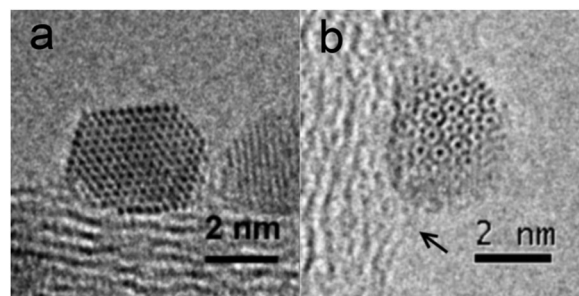
Fig. 2 Aberration corrected HRTEM images of Au particles supported on CNFs. (a) Au particle exhibits {111} facets epitaxially parallel to the ordered graphitic layer; (b) Au particle exhibits rough surfaces on the disordered graphitic surface of CNFs. Adapted with permission from ref. 68. Copyright 2013 Wiley VCH Verlag GmbH & Co. KGaA, Weinheim.
