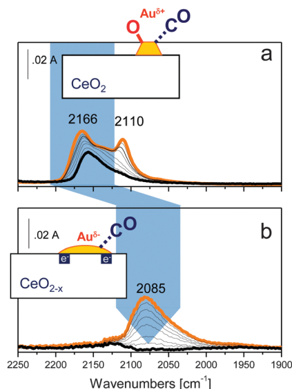
Fig. 19 FTIR spectra of oxidized (section a) and reduced (section b) AuCeO 2 collected after CO adsorption (15 mbar) at ambient temperature (orange curve), at decreasing pressures (fine curves) and under outgassing at r.t. (bold curve). The blue arrow is an eye guide to follow the pre-treatment induced evolution of bands.
