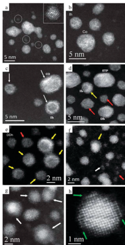
Fig. 30 Representative STEM HAADF images of the starting colloids (a and b) a Au/Pd random alloy, (c-e) Pd core/Au shell particles and (f-h) Au core /Pd shell particles. Reproduced with permission from ref. 89. Copyright 2011, The Royal Society of Chemistry.
