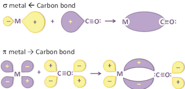
Scheme 1 Metal carbonyl bond: formation of a \sigma metal \leftarrow carbon bond and of a \pi metal \rightarrow carbon bond. The other CO molecular orbitals are omitted for the sake of clarity; the violet orbitals are full, the yellow one is empty.
