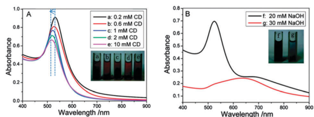
Fig. 9 (A) UV Vis absorption spectra of the AuNPs prepared at different \alpha CD concentrations; (B) UV Vis absorption spectra of the AuNPs prepared at different NaOH concentrations. Adapted with permission from ref. 170. Copyright (2009) American Chemical Society.
