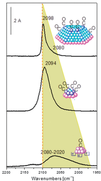
Fig. 17 FTIR spectra of 0.5 mbar CO adsorbed at 116 °C on Au/TiO 2 (top curve), Au/ZrO 2 (middle curve) and Au/CeO 2 (bottom curve). Spectra normalised with respect to Au content and absorption coefficients.
