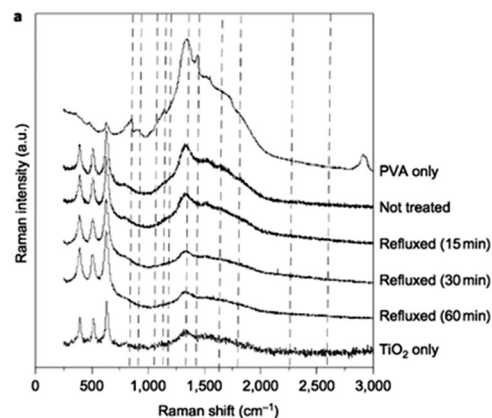
Fig. 25 Monitoring the presence of PVA present on a 1 wt% Au/ \text{TiO}_2 catalyst by Raman spectroscopy. Figure reproduced with permission from Nature publishing. 313
