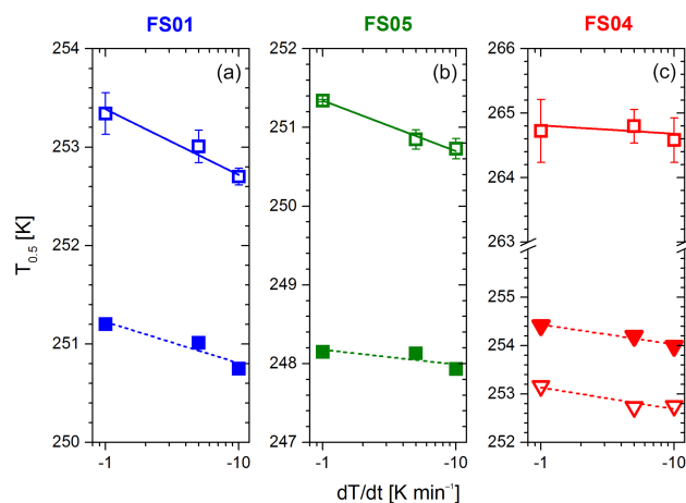
Figure 12. (a, b) Median freezing temperature T_{0.5} for the aqueous suspensions of FS01 and FS05 aged for over 5 months (blue and green filled symbols). (c) Median freezing temperature T_{0.5} of FS04 0.8 wt % suspension treated with 30 % \text{H}_2\text{O}_2 for an hour (filled triangles) and overnight (open triangles). T_{0.5} for the freshly prepared suspensions is shown as open square symbols in all three panels. Straight lines are non-weighted linear regressions of the averaged T_{0.5} values for three different cooling rates.
