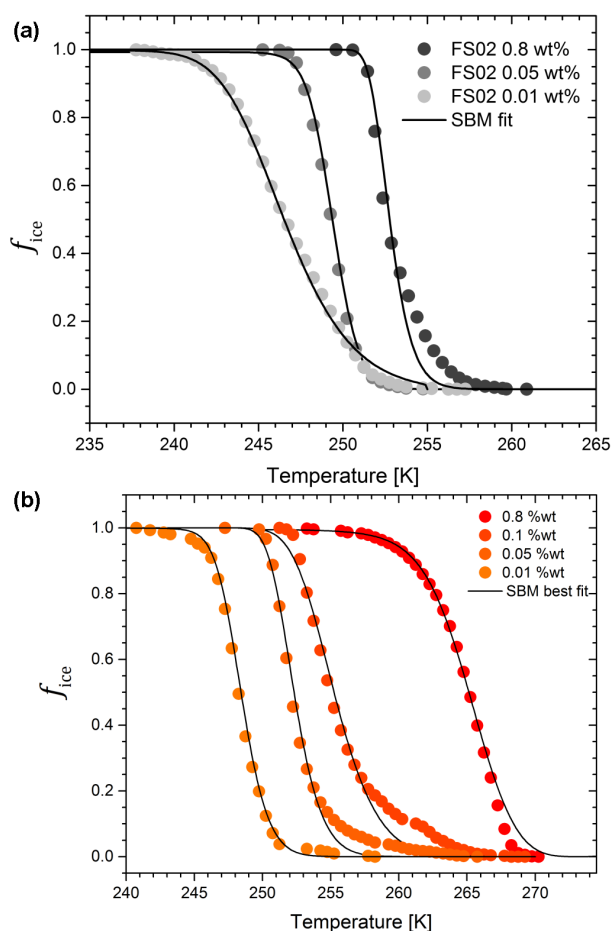
Figure 6. Freezing curves of FS02 (a) and FS04 (b) binned into 0.5 K temperature intervals (filled symbols) and SBM best fit (solid curves). Fit parameters are given in Table 2a.
