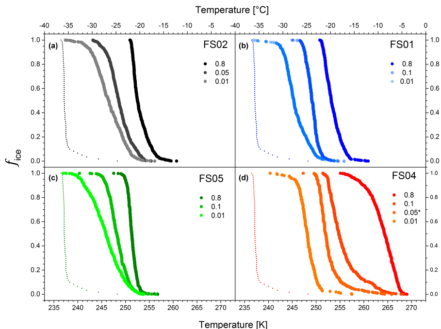
Figure 5. Frozen fraction curves of feldspar suspensions with various concentrations for (a) FS02, (b) FS01, (c) FS05, and (d) FS04 samples. Suspension concentration is given in the legend of each plot in wt %. Frozen fraction curves for Nanopure water droplets on a clean silicon wafer are indicated by the dotted line on each plot. All curves were measured with a cooling rate of -1 \text{ K min}^{-1} except for FS05 0.05 wt %, for which the cooling rate was -5 \text{ K min}^{-1} (marked with an asterisk). Note the initiation of freezing at 268 K for FS04 0.8 wt % suspension droplets.
