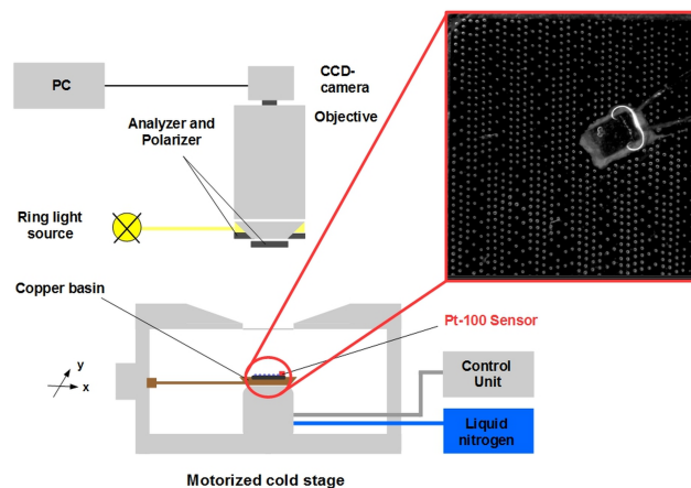
Figure 1. Schematic drawing of the nanoliter droplet freezing assay setup (side view). The inset shows the top view of 10 × 10 mm Si-wafer with ≈ 1200 droplets immersed in silicon oil. The square shape near the center of the wafer is the Pt-100 temperature sensor.
