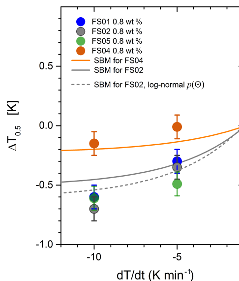
Figure 8. The shift \Delta T_{0.5} of the median temperature T_{0.5} relative to the T_{0.5} at 1 \text{ K min}^{-1} for different cooling rates c = dT/dt . Solid lines represent expected \Delta T_{0.5}(c) calculated with fit parameters given in Table 2. Dashed line is the theoretical temperature shift calculated with the same SBM parameters for FS02 but assuming the log-normal distribution of contact angles p(\theta) .
