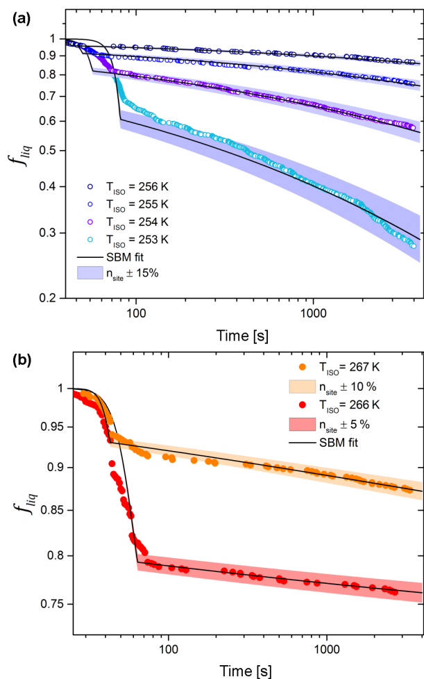
Figure 7. Decay of the fraction of liquid droplets with time for FS02 (a) and FS04 (b) for different T_{ISO} (log–log scale). Solid lines show composite SBM fit with parameters given in Table 2 (see Sect. 7 for detailed discussion). Shaded areas indicate the variability n_{site} \pm \Delta n_{site} of a best-fit value, with actual \Delta n_{site} given in the legend.
