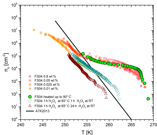
Figure 13. n_s(T) curves of K-feldspar particles (FS04) after heating to 90 °C and chemical treatment with hydrogen peroxide.
