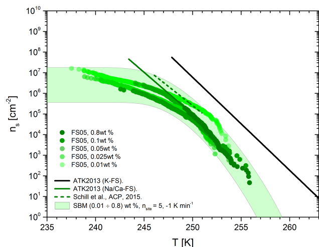
Figure 10. n_s(T) curves of Na/Ca-feldspar suspensions FS05. Shaded area shows the range of n_s(T) values predicted by Eq. (4) with fixed-fit parameter set \mu_\theta = 1.33 rad, \sigma_\theta = 0.102 rad, n_{\text{site}} = 5 , and concentration of feldspar suspensions varied between 0.01 and 0.8 wt %. Black and green solid lines are exponential fits of data from ATK2013 for K-rich and Na/Ca-rich feldspar suspension droplets, respectively.
