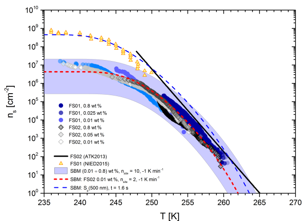
Figure 9. n_s(T) curves of K-feldspar particles FS01 and FS02. The shaded area shows the range of n_s(T) values predicted by Eq. (4) with fixed parameter set \mu_\theta = 1.32 rad, \sigma_\theta = 0.1 rad, n_{\text{site}} = 10 , and suspension between 0.01 and 0.8 wt %. The red broken line corresponds to the best-fit parameter set for FS02 (Table 2a) with 0.01 wt % and dT/dt = -1 K \text{min}^{-1} . The blue broken line is calculated with the same parameter set but assuming a single FS01 particle with Stokes diameter 500 nm per droplet and fixed temperature lasting for 1.6 s (LACIS conditions) instead of constant cooling rate.
