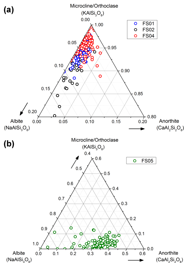
Figure 3. EDX data of individual feldspar particles plotted on the ternary phase diagram based on elemental mass percentages. (a) Ternary phase diagrams of K-feldspar particles (FS01, FS02, and FS04) and (b) Na/Ca-feldspar particles (FS05). Note the different scales of the ternary axis.
