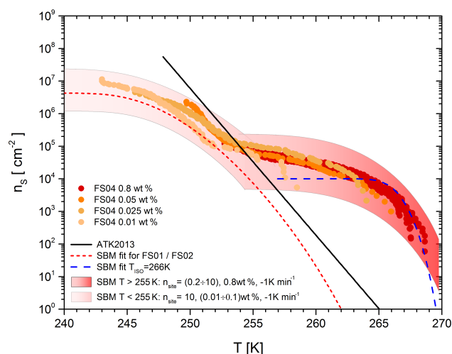
Figure 11. n_s(T) curves of K-feldspar particles (FS04). Shaded areas show the range of n_s(T) values (for details see text). The black solid line is a fit of data from ATK2013 for FS02. The red broken line is a fit to our FS02 data (as in Fig. 9). Blue broken line is the n_s(T) curve predicted by Eq. (4) with parameters obtained from the isothermal freezing experiments (Table 2b).
