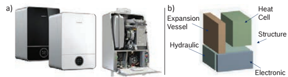
Fig. 6. (a) Junkers Cerapur 9000 (courtesy of Bosch TT); (b) modular boiler
