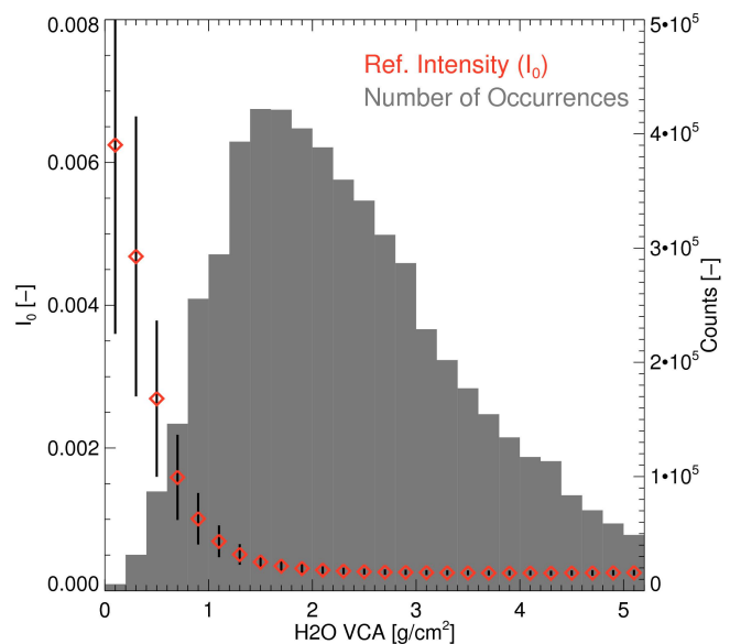
Fig. 2. Analysis of 1.4 \mu\text{m} (1390 nm–1410 nm) radiances as measured by SCIAMACHY for the years 2003–2009. The red diamonds show the reference intensity ( I_0 ) as a function of the water vapour vertical column amount ( \text{H}_2\text{O VCA} ). The reference intensity is defined as the mean of the 40 % lowest values of the (sun-normalised) radiances (corresponding to scenes with no clouds or very small effective cloud cover). The black vertical lines are the corresponding standard deviations. The grey histogram shows the number of occurrences as a function of the water vapour vertical column amount.
