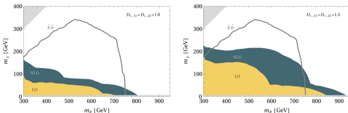
Figure 6. Limits on the mDMFV model from CMS squark searches [1].
