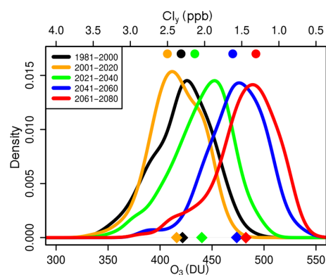
Figure 2. Probability density functions (PDFs) for 20-year intervals taken from the period 1981 to 2080 for Arctic mean total ozone column (DU) in March. Each PDF contains data from seven ensemble members. Coloured diamonds indicate the 20-year means of the total ozone columns and coloured points the corresponding means of Arctic mean \text{Cl}_y (ppb) at 20 km.
