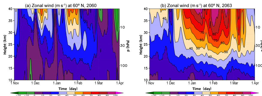
Figure 9. Time–altitude cross sections of the daily Arctic ( 60^{\circ} N) zonal mean zonal wind ( \text{m s}^{-1} ) in (a) 2060 and (b) 2063.
