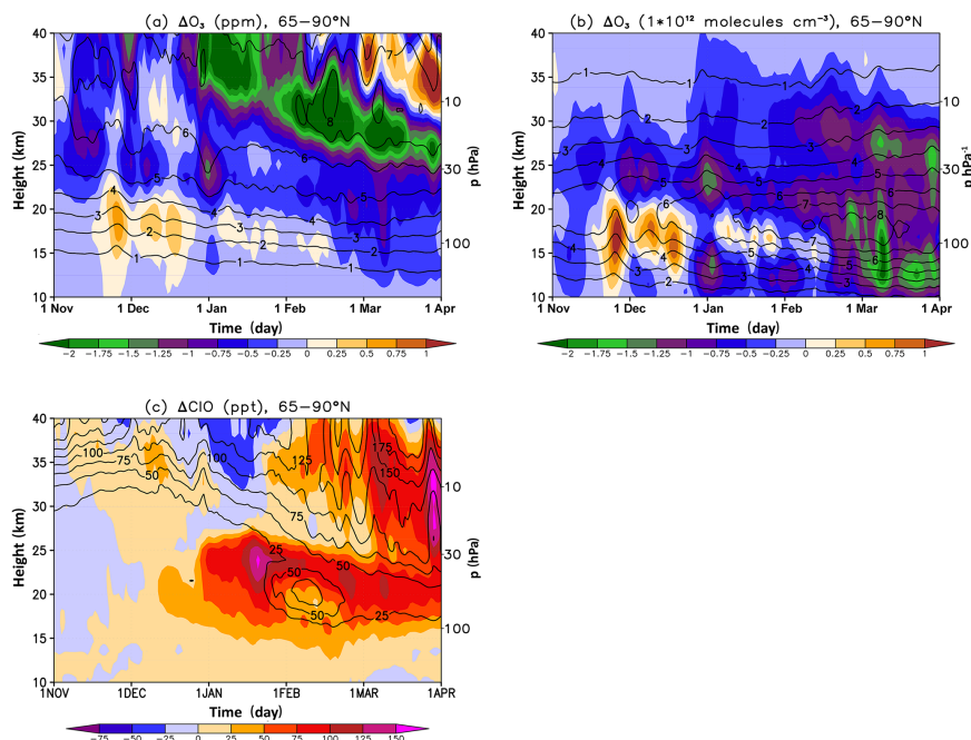
Figure 10. Colours: time–altitude cross sections of the Arctic mean differences between the years 2063 and 2060 in (a) ozone mixing ratios (ppm), (b) ozone number density ( 10^{12} molecules \text{cm}^{-3} ) and (c) ClO mixing ratio (ppt). The solid contours show the year 2060 for reference.
