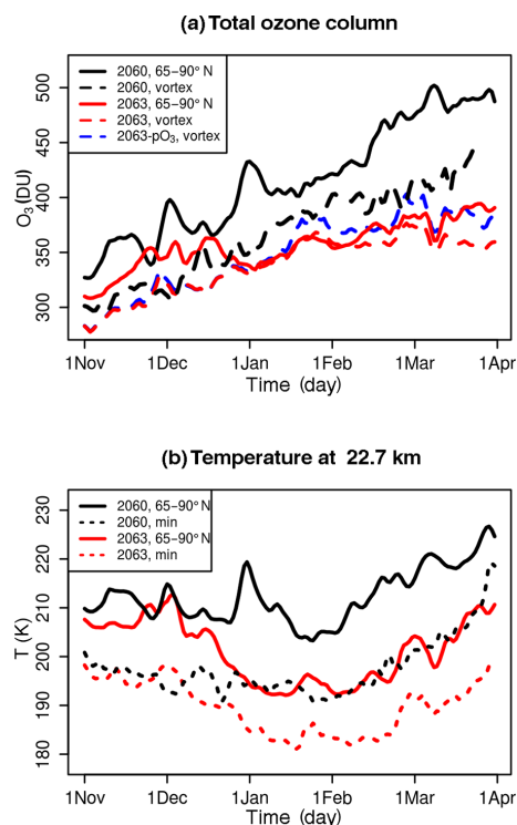
Figure 8. Time series of Northern Hemisphere (a) daily total column ozone (DU) during the winters 2060 (black) and 2063 (red) and (b) temperature (K) at 22.7 km. Solid lines show the Arctic mean (65–90° N), dashed lines in (a) show polar vortex averages (see text for details) and dotted lines in (b) show minimum daily mean temperatures found anywhere poleward of 65° N. The blue dashed line in (a) shows the evolution of the vortex-averaged passive ozone tracer in 2063.
