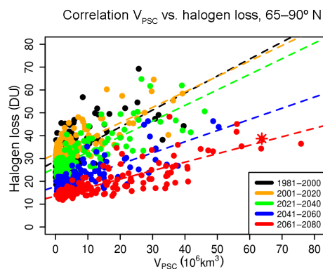
Figure 5. Scatter plot for November to March mean potential V_{\text{PSC}} ( \times 10^6 \text{ km}^3 ) against halogen-induced ozone loss (DU) over 1–25 km integrated over the same months. Colours denote the same 20-year intervals as in Fig. 2. Dashed lines indicate linear fits for the individual 20-year periods. The model year 2063 analysed in Sect. 3.3 is highlighted with a red asterisk.
