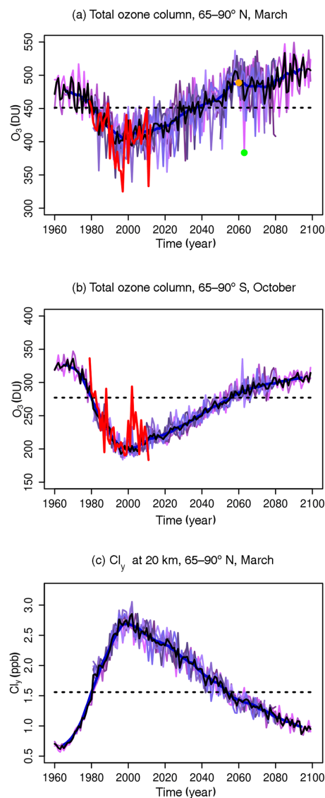
Figure 1. Time series of monthly mean polar averaged (65–90°) total column ozone (DU) from 1960 to 2099 for (a) the Arctic in March and (b) the Antarctic in October. (c) As in (a) for the March total inorganic chlorine loading (Cl y ) at 20 km (ppb). The red lines in (a, b) denote observations from the Bodeker total ozone column dataset (Bodeker et al., 2005; Müller et al., 2008). Thick black and blue lines denote the ensemble mean and its 11-year running average, respectively. Orange and green points in (a) denote the two case study years of 2060 and 2063, respectively, described in Sect. 3.3.
