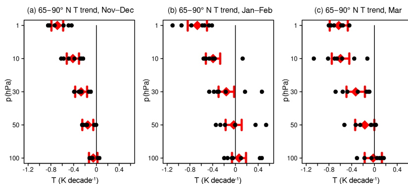
Figure 4. Linear trends in Arctic mean temperature ( \text{K decade}^{-1} ) at selected stratospheric pressure levels in (a) November/December, (b) January/February and (c) March calculated for each ensemble member individually (black points) for the period 1981–2080. Red diamonds and whiskers show the corresponding trends ( \pm 2 standard errors) calculated for the ensemble mean.
