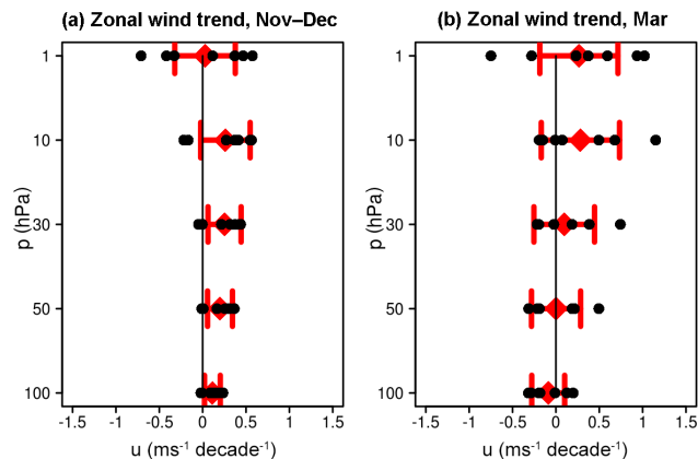
Figure 7. Linear trends in zonal mean zonal wind ( \text{m s}^{-1}\text{ decade}^{-1} ) at 61^\circ\text{ N} at selected stratospheric pressure levels in (a) November/December and (b) March calculated for each ensemble member individually (black points) for the period 1981–2080. Red diamonds and whiskers show the corresponding trends ( \pm 2 standard errors) calculated for the ensemble mean.
