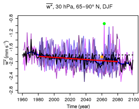
Figure 6. Time series of DJF mean residual vertical velocity, w^* ( \text{mm s}^{-1} ), over 65\text{--}90^\circ\text{ N} at 30 hPa from 1960 to 2099. Thick black and blue lines denote the ensemble mean and its 11-year running average, respectively. Thick red line shows the linear trend calculated for the ensemble mean over the 1981–2080 period. Orange and green points denote the two case study model years 2060 and 2063, respectively, discussed in Sect. 3.3.
