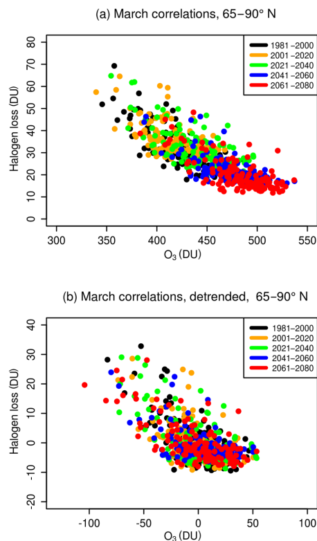
Figure 3. (a) Scatter plot of Arctic mean March total column ozone (DU) vs. cumulative (1 November to 30 March) halogen-induced total ozone loss (DU) (see Sect. 2.3) summed from the surface to 25 km. Each point shows a single winter and the colours denote the same 20-year intervals as in Fig. 2. (b) As in (a) but for deviations of column ozone and halogen losses from their corresponding 11-year running ensemble mean.
