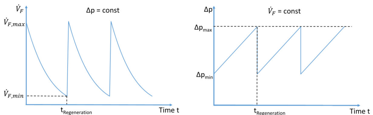
Figure 1: Operating conditions in filtration process for constant pressure difference (left) and constant filtrate flow (right), based on Melin et al. [2].
