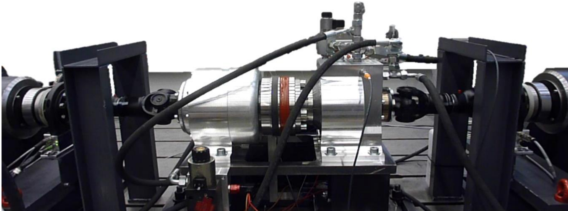
Fig. 6: Demonstrator during a test run on the test bench.
