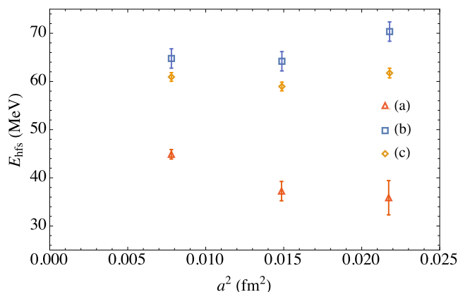
Figure 2. The results of the lattice simulation of the bottomonium hyperfine splitting with \mathcal{O}(v^6) NRQCD action and the four-quark Wilson coefficient given by (a) the asymptotic expansion about the continuum limit [1], (b) the direct numerical matching and (c) d_\sigma = 0 [2]. All data points include the statistical error and the uncertainty in the value of the lattice spacing. The error bars of (a) include also the uncertainty due to the higher order perturbative corrections. The difference between (a) and (b) data sets is mainly due to the spurious linear Coulomb artifact contributing to (b).
