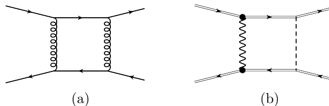
Figure 1. One-loop Feynman diagrams with Coulomb singularity contributing to the spin-dependent one-particle irreducible part of the scattering amplitude in QCD (a) and NRQCD (b). The symmetric NRQCD diagram is not shown. In the diagram (b) the double arrow, dashed and wavy lines stand for the nonrelativistic quark, Coulomb and transverse gluon propagators, respectively. The black circles denote the effective spin chromomagnetic interaction proportional to the Wilson coefficient c_F in eq. (1.1).
