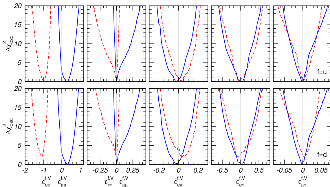
Figure 1. Dependence of the \Delta\chi^2_{\text{OSC}} function for the global analysis of solar, atmospheric, reactor and LBL data on the NSI parameters \epsilon_{\alpha\beta}^{f,V} for f = u (upper panels) and f = d (lower panels). Solid curves correspond to the standard LMA solution and dashed curves correspond to the LMA-D degeneracy. These results correspond to the current limits assuming light NSI mediators. Results adopted from ref. [13].
