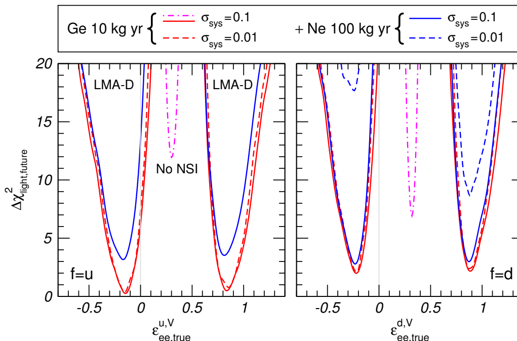
Figure 8. The full and dashed lines show \Delta\chi_{\min}^2 (LMA-D) from a combination of current oscillation and future COHERENT data (for different assumptions on target and systematics as labeled) as a function of the assumed value of \epsilon_{ee,\text{true}}^{q,V} . All other true values used to generate COHERENT data are set to the current best fit point from oscillations. To determine the minimum of the joint \chi^2 in the LMA-D region all oscillation and NSI parameters are varied. The dash-dotted curve shows the \Delta\chi^2 for no-NSI under the same assumptions for our default COHERENT configuration.
