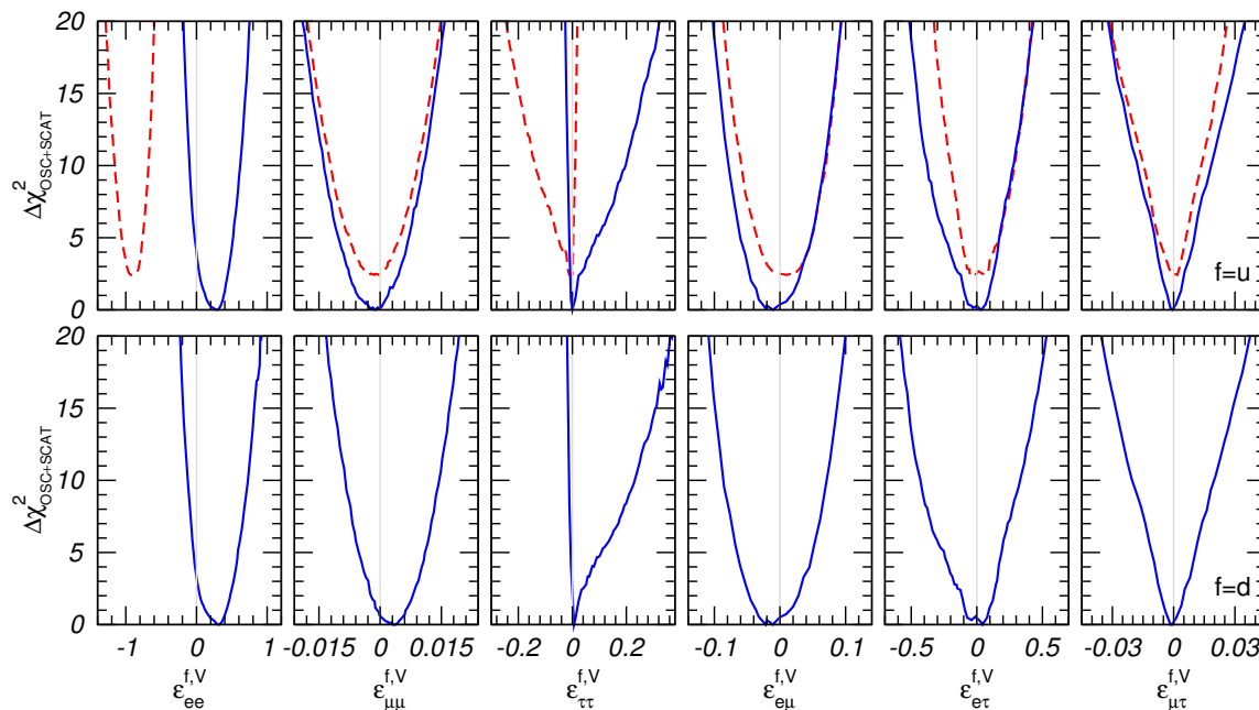
Figure 4. Dependence of the \Delta\chi_{\text{OSC+SCAT}}^2 on the NSI parameters \epsilon_{\alpha\beta}^{q,V} for q = u (upper panels) and q = d (lower panels), for both LMA (solid) and LMA-D (dashed) regions from the combined analysis of global oscillation and CHARM + NuTeV scattering data. These results correspond to the current limits assuming heavy NSI mediators.
