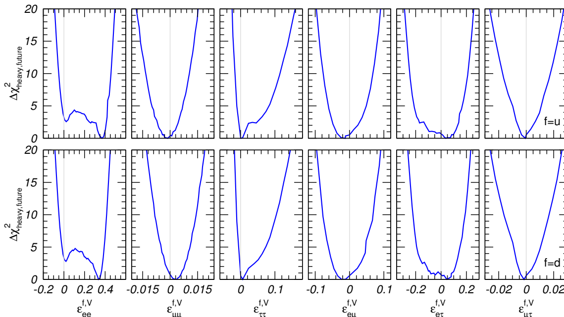
Figure 9. Dependence of \Delta\chi_{\text{heavy,future}}^2 on the NSI parameters \epsilon_{\alpha\beta}^{f,V} for f = u (upper panels) and f = d (lower panels), using current global data on oscillations and DIS data from NuTeV and CHARM combined with artificial COHERENT data generated for all \epsilon_{\alpha\beta} set to zero.
