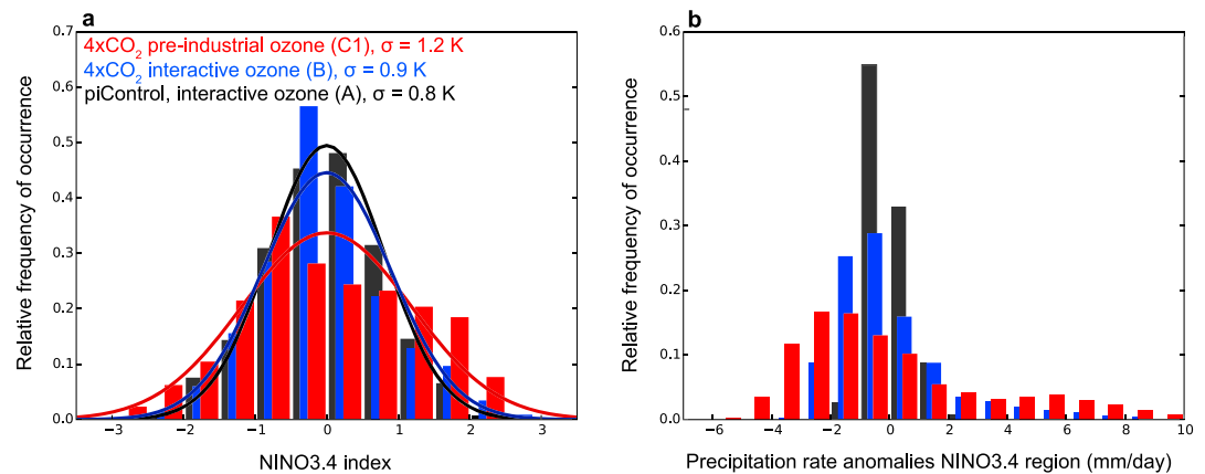
Figure 1. Normalized histograms of NINO3.4 (a) temperature and (b) precipitation rate anomalies as relative frequencies of occurrence, color coding for the integrations as in Figure 1a.
