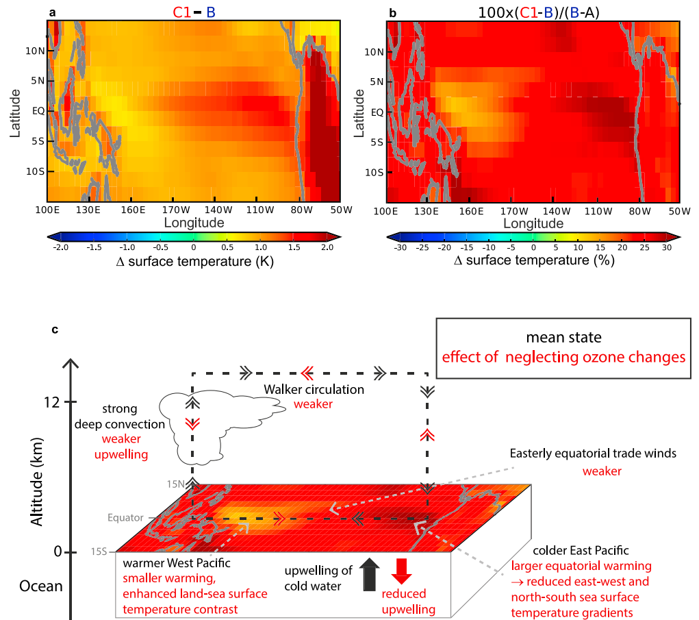
Figure 4. (a) Surface temperature differences (K) between the 4xCO 2 runs with preindustrial ozone (C1) and interactive chemistry (B) for the region 15N–15S, 100E–50W. (b) The same temperature anomalies expressed as percentage differences relative to the surface warming caused by 4xCO 2 from run A to B. (c) Sketch summarizing the climatological mean state effect of neglecting ozone changes.
