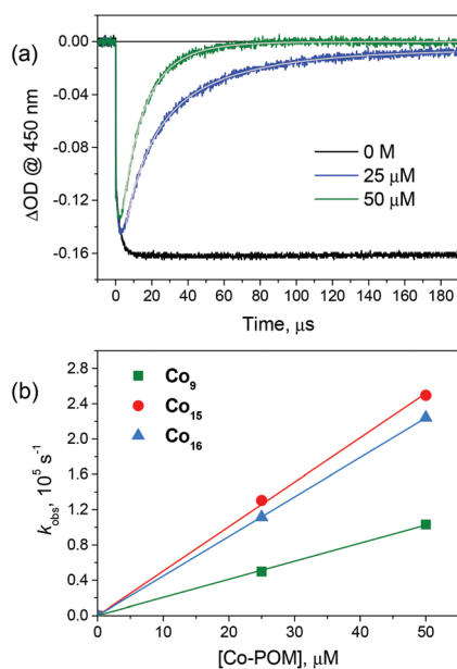
Fig. 3 (a) Laser flash photolysis experiments ( \lambda_{\text{exc}} = 355 \text{ nm} ) in aqueous phosphate buffer (pH 8) containing 5 mM \text{S}_2\text{O}_8^{2-} , 50 \mu\text{M} \text{Ru}(\text{bpy})_3^{2+} , and 0–50 \mu\text{M} \text{Co}_9 . (b) Plots of pseudo-first-order rate constants of bleach recovery vs. catalyst concentration, yielding bimolecular hole scavenging rate constants of 2.1 \times 10^9 , 5.0 \times 10^9 and 4.5 \times 10^9 \text{ M}^{-1} \text{ s}^{-1} for \text{Co}_9 , \text{Co}_{15} and \text{Co}_{16} , respectively.
