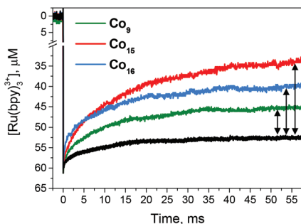
Fig. 4 Laser flash photolysis experiments ( \lambda_{\text{exc}} = 355 \text{ nm} ) in aqueous phosphate buffer (pH 8) containing 5 mM \text{S}_2\text{O}_8^{2-} , 50 \mu\text{M} \text{Ru}(\text{bpy})_3^{2+} (black trace), and 1 \mu\text{M} \text{Co}_9 (green trace), 0.5 \mu\text{M} \text{Co}_{15} (red trace), and 0.5 \mu\text{M} \text{Co}_{16} (blue trace). The amount of \text{Ru}(\text{bpy})_3^{3+} reduced by the catalyst in the time lag of the experiment (indicated by vertical double arrows) is 7.5 \mu\text{M} for \text{Co}_9 , 16 \mu\text{M} for \text{Co}_{15} and 10 \mu\text{M} for \text{Co}_{16} .
