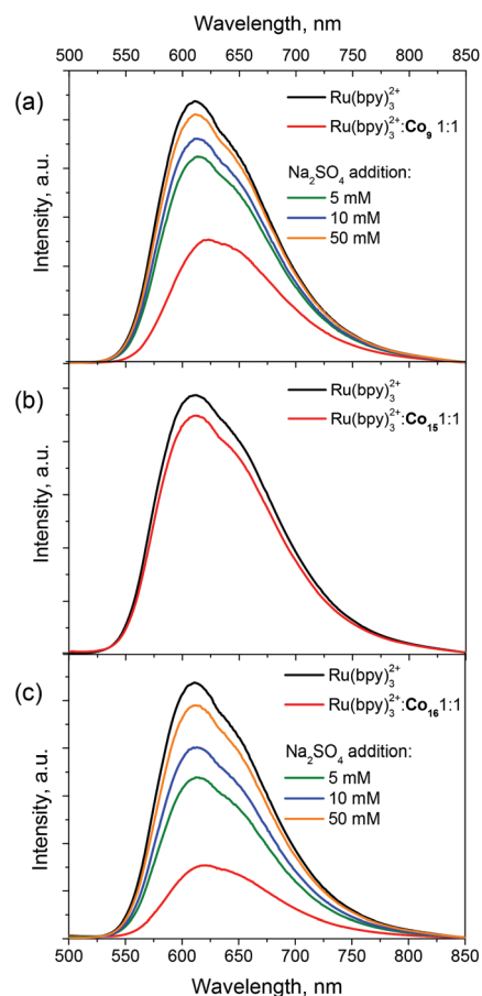
Fig. 2 Variation of Ru(bpy) 3 2+ photoluminescence (50 μM, air-equilibrated water solution, excitation at 450 nm) upon addition of Co 9 (a), Co 15 (b) and Co 16 (c). Black traces: Ru(bpy) 3 2+ (reference); red traces: Ru(bpy) 3 2+ : Co-POM 1 : 1; green, blue, orange traces: Ru(bpy) 3 2+ : Co-POM 1 : 1 in the presence of 5–50 mM Na 2 SO 4 .
