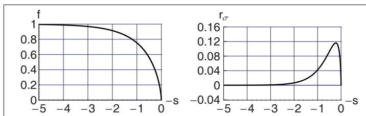
Fig. 1. The left panel gives the analytic infinite-radius q -ball profile f(s) from (5.17) with f(0) = 0 and f \uparrow f_0 = 1 for -s \rightarrow -\infty . Here, f refers to the dimensionless q -field and s to the dimensionless spatial coordinate orthogonal to the edge of the infinite-radius q -ball. The right panel gives the corresponding energy density (5.16).
