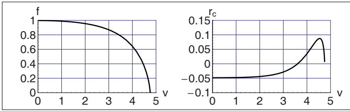
Fig. 2. The left panel gives the numeric finite-radius q -ball profile f(v) from the second-order ODE (6.3) with parameters and boundary conditions (6.7). Here, f refers to the dimensionless q -field and v to the dimensionless radial coordinate of the q -ball. The right panel gives the corresponding energy density (6.5).
