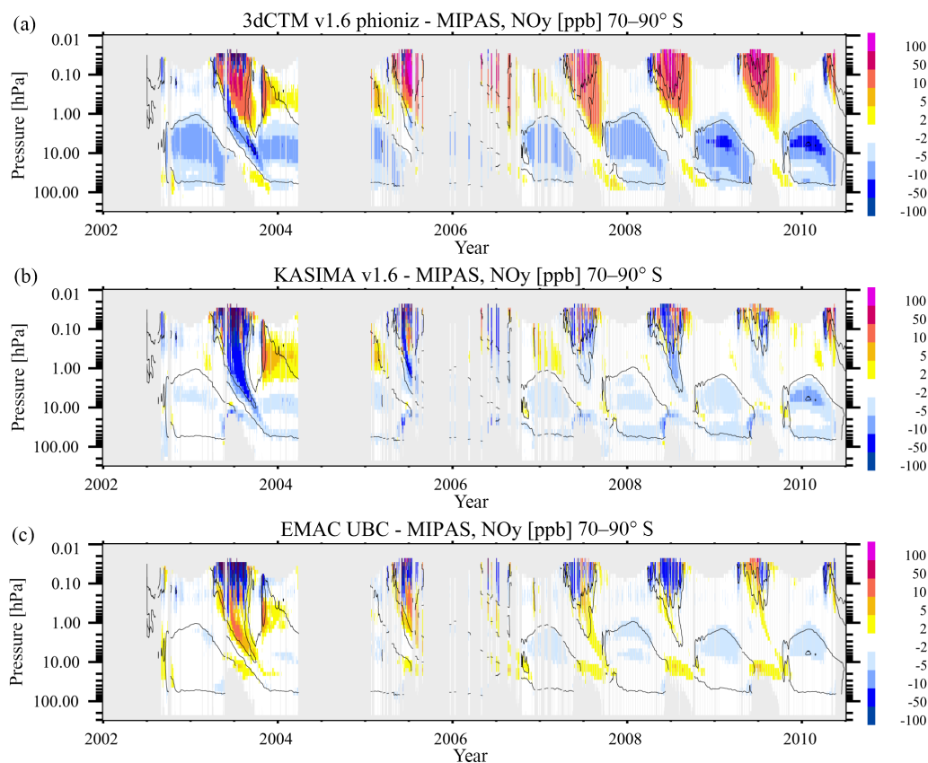
Figure 5. Absolute difference in \text{NO}_y (ppb) between models and MIPAS observations at high southern ( 70\text{--}90^\circ\text{ S} ) latitudes. Model data have been interpolated to the vertical grid of the MIPAS data, and days and altitudes are only shown where MIPAS data are available and fulfill the averaging kernel criterion. From top to bottom: 3dCTM v1.6 phioniz, KASIMA v1.6, and EMAC UBC. The black lines show the 10, 20, and 3000 ppb contours of the MIPAS data, smoothed with a 7-day running mean for clarity. The gray shaded areas are periods without MIPAS data; the period before the start of the KASIMA model run is also shown in the second panel.
