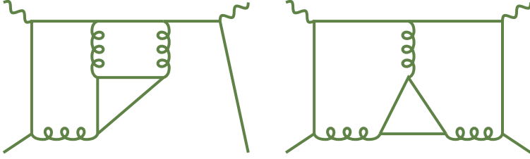
Fig. 1. The three-loop gauge-boson–quark forward scattering diagrams with MINCER topology BE that contribute to C_A C_F n_f part of the three-loop splitting functions for the quark \pm antiquark flavour differences in Eq. (2.3). The same diagrams, but with a one-loop insertion in one of the gluon lines, form the hardest part of the corresponding calculation of the four-loop C_A C_F n_f^2 contribution.
