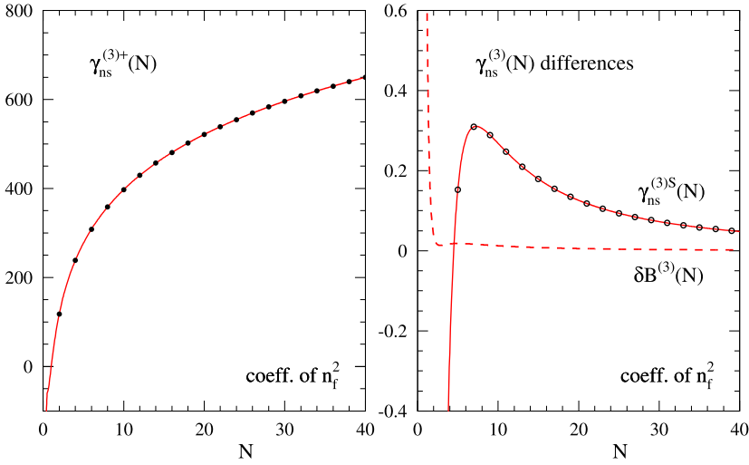
Fig. 2. The n_f^2 parts of the anomalous dimensions \gamma_{ns}^{(3)+}(N) (left) and \gamma_{ns}^{(3)s}(N) = \gamma_{ns}^{(3)v}(N) - \gamma_{ns}^{(3)-}(N) (right). Their even- N (left) and odd- N (odd) moments computed using FORCER [20,21] are shown together with the numerical all- N curves. Also shown on the right, where we focus on \gamma_{ns}^{(3)s} at N > 4 , is the difference \delta B^{(3)}(N) = \gamma_{ns}^{(3)-}(N) - \gamma_{ns}^{(3)+}(N) . Note the normalization of our expansion parameter a_s in Eq. (2.5).
