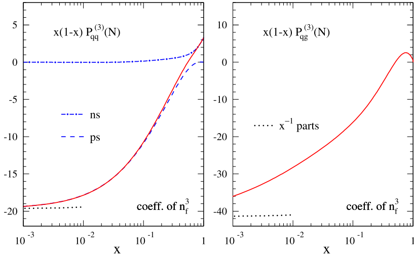
Fig. 7. The n_f^3 parts of the ‘upper row’ quark–quark and gluon–quark four-loop splitting functions in the \overline{\text{MS}} scheme, multiplied by x(1-x) for display purposes, together with their x^{-1} leading small- x terms at x < 10^{-2} . For the quark–quark case also the non-singlet and pure-singlet contributions are shown.
