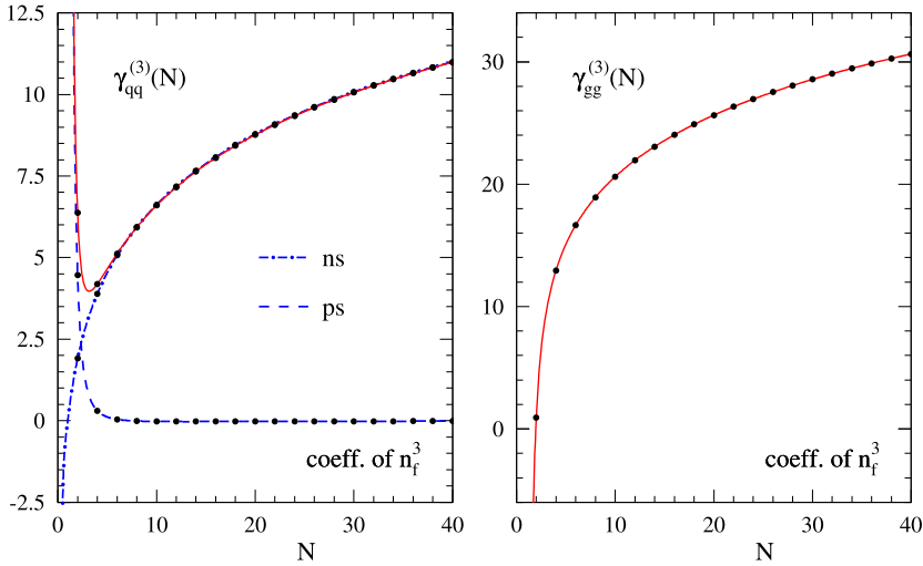
Fig. 3. The n_f^3 parts of the ‘diagonal’ quark–quark and gluon–gluon four-loop anomalous dimensions. The analytically calculated even- N moments are shown together with their continuation calculated via a numerical Mellin transformation of the corresponding x -space expressions using the program of Ref. [61]. For the quark–quark case the non-singlet and pure-singlet contributions are displayed separately.
