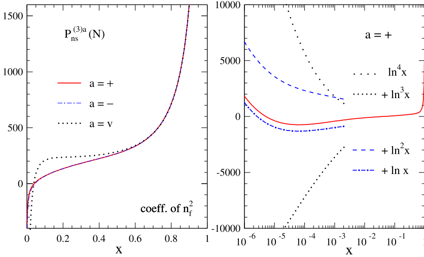
Fig. 5. Left: the n_f^2 parts of the four-loop splitting functions for the evolution of the combinations (2.3) of quark and anti-quark distributions given by Eqs. (4.5) – Eqs. (4.11). Right: the small- x behaviour of this contribution to P_{ns}^+ , compared to its successive approximations by the small- x logarithms in Eq. (4.14).
