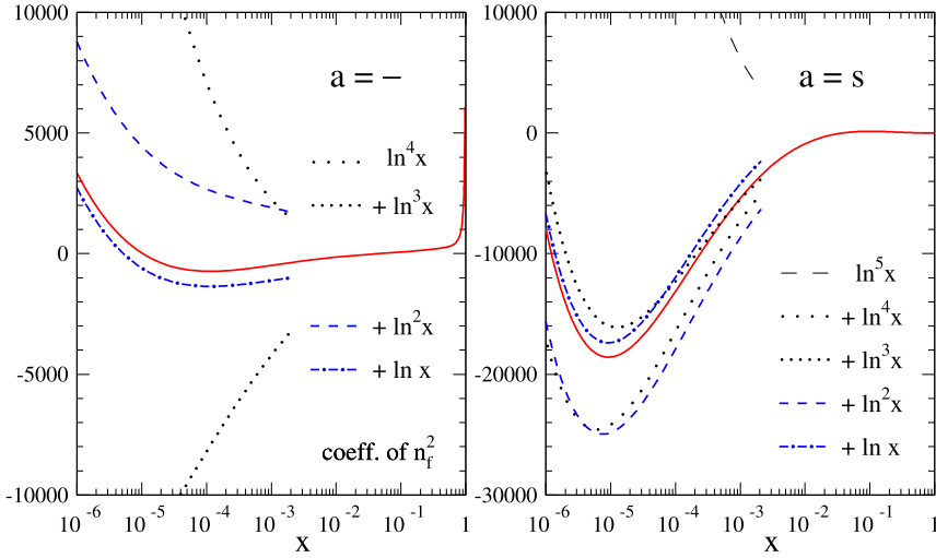
Fig. 6. As the right panel of Fig. 5, but for the splitting functions P_{ns}^- (left) and P_{ns}^s (right). Due to Eq. (2.5) all numbers have to be divided by (4\pi)^4 \simeq 25000 for an expansion in powers of \alpha_s .
