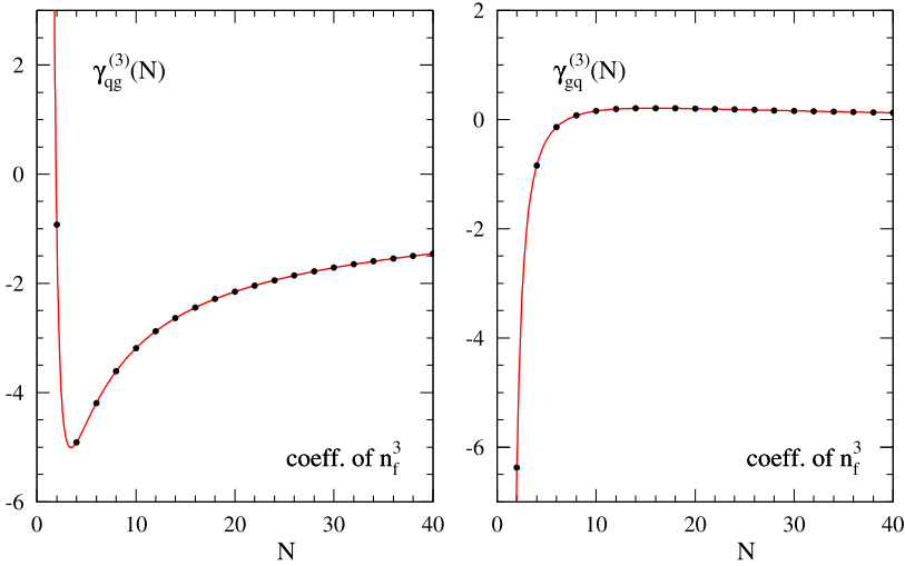
Fig. 4. As Fig. 3, but for the ‘off-diagonal’ gluon–quark and quark–gluon anomalous dimensions.
