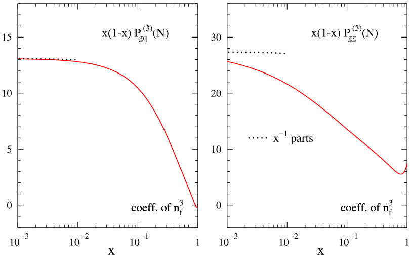
Fig. 8. As Fig. 7, but for the ‘lower row’ quark–gluon and gluon–gluon splitting functions at N^3\text{LO} .
