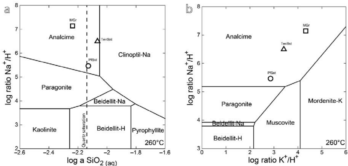
Fig. 3. Activity diagrams calculated with \text{GWB}^1 (GWB dataset thermos.tdat) with data points of the experimental fluid. Conditions were temperatures of 260 °C and corresponding water vapor pressure. Al was balanced with kaolinite. (a) \log a(\text{Na}^+)/a(\text{H}^+) vs. \log a(\text{SiO}_2(\text{aq})) ; (b) \log a(\text{K}^+)/a(\text{H}^+) vs. \log a(\text{Na}^+)/a(\text{H}^+) ; ( \text{SiO}_2(\text{aq}) = \text{Quartz saturated} ).
