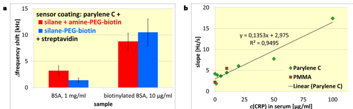
Fig. 1: Performance of SAW biosensors coated with silane-PEG-biotin. (a) Comparison of signal responses obtained by coating parylene C coated SAW devices with either silane plus amine-PEG-biotin or with silane-PEG-biotin. After immobilization of streptavidin, BSA and biotinylated BSA samples were applied subsequently. (b) Signal responses obtained with CRP samples and SAW devices coated subsequently with polymer (parylene C or PMMA), silane-PEG-biotin, streptavidin, and biotinylated anti-CRP.
