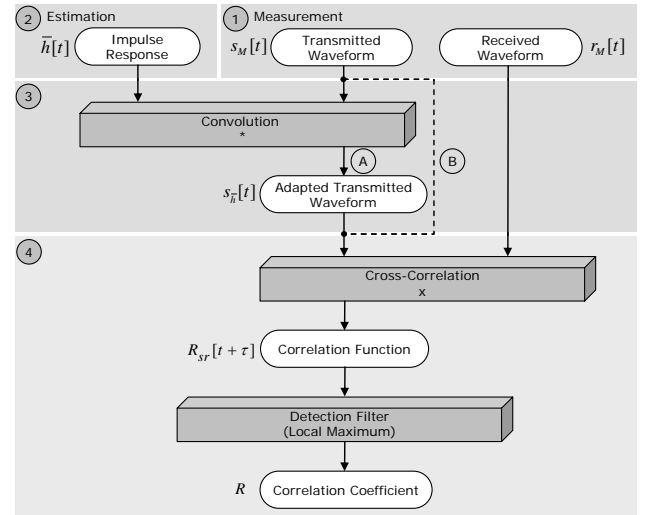
Figure 4. Processing chain.
