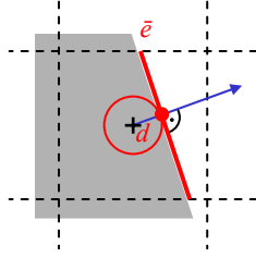
Figure 10. Edge \bar{e} with distance d
