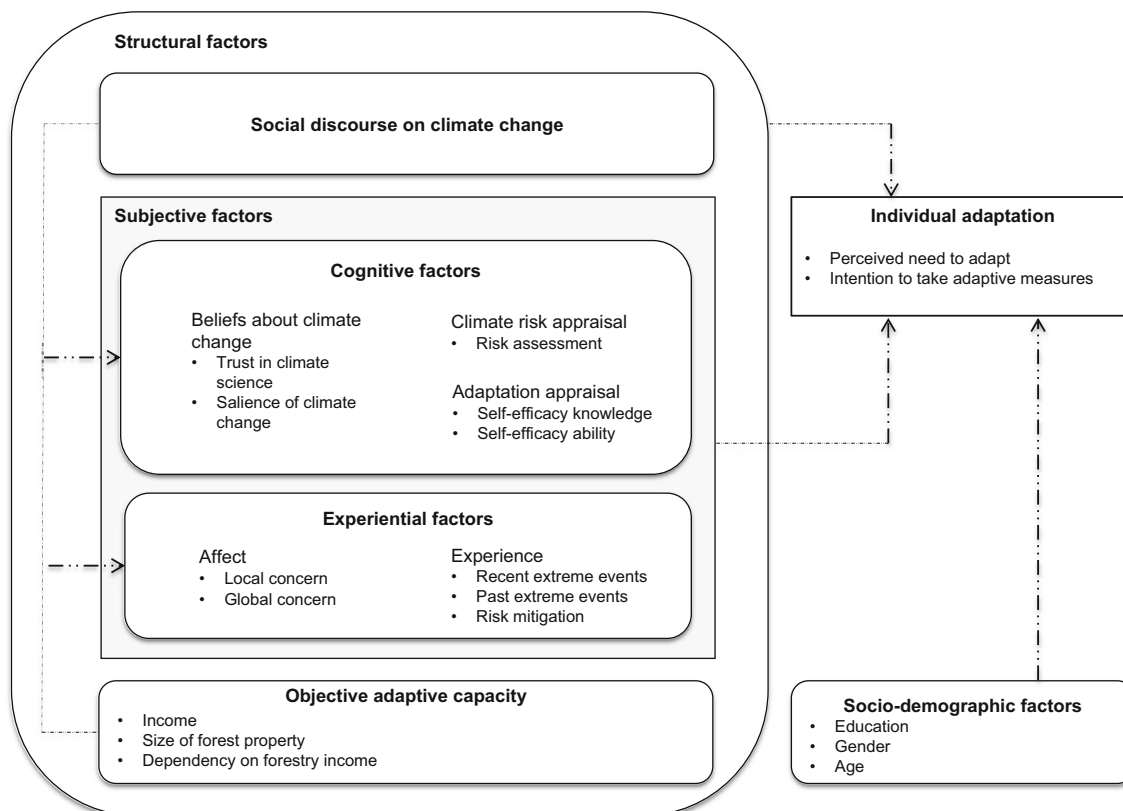
Fig. 1 Conceptual and analytical model of individual adaptation to climate change (based on Grothmann and Patt 2005 and van der Linden 2015)
