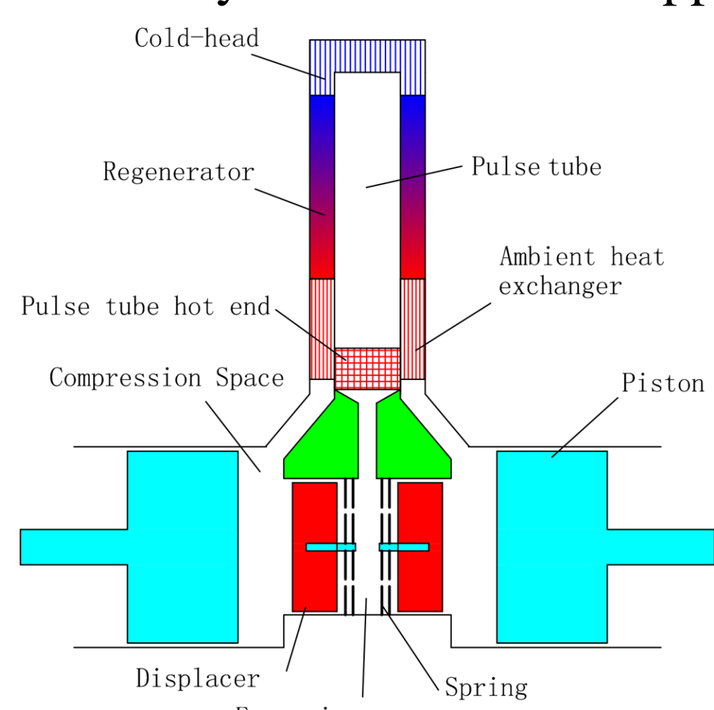
Fig.1 Illustration of pulse tube cryocooler using room temperature displacers
