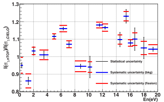
Figure 3. Ratio between the ^{235}\text{U}(n,\gamma) cross section measured at the CERN n_TOF facility and the latest CIELO release in the ^{235}\text{U} resonances from 0.2 eV to 20 eV.
