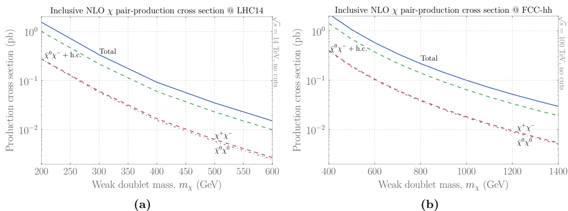
Figure 1. Corrected pair-production cross sections for a weak doublet with hypercharge \frac{1}{2} at NLO, obtained using PROSPINO in the pure-Higgsino limit, for LHC14 (a) and FCC-hh (b).
