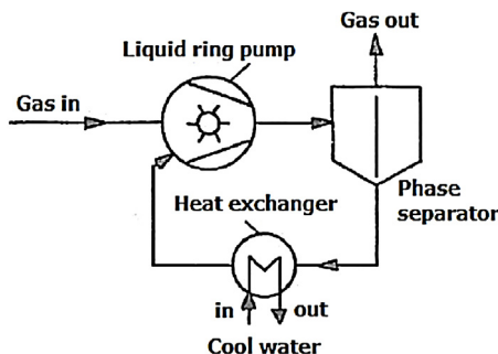
Fig. 2. Flowchart of a liquid ring pump station [5].
