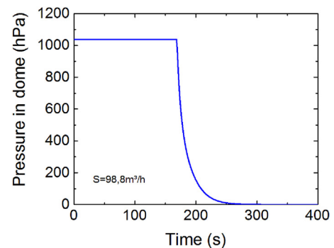
Fig. 4. First pump-down curve.
