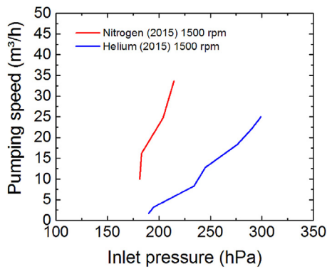
Fig. 5. Pumping speed curves for nitrogen and helium.
