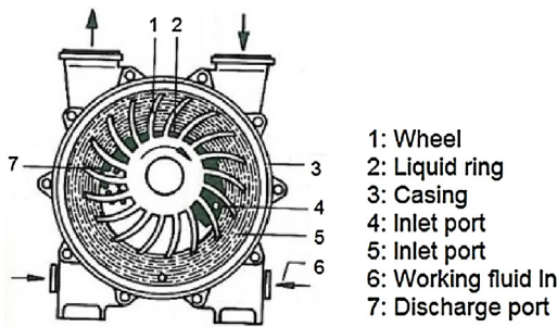
Fig. 1. Working principle of a liquid ring pump [5].
