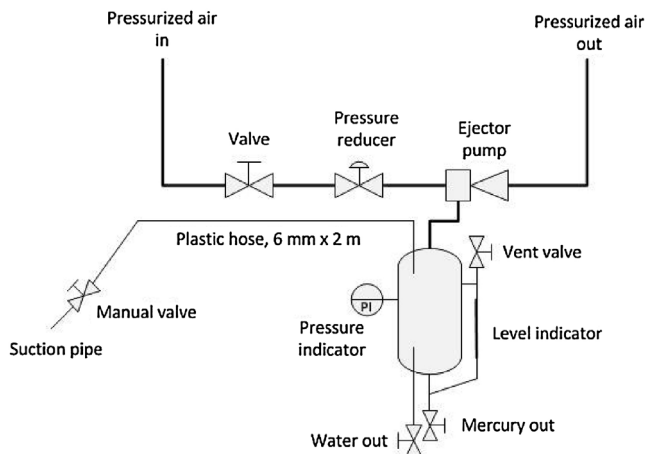
Fig. 7. Flowchart of the handling tool for mercury transfer.
