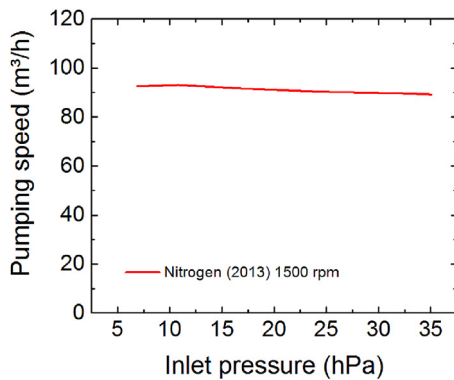
Fig. 6. Pumping speed curves for the first pump-down.
