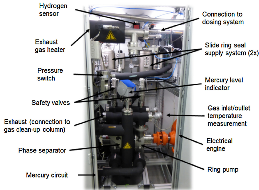
Fig. 3. Pump installed in the enclosure.
