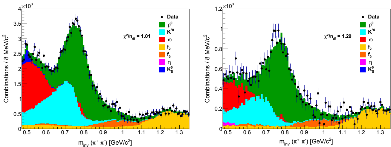
Fig. 6 Invariant mass distribution of oppositely charged particles, calculated assuming pion masses, in \pi^- + C production interactions in the range 0.3 < x_F < 0.4 at 158 GeV/c (left) and at 350 GeV/c (right).
