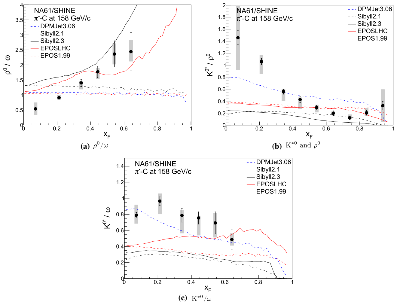
Fig. 21 Ratio of meson spectra in \pi^- + C production interactions at 158 GeV/c. The dots with error bars show the data and its statistical uncertainties. The shaded boxes denote the systematic uncertainties.
