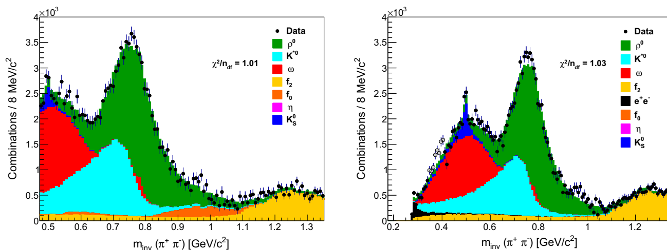
Fig. 8 An example of the template fit to 158 GeV/c data in the range 0.3 < x_F < 0.4 using the nominal fit range (left) and the extended fit range (right) including a template for e^+e^- pair production
