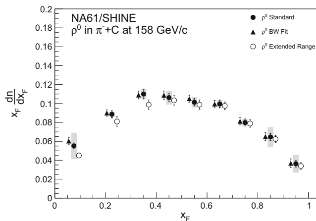
Fig. 10 Comparison of \rho^0 x_F spectra at 158 GeV/c (left) and 350 GeV/c (right) from the standard template analysis method, the extended fit range and when using a Breit–Wigner function to param-
