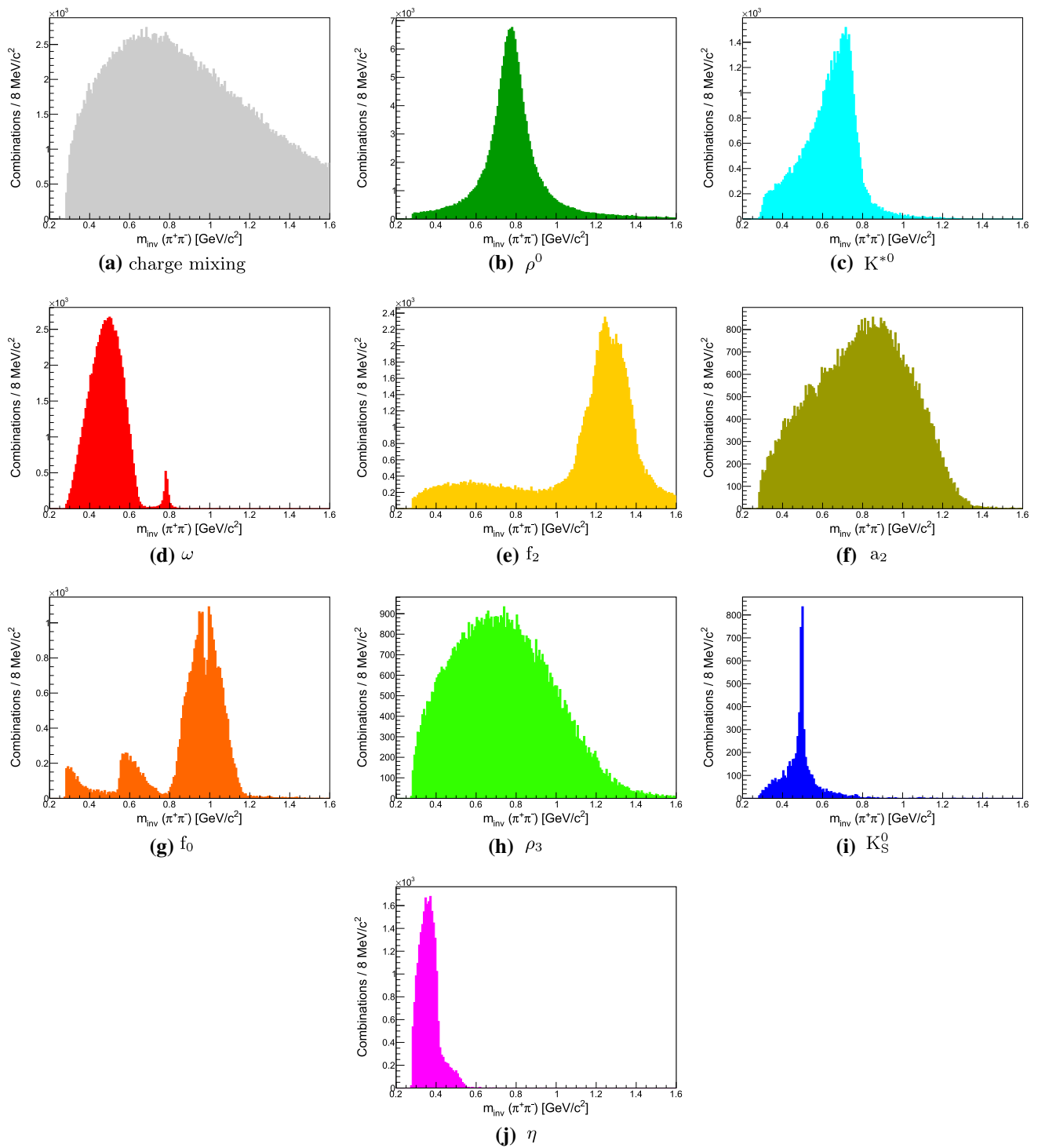
Fig. 15 Templates of the invariant mass spectra of resonances and background at 158 GeV/c in the range 0.4 < x_F < 0.5 assuming pion masses
