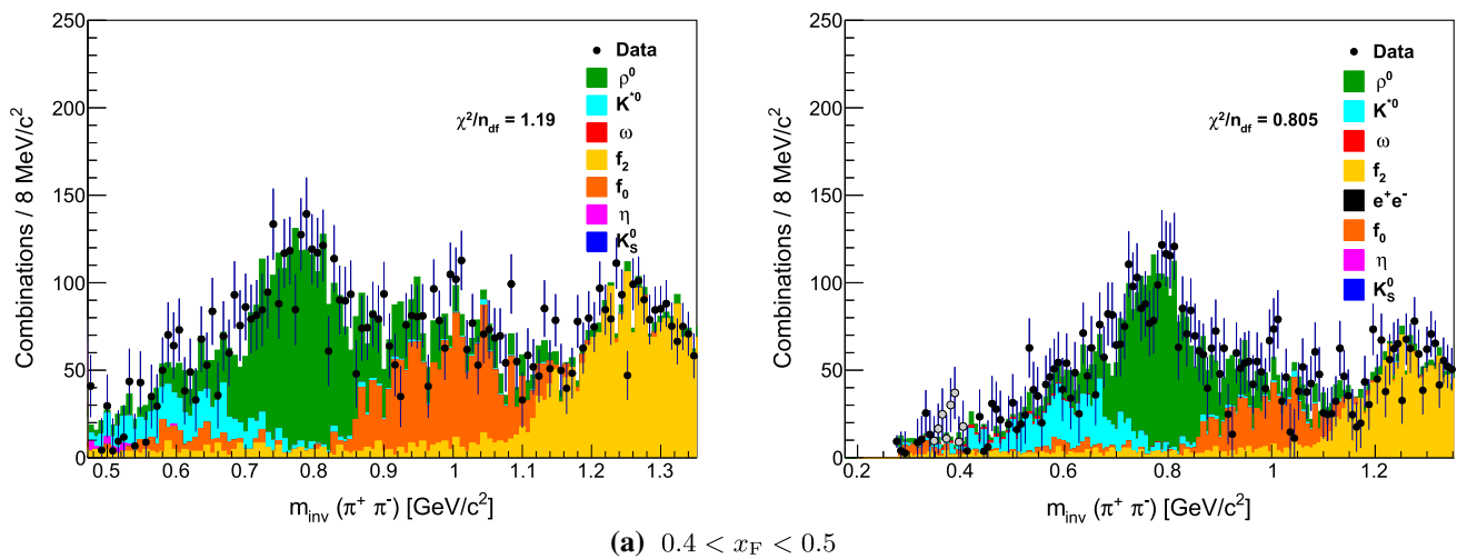
Fig. 20 Invariant mass distribution of opposite charged particles, calculated assuming pion masses, in \pi^- + C interactions at 350 GeV/c. Dots with error bars denote the data and the fitted resonance templates are shown as filled histograms. The fitted background and high mass
