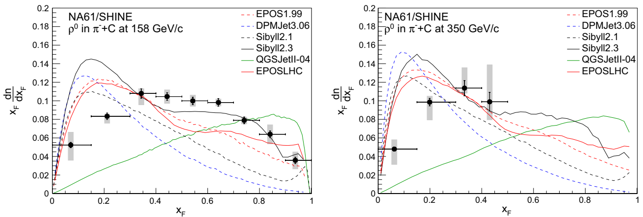
Fig. 12 Scaled x_F -spectra of \rho^0 mesons, x_F dn/dx_F , in \pi^- + C production interactions at 158 (left) and 350 GeV/c (right). The error bars show the statistical, the bands indicate systematic uncertainties. The
