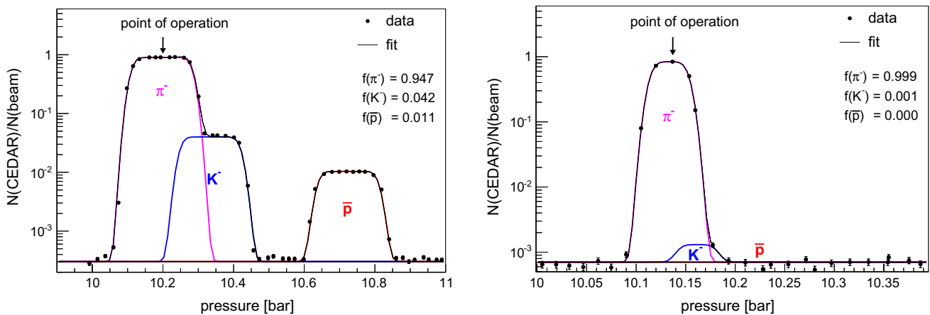
Fig. 2 The fraction of CEDAR triggers as a function of its gas pressure for beam momenta of 158 (left) and 350 (right) GeV/c. The fitted fractions f of pions, kaons and anti-protons are quoted within the figures and the point of operation during data taking is indicated by an arrow
