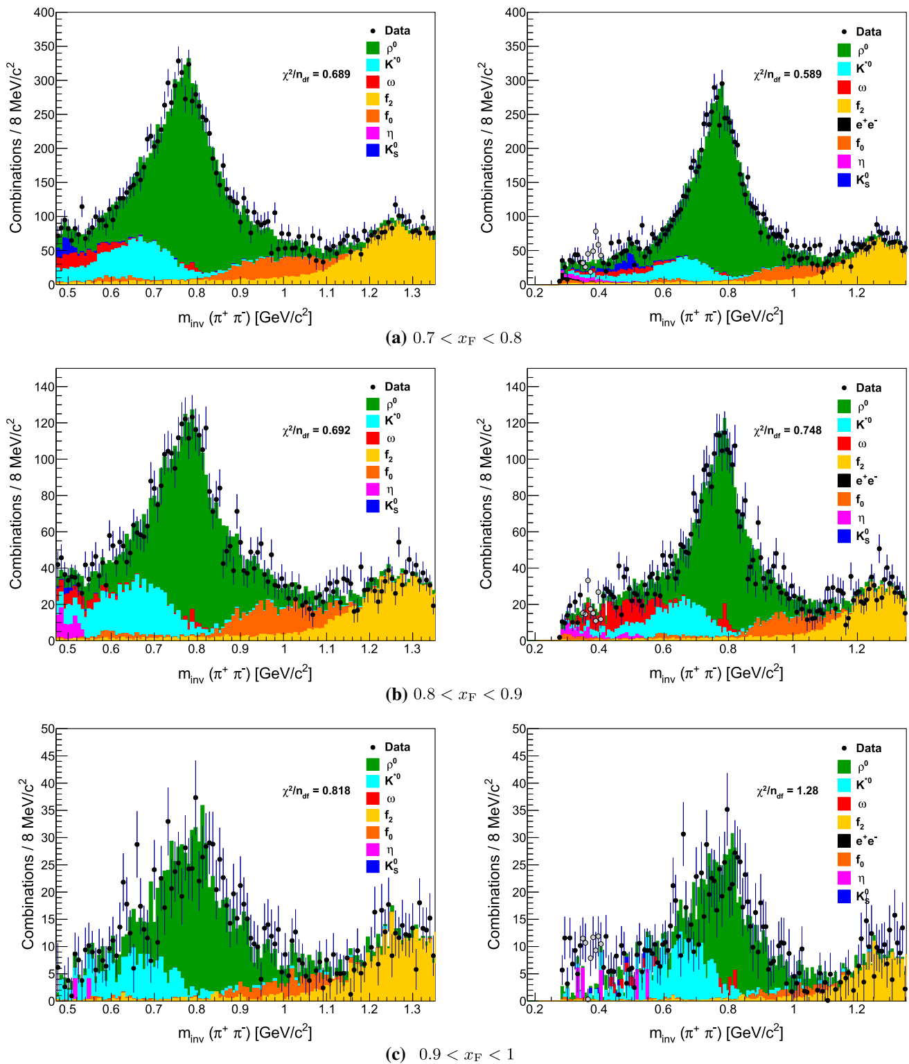
Fig. 18 Invariant mass distribution of opposite charged particles, calculated assuming pion masses, in \pi^- + C interactions at 158 GeV/c. Dots with error bars denote the data and the fitted resonance templates are shown as filled histograms. The fitted background and high mass resonances have been subtracted. Two fits with different m_{\text{inv}}(\pi^+\pi^-)
