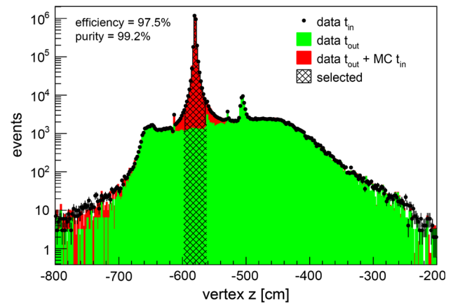
Fig. 4 Distribution of fitted vertex z positions for \pi^- + C interactions at 158 GeV/c. The filled green area shows the distribution for events recorded with the target removed, while the filled red area shows the distribution for the reconstructed Monte Carlo simulation. The dashed area indicates events selected for this analysis
