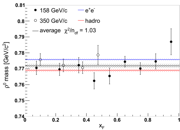
Fig. 9 Fitted \rho^0 mass for \pi^- + C production interactions as a function of x_F . The blue line indicates the average mass from e^+e^- annihilation and the red line indicates the average mass from other reactions, which is dominated by hadroproduction measurements [51]. The black line is the weighted mean of all measurements, combining both 158 and 350 GeV/c data
