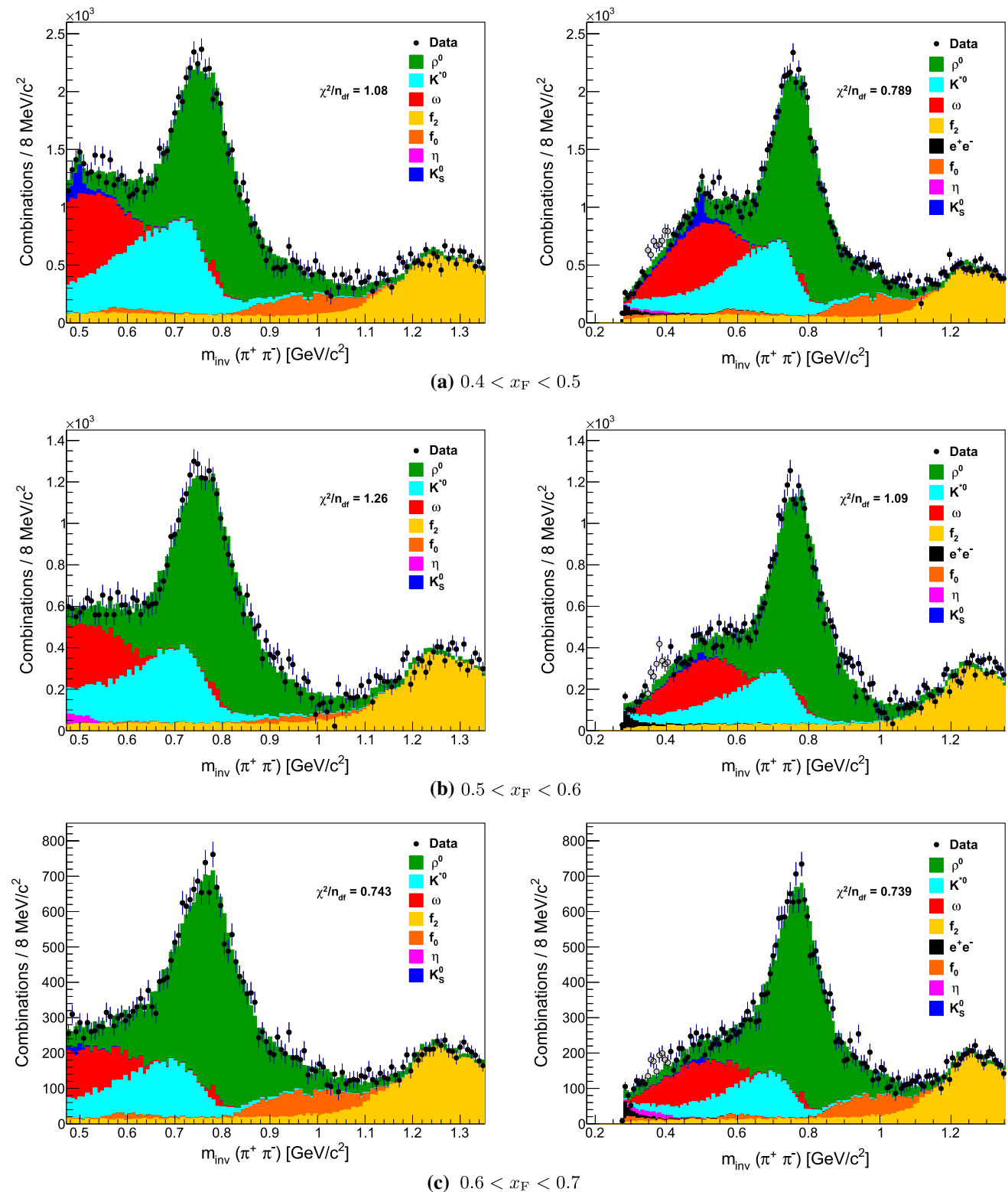
Fig. 17 Invariant mass distribution of opposite charged particles, calculated assuming pion masses, in \pi^- + C interactions at 158 GeV/c. Dots with error bars denote the data and the fitted resonance templates are shown as filled histograms. The fitted background and high mass resonances have been subtracted. Two fits with different m_{\text{inv}}(\pi^+\pi^-)
