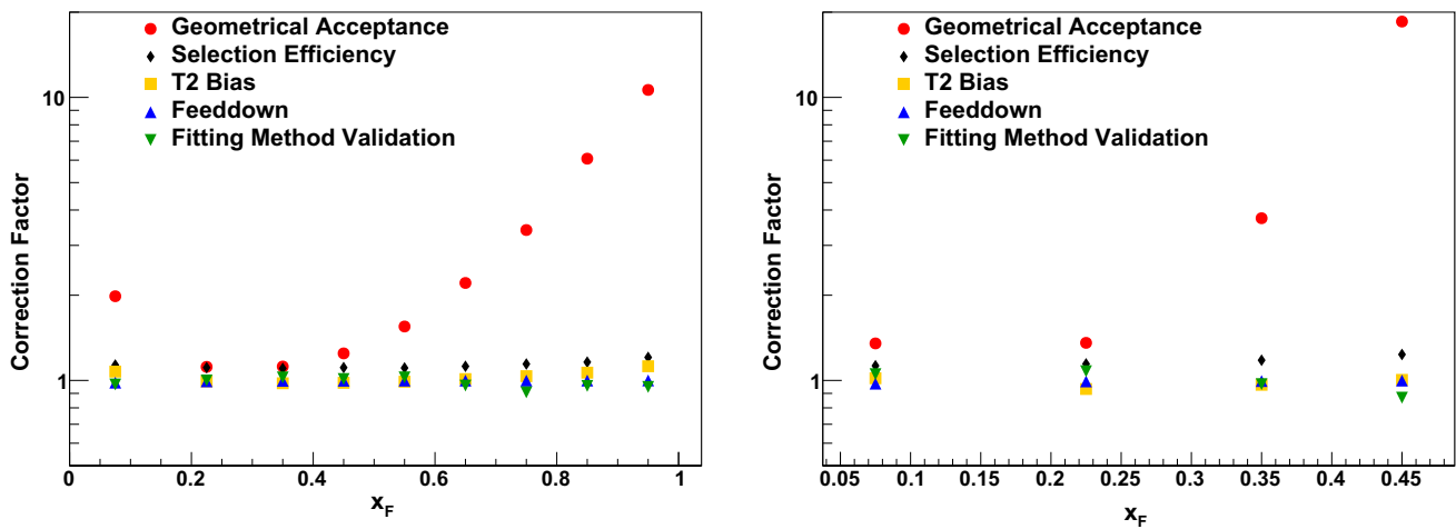
Fig. 7 Correction factors for the \rho^0 spectra in \pi^- + C production interactions at 158 GeV/c (left) and 350 GeV/c (right). It can easily be seen that the correction for geometrical acceptance dominates in almost every bin
