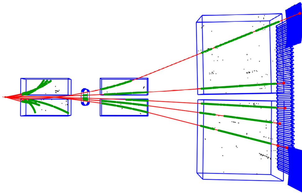
Fig. 3 An example of a \pi^- + C interaction at 158 GeV/c measured in the NA61/SHINE detector (top view). The measured points (green dots) are used to fit tracks (red lines) to the interaction point. The black dots show the noise clusters and the red dots show matched Time of Flight hits (not used in this analysis)
