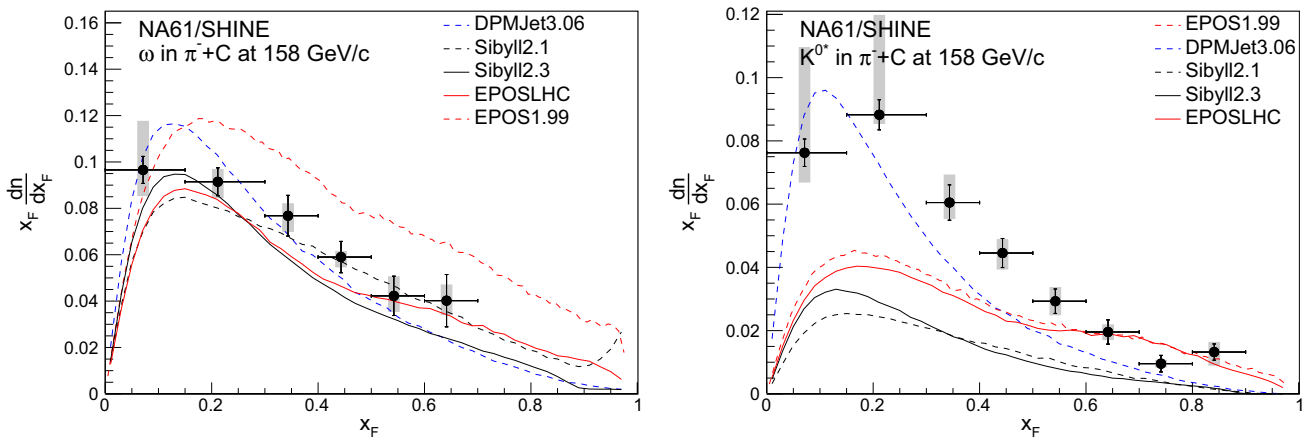
Fig. 13 Scaled x_F -spectra of \omega (left) and K^{*0} (right) mesons, x_F dn/dx_F , in \pi^- + C production interactions at 158 GeV/c. The error bars show the statistical, the bands indicate systematic uncertainties.
