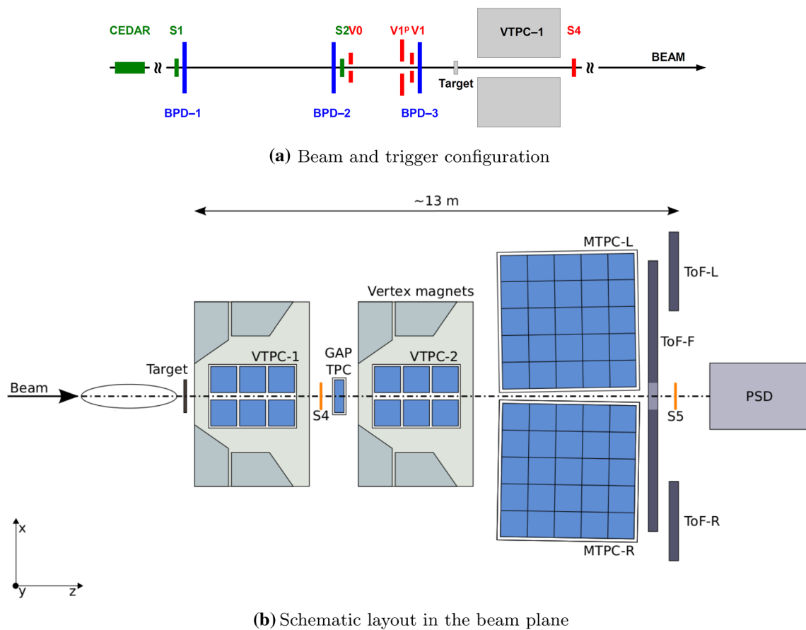
Fig. 1 Experimental setup of the NA61/SHINE experiment [30] (configuration for the \pi^- + C data taking). The coordinate system used in this paper is indicated on the lower left. The incoming beam direction is along the z axis. The magnetic field bends charged particle trajectories in the x-z (horizontal) plane. The drift direction in the TPCs is along
