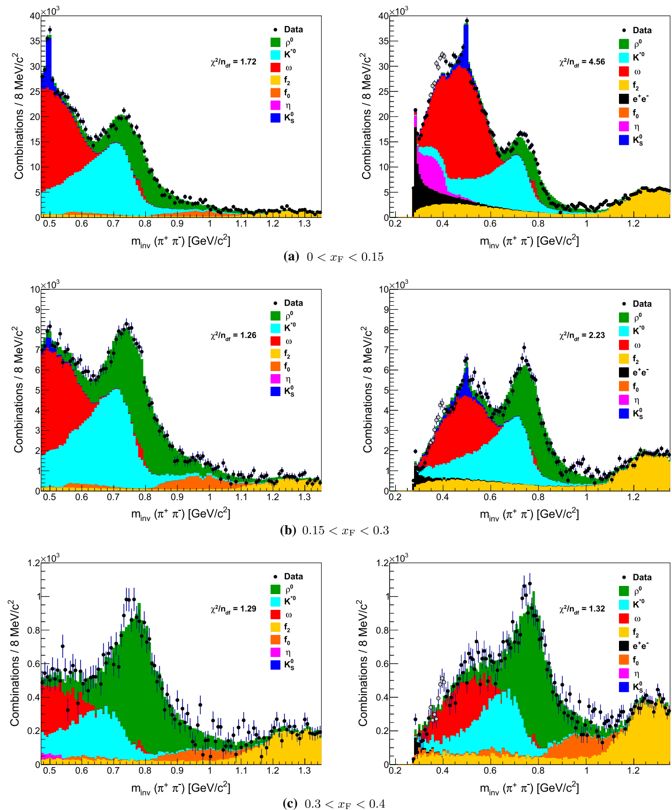
Fig. 19 Invariant mass distribution of opposite charged particles, calculated assuming pion masses, in \pi^- + C interactions at 350 GeV/c. Dots with error bars denote the data and the fitted resonance templates are shown as filled histograms. The fitted background and high mass resonances have been subtracted. Two fits with different m_{\text{inv}}(\pi^+\pi^-)
