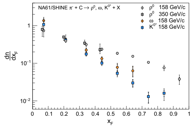
Fig. 11 Average multiplicity of meson resonances in \pi^- + C collisions. The results for \rho^0 mesons are shown for p_{\text{beam}} = 158 and 350 GeV/c and the spectra of \omega and K^{*0} mesons were measured at p_{\text{beam}} = 158 GeV/c. The inner error bars show the statistical uncertainty and the outer error bar denotes the total uncertainty obtained by adding statistical and systematic uncertainties in quadrature
