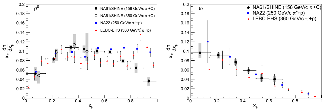
Fig. 14 Scaled x_F -spectra of meson production in \pi^- + C production interactions at 158 and 350 GeV/c (350 GeV/c shifted by 0.035). The error bars show the statistical, the bands indicate systematic uncer-
