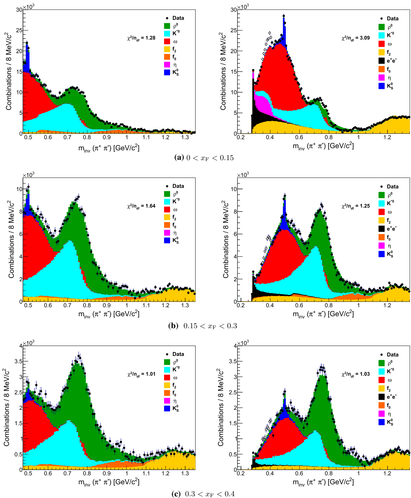
Fig. 16 Invariant mass distribution of opposite charged particles, calculated assuming pion masses, in \pi^- + C interactions at 158 GeV/c. Dots with error bars denote the data and the fitted resonance templates are shown as filled histograms. The fitted background and high mass resonances have been subtracted. Two fits with different m_{inv}(\pi^+\pi^-)
