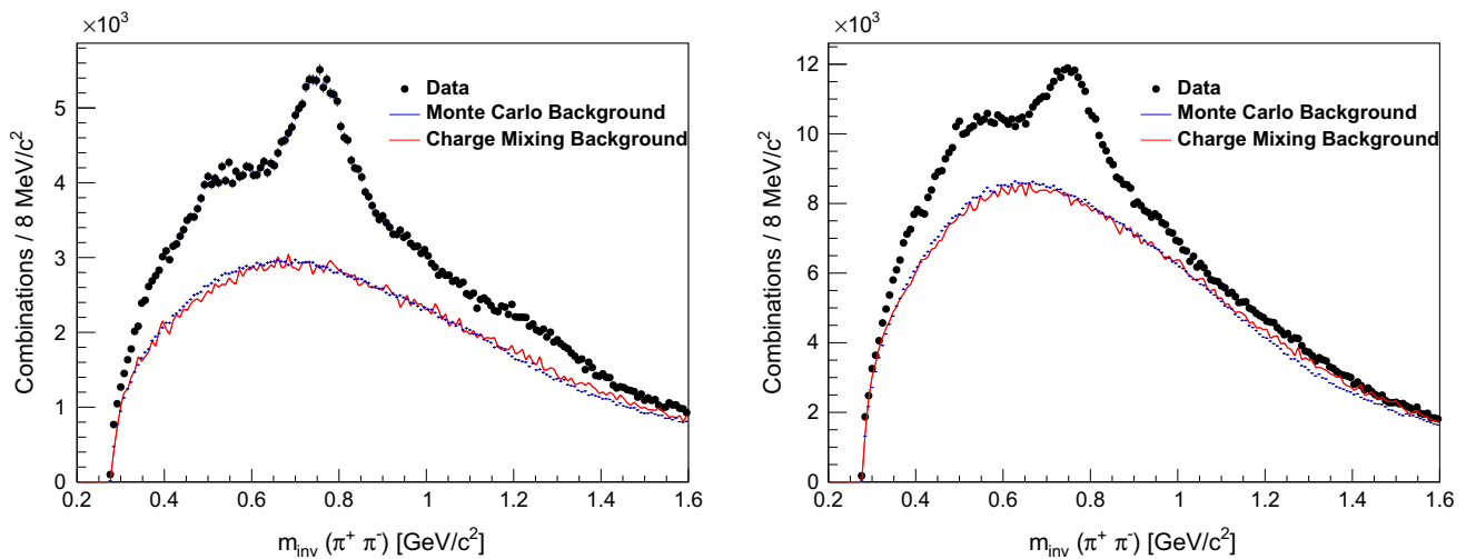
Fig. 5 Invariant mass distribution of opposite charge particles, calculated assuming pion masses, in \pi^- + C production interactions at 158 GeV/c in the range 0.4 < x_F < 0.5 (left) and 0.3 < x_F < 0.4
